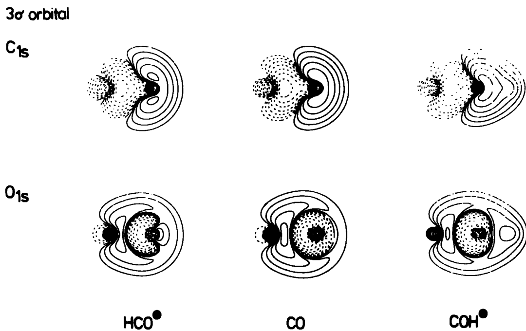
Fig. (7.7) Density difference contour plots for HCO + , CO and COH + .
