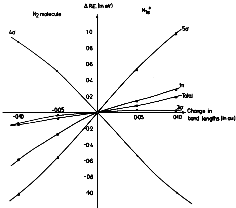
Fig. (6.14) Variation of single orbital relaxation energies as a function of bond-length.
