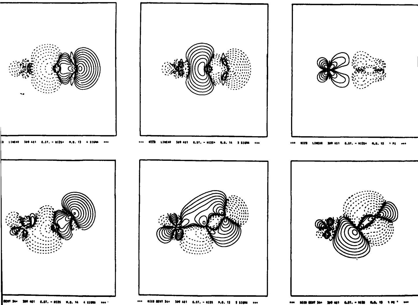
Fig. (8.10) Density difference contours for Ni_{12s} core-ionization.
