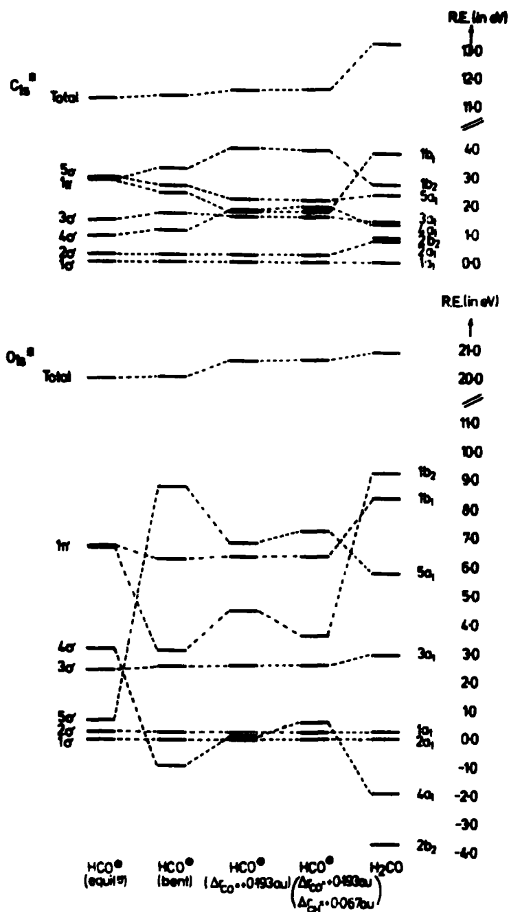
Fig.(7.5) Total R.E. and individual orbital contributions to the total R.E. in the series HCO^+ (linear), HCO^+ (bent) and H_2CO subsequent upon C_{1s} and O_{1s} core-ionization.
