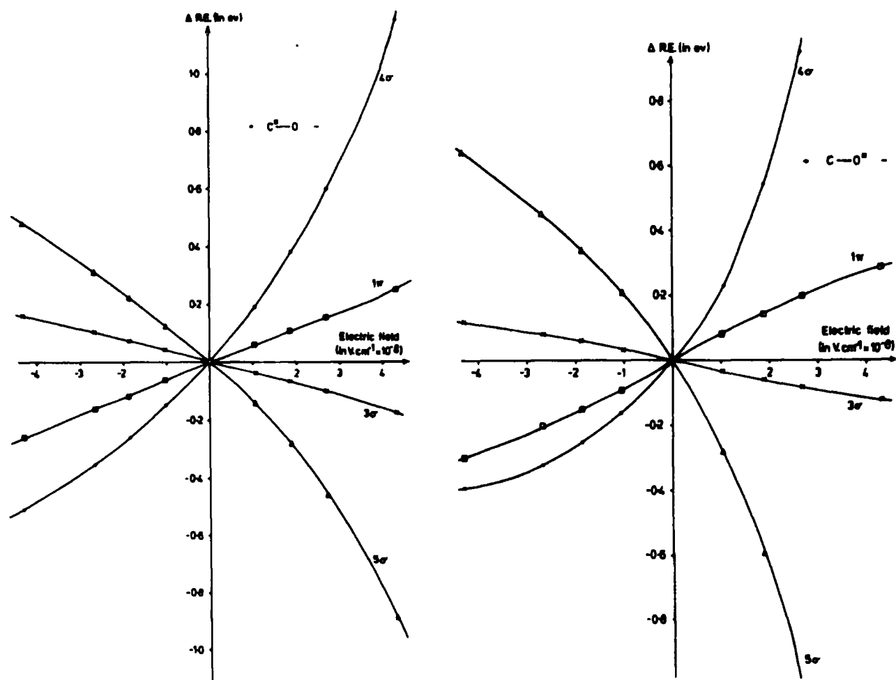
Fig.(6.16) Variation of single orbital relaxation energies in CO as a function of electric field.
