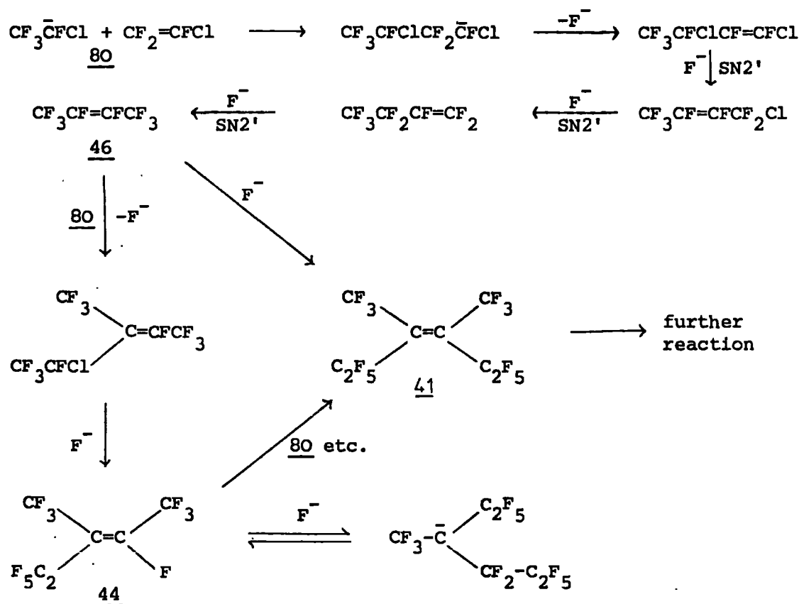
Scheme 27
