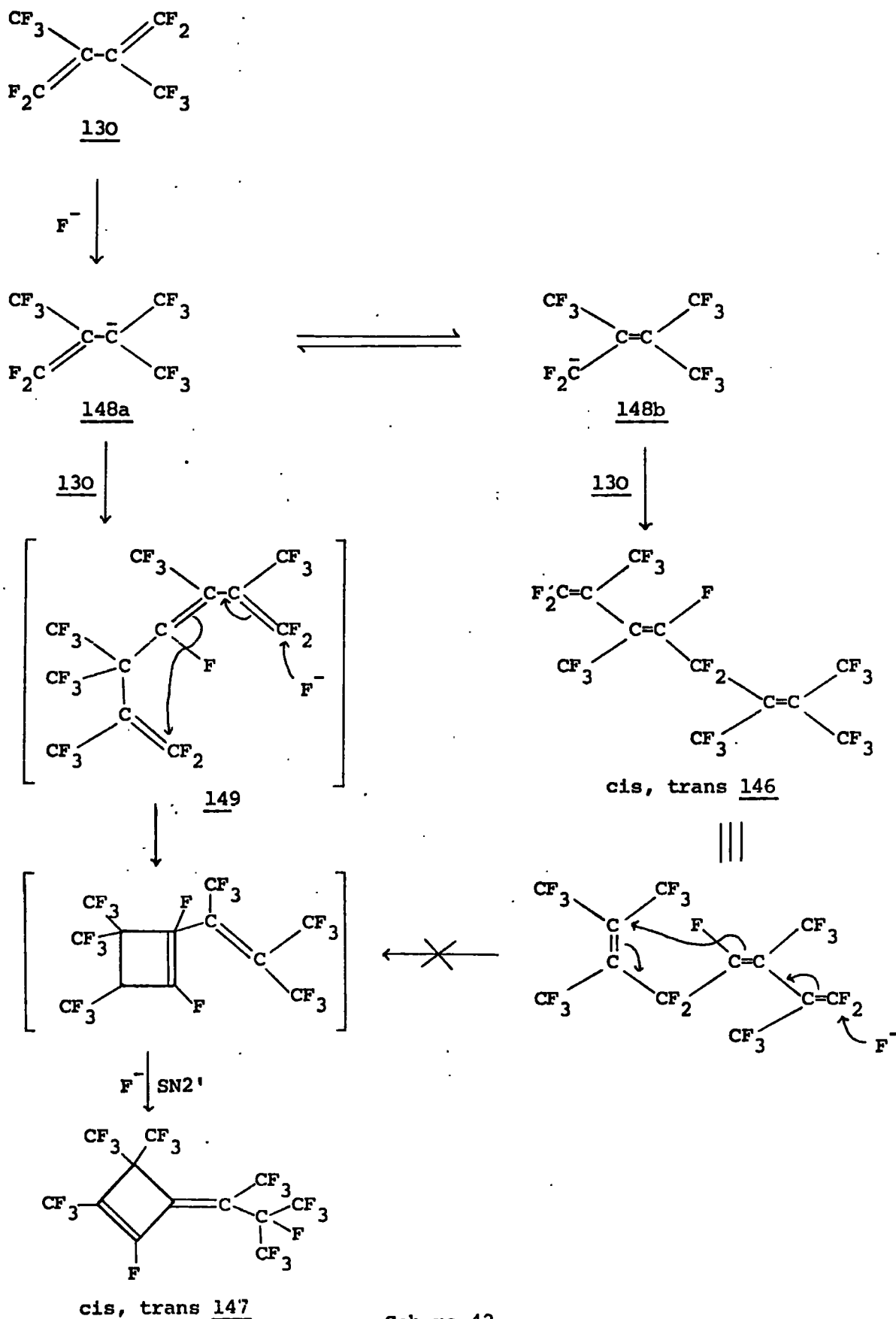
Scheme 42
