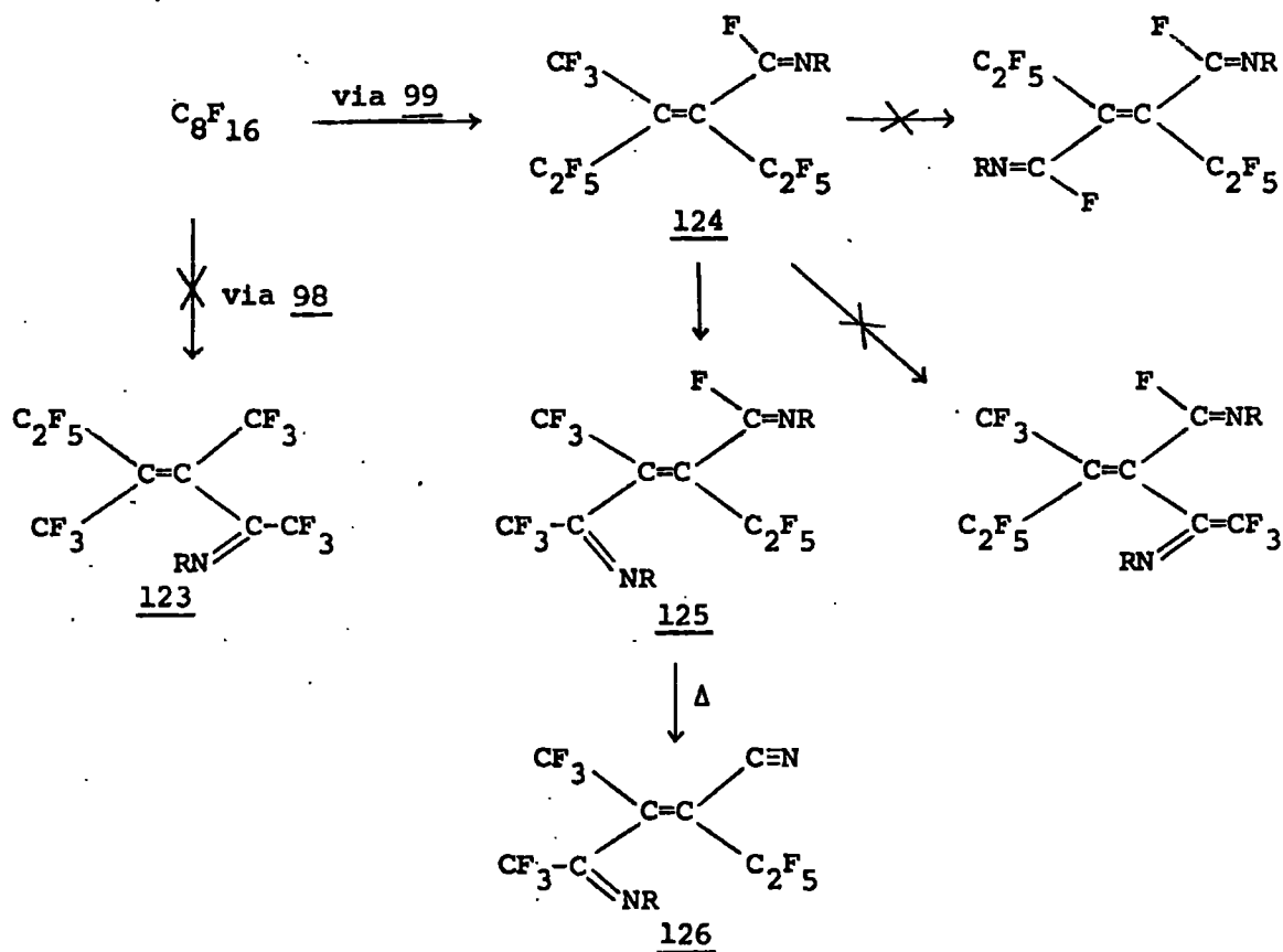
Scheme 39
