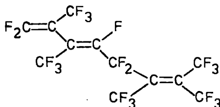
cis, trans 146
