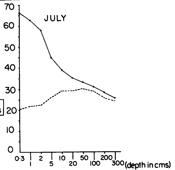
Fig.3-10 EXTREME SOIL TEMPERATURE IN DRY AND WET FIELDS AT GIZA
