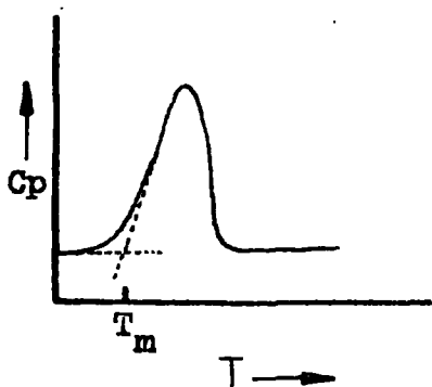
Fig. 5.2 DSC trace of a melting point transition.
