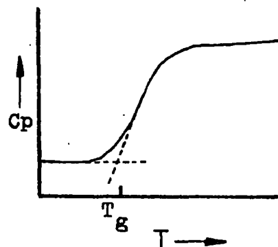
Fig. 5.3 DSC trace of a glass transition.
