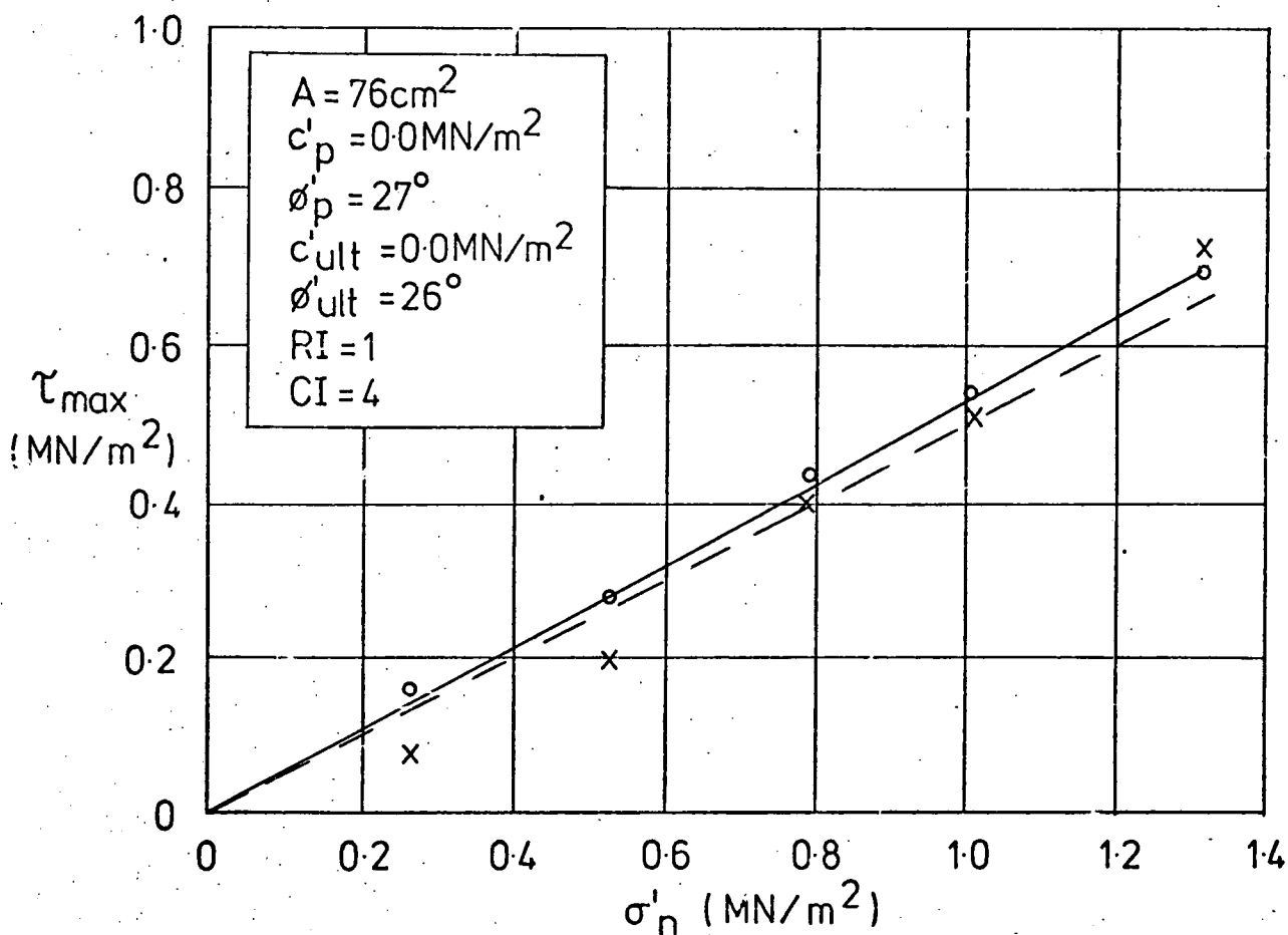
Fig. K.4 DRY SAMPLE, BOREHOLE 100, DEPTH 29.8m
