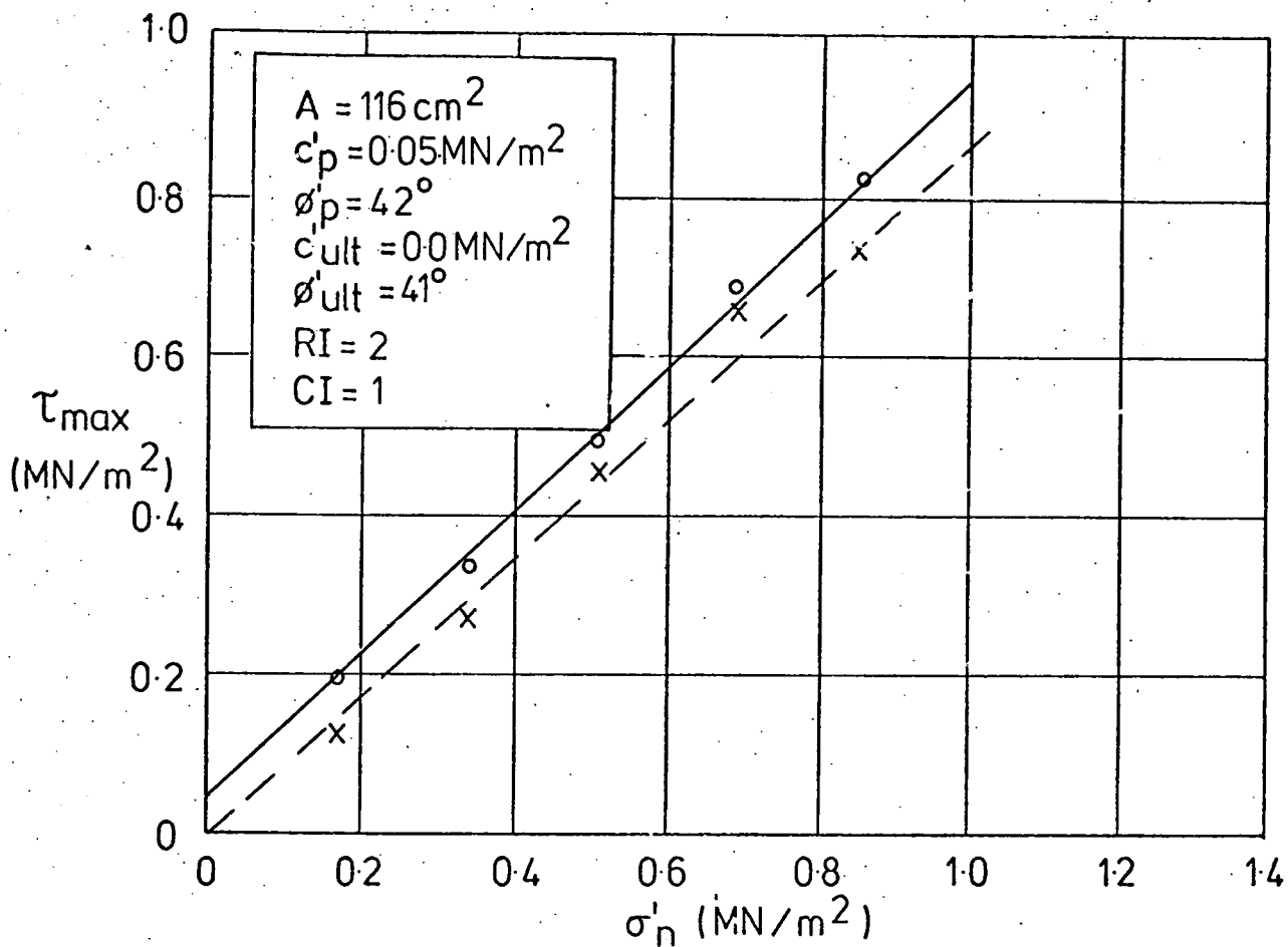
Fig.K.3 DRY SAMPLE, BOREHOLE 100, DEPTH 17.6m.
