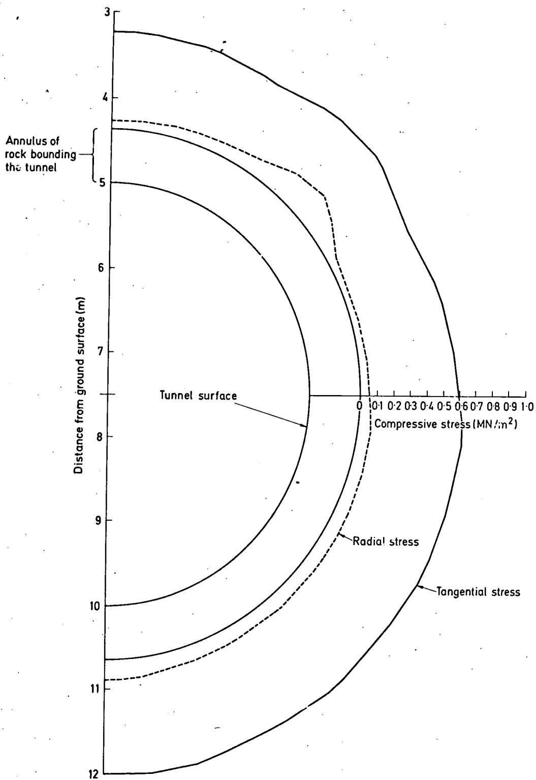
Fig. 8.10 VARIATION IN THEORETICAL RADIAL AND TANGENTIAL STRESS MAGNITUDES ROUND THE ANNULUS OF ROCK 0.3m FROM THE TUNNEL SURFACE, K_0=1.0 , SHALLOW
