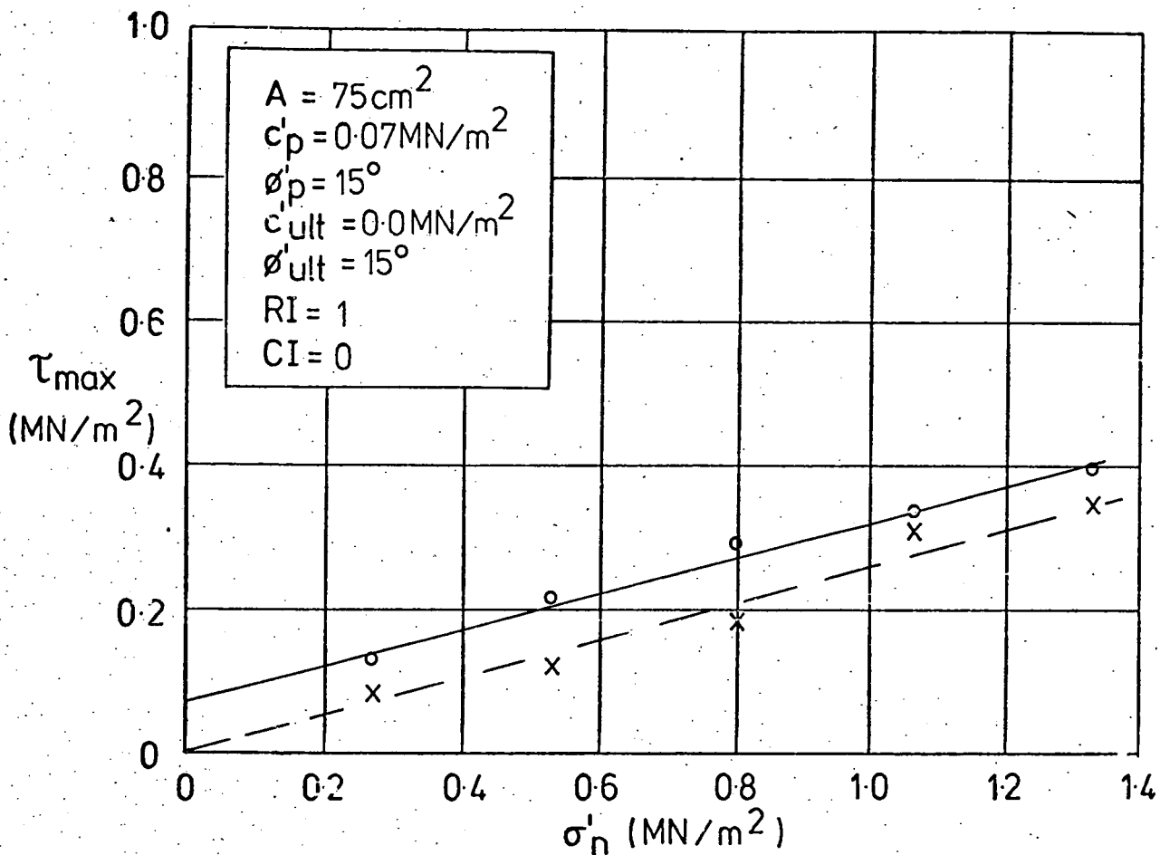
Fig.K.21 WET SAMPLE , BORHOLE 104 , DEPTH 182m.
