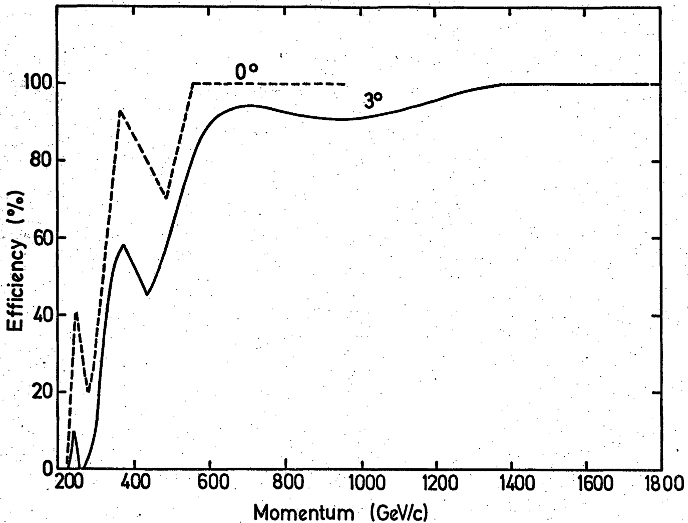
Figure 4.12. Efficiency of Mark I momentum selector for incident angles of 0^\circ and 3^\circ for negative particles in positive field.
