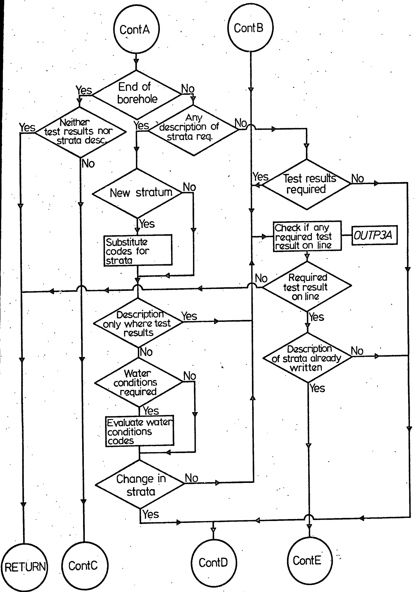
Fig. C.9b Part b of the structure of Outp3
