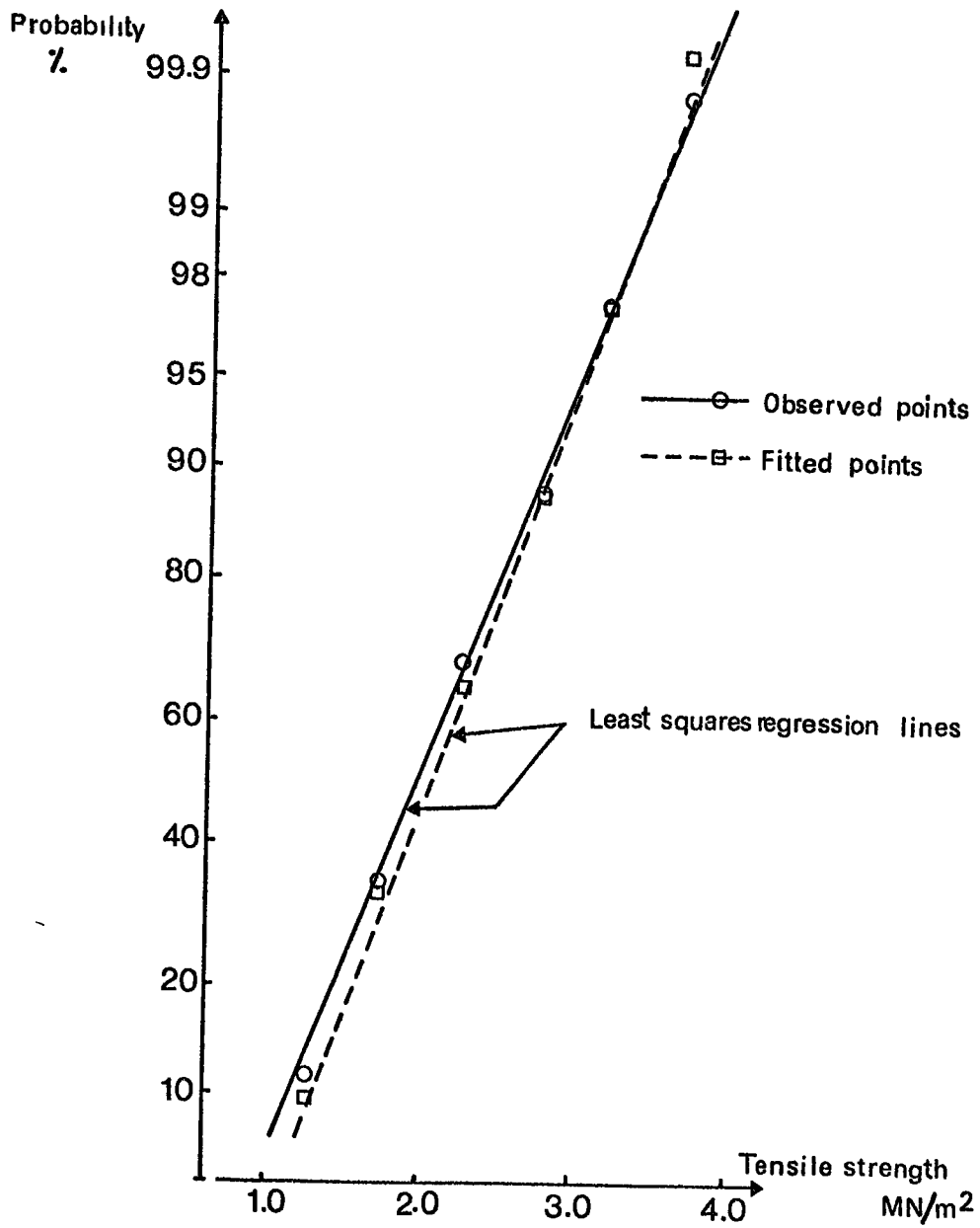
Fig. 4.4. Normal Distribution for 26 Determinations of the Tensile Strength of Coarse Carboniferous Sandstone by Brazilian Test.
