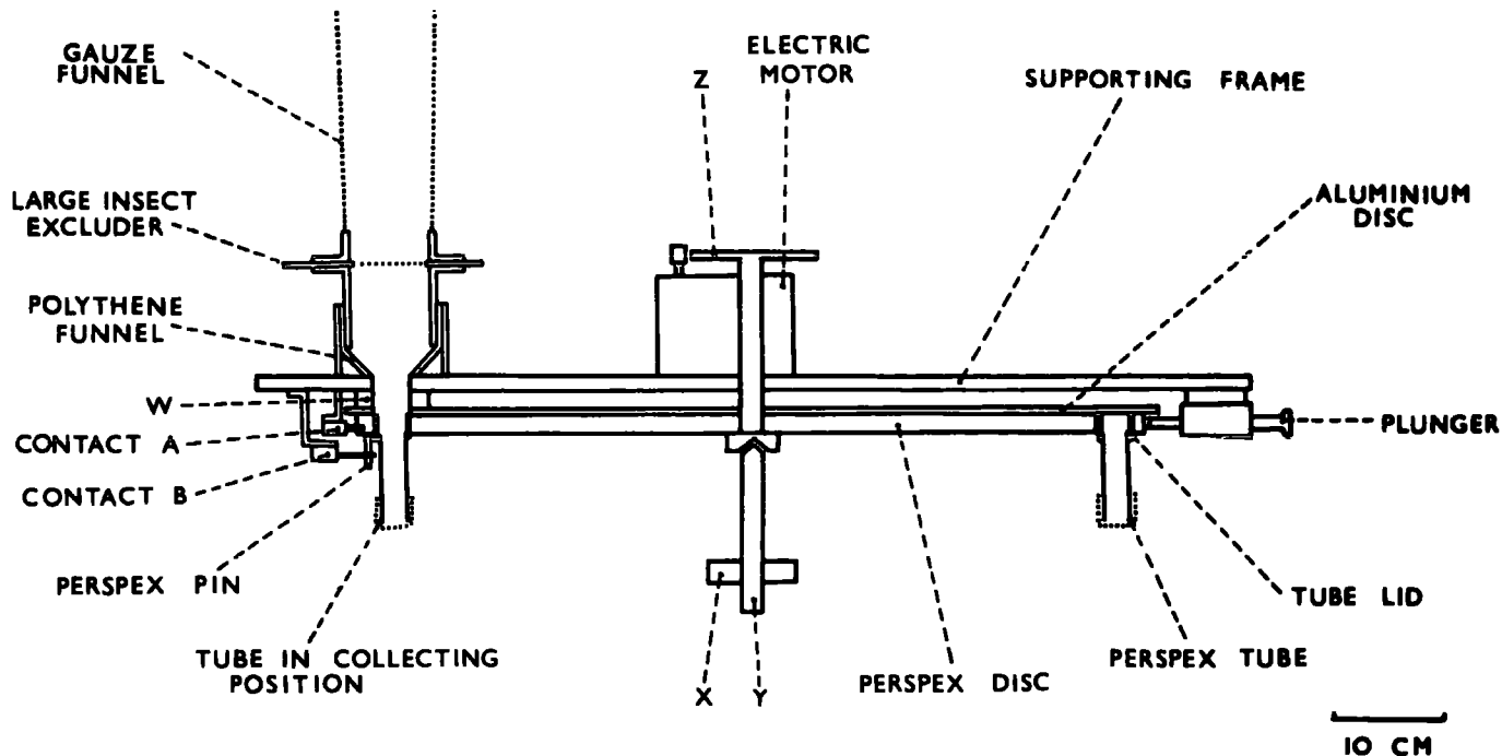
FIG. 2 Section along A-B (Fig.1) of the apparatus. [ W = perspex washer; X = cross bar; Y = pivoting spindle of the perspex disc, geared to the motor; Z = driving spindle of the perspex disc, geared to the motor].
