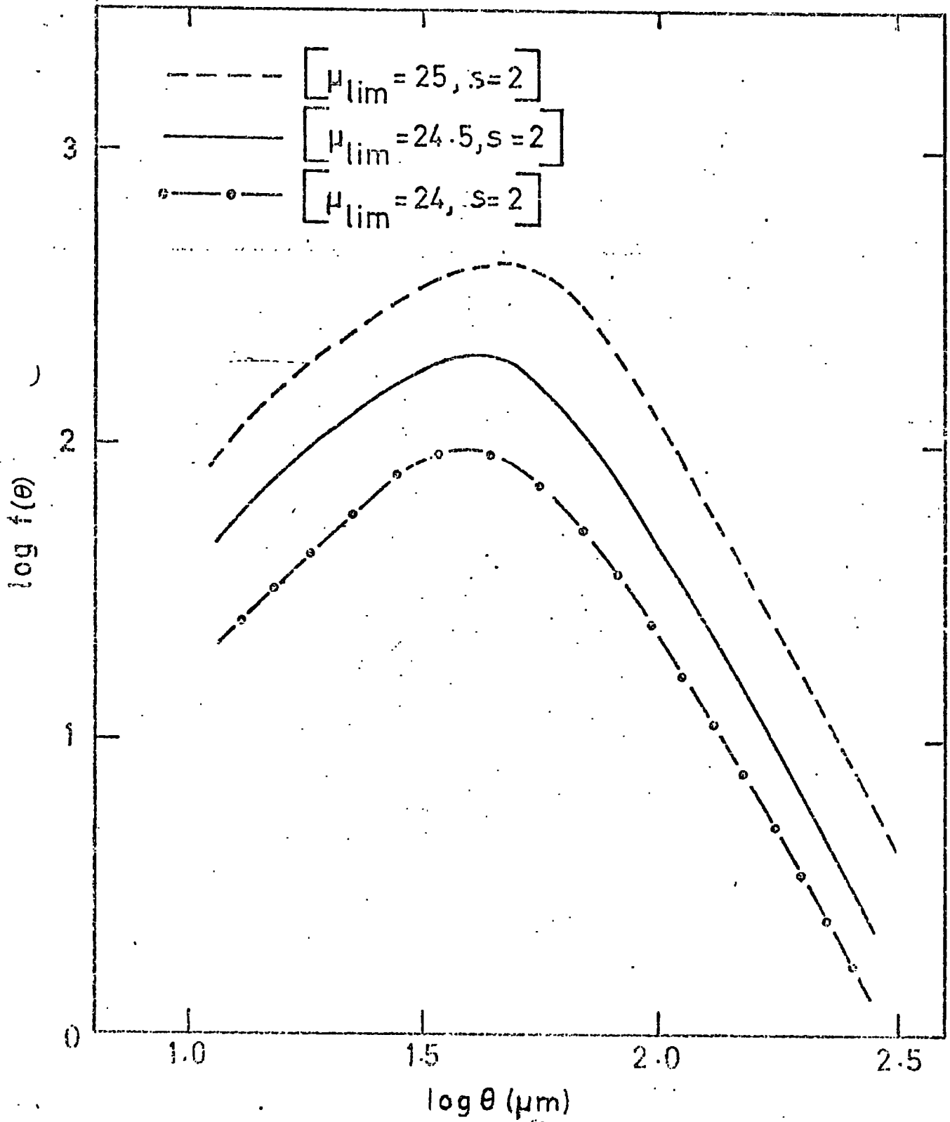
Expected differential count f(\theta) for J plate with S as shown and various values of \mu_{lim} as indicated.
