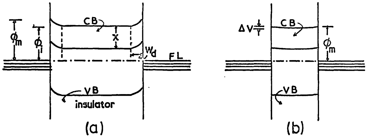
Contacts with depletion layers on, (a) thick film, (b) thin film.
