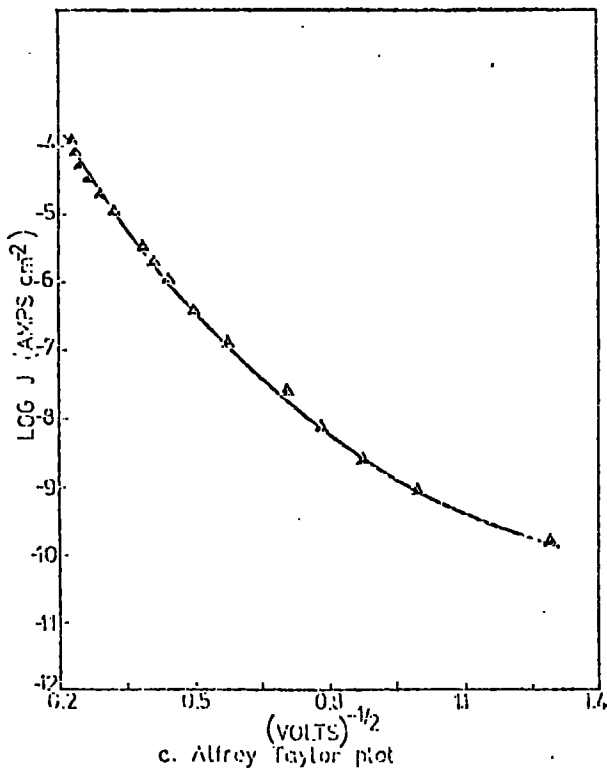
Fig. 8.2 Comparison of experimental results for \text{SiO}_x with different theories.
