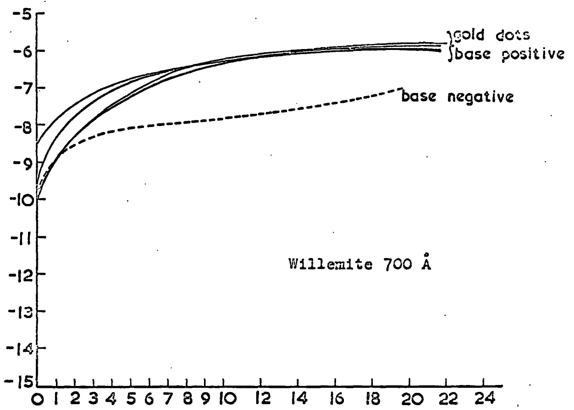
Smoothed I-V curves for sample S3
