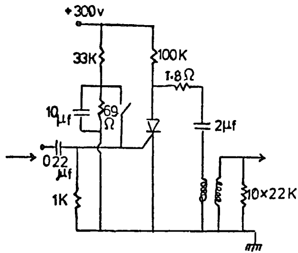
Figure 4.3 High voltage pulsing unit
