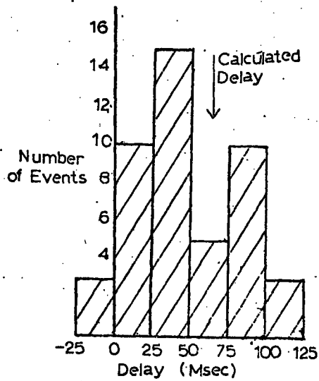
Histogram of Delay between Borehole and Surface Seismometers
