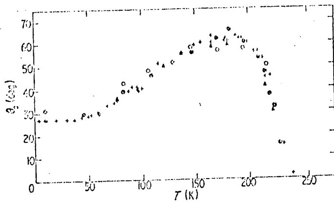
Plot of the angle between the magnetization and c axis as a function of temperature. +, present experimental points at 0.35 T; A, our extrapolated values; O, taken from neutron diffraction data of Cable and Wollan (1968) (O from 100 reflections, e from 602 reflections).
