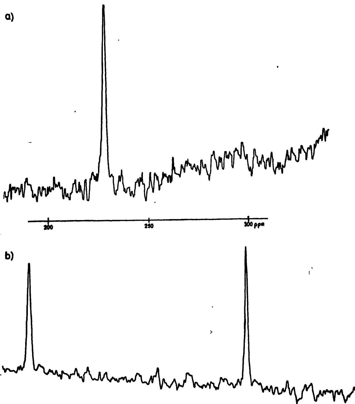
Fig 4 ^{31}\text{P} n.m.r. solution spectra
