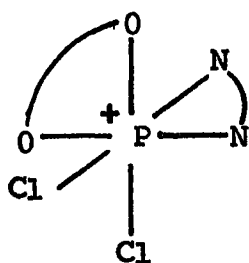
Possible isomers of \text{catPCl}_2\text{phen}^+ and \text{cat}_2\text{PCl}_2\text{dipy}^+
