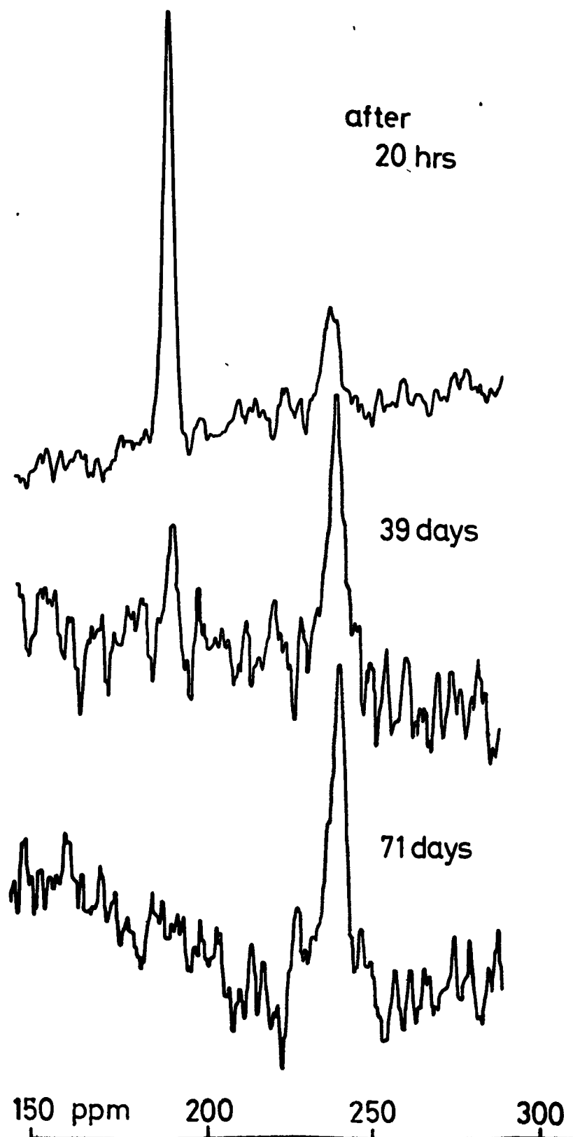
Fig 14 ^{31}\text{P} nmr solution spectrum of \text{PCl}_4^+\text{AlCl}_4^- + 2\text{equms} pyridine in nitrobenzene
