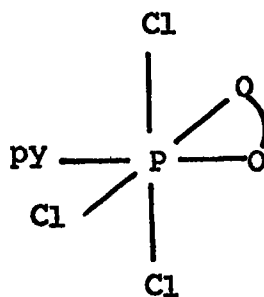
Isomers of \text{catPCl}_3.\text{pyridine}
