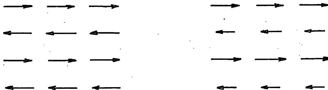
(a) Antiferromagnetic
