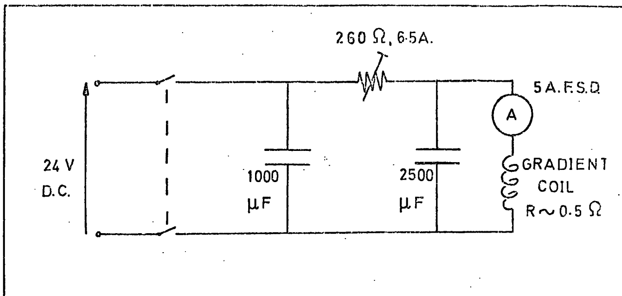
FIG. 4.11 SMOOTHING CIRCUIT FOR GRADIENT COIL SUPPLY
