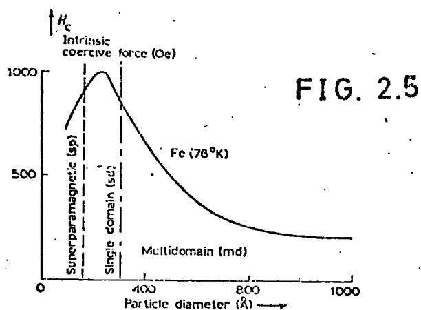
Coercive force for iron powder as a function of particle diameter (MEIKLEJOHN [1953]).
