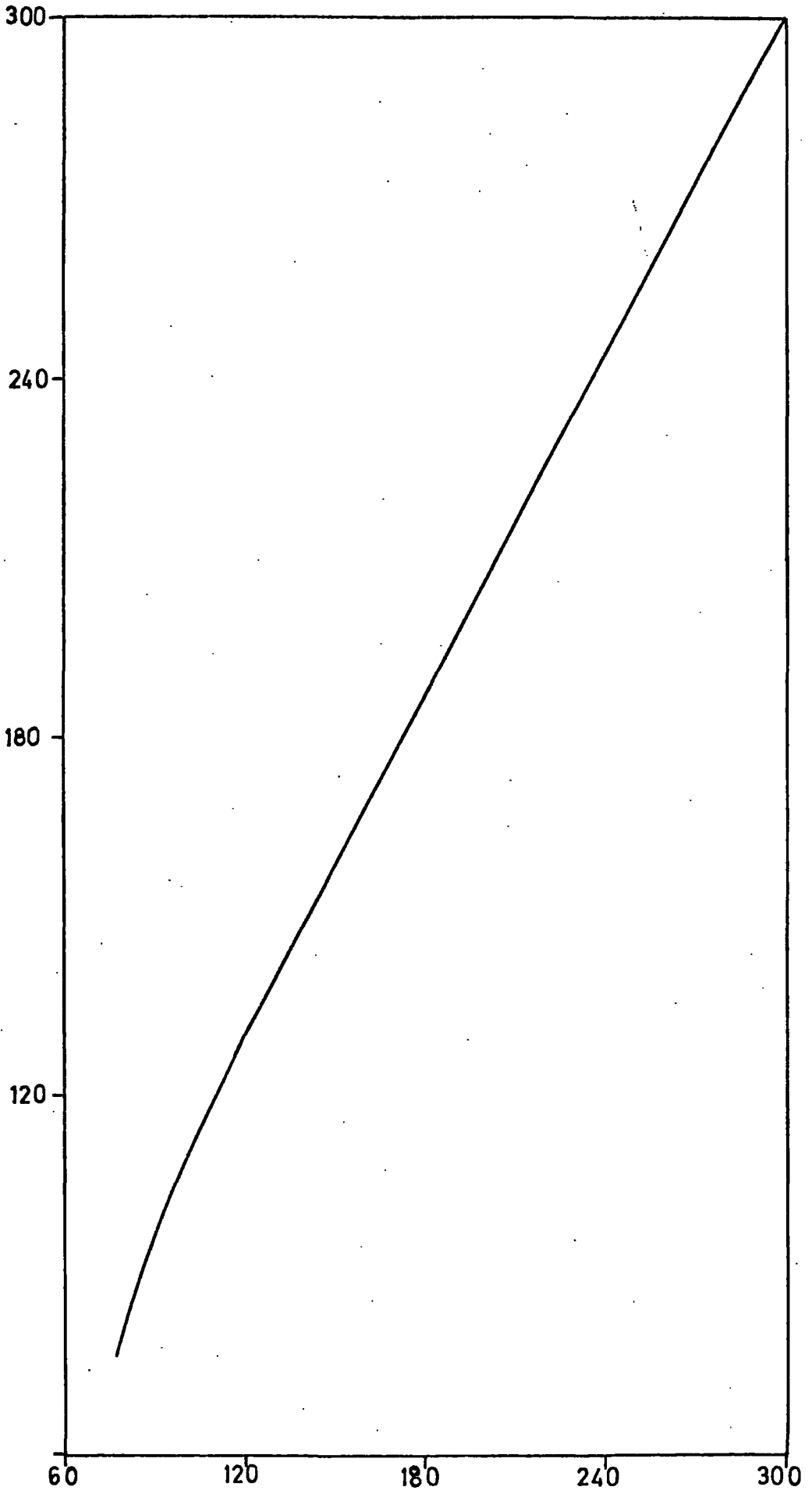
FIG. 4.19 TEMPERATURE CALIBRATION
