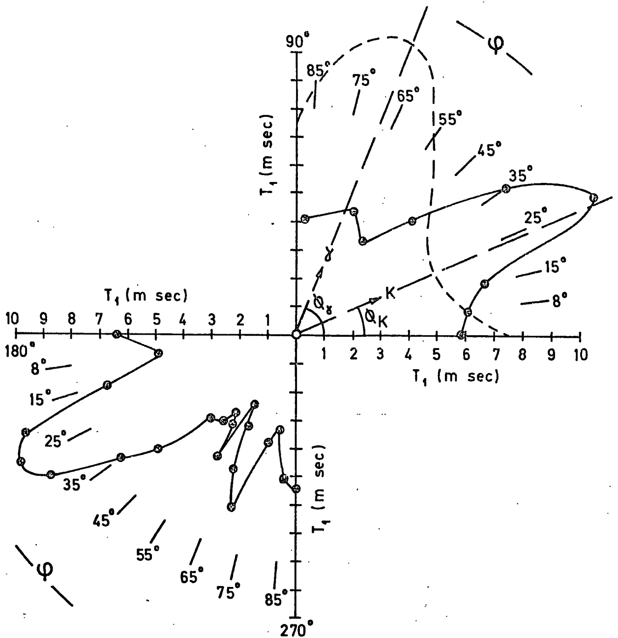
FIG.4.12 T_1 - Angular variation in the \phi - plane for Gd^{3+}/CaWO_4 (0.005%), temperature 4.2K, frequency 37.5 GHz, compared with ultrasonic measurements of Young's modulus in the same plane (dotted curve).
