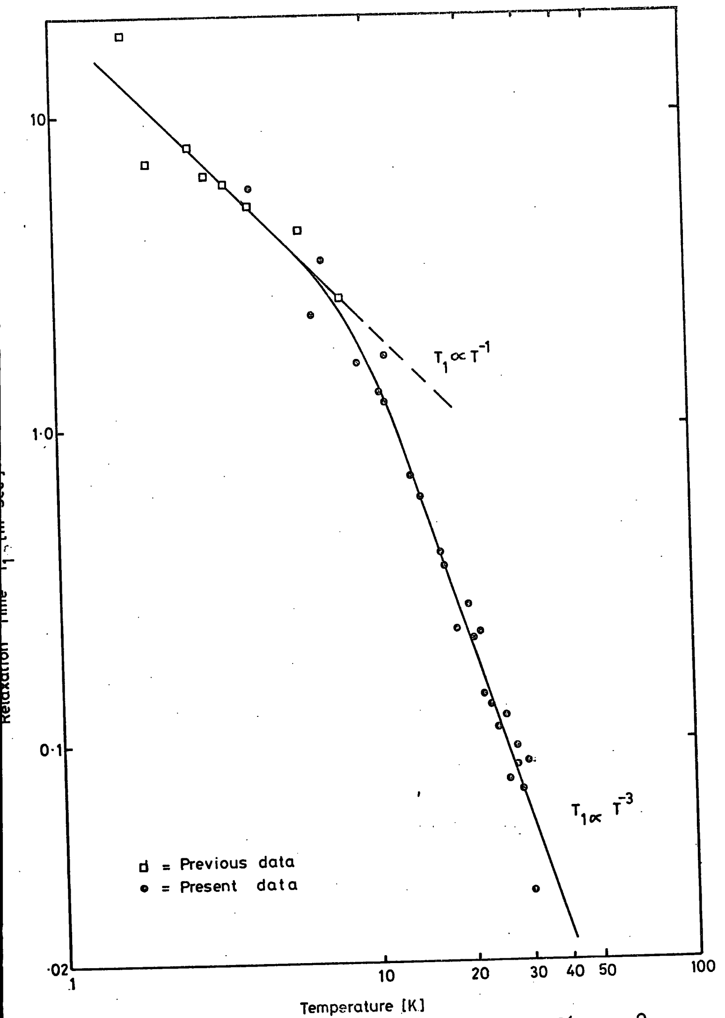
FIG 4.5 Temperature dependence of T_1 , \text{Gd}/\text{CaWO}_4 [0.005%], \varphi = 8^\circ Frequency 37.5 GHz.
