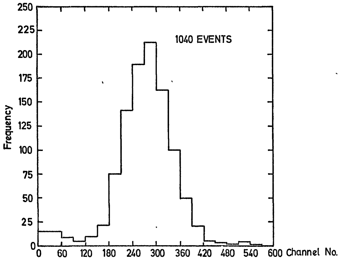
(b) T.A.C. distribution for detector 33.
