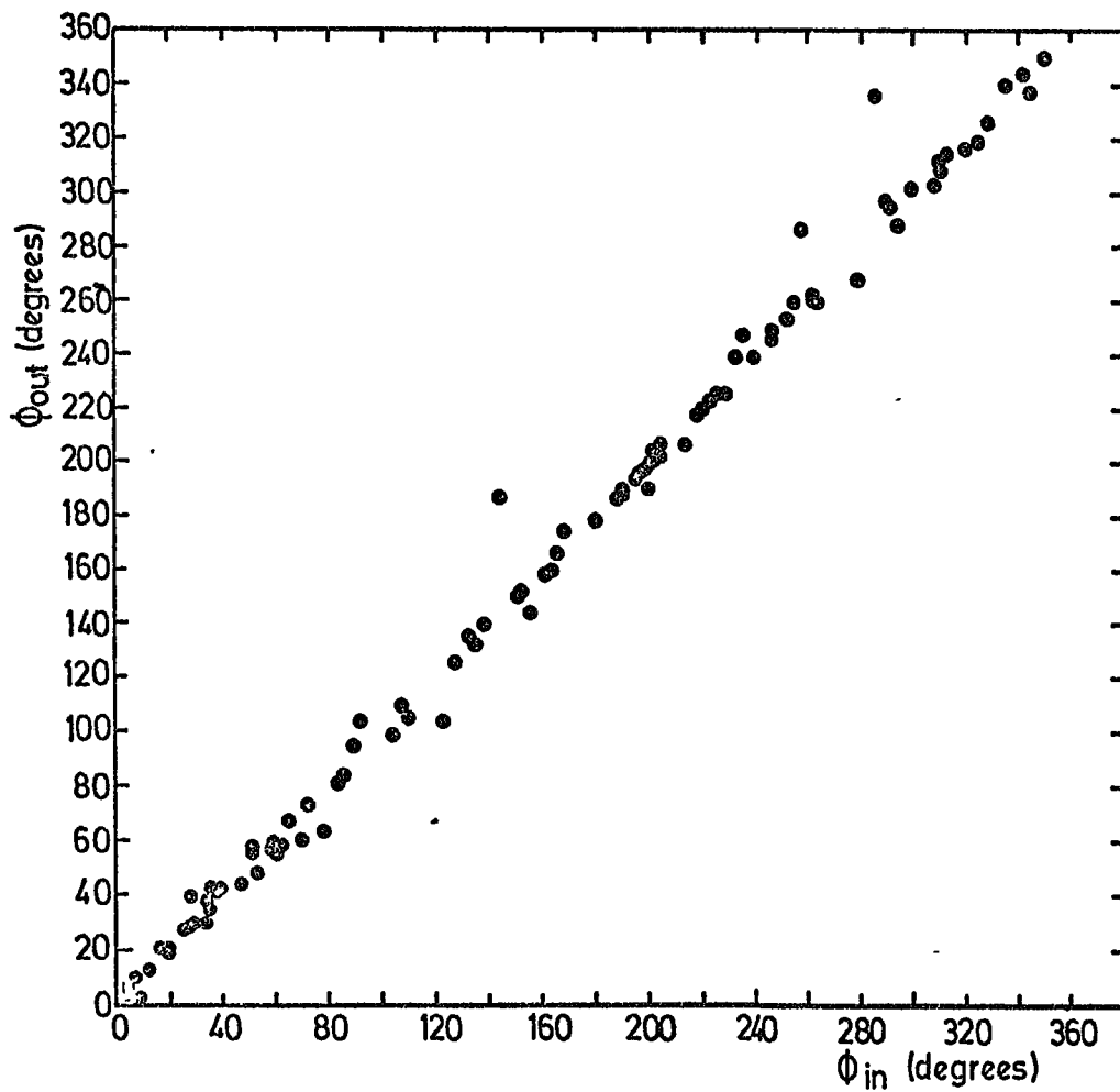
Figure 6.6 (b). \phi_{in} versus \phi_{out} for simulated showers. The three points off the main line had \theta < 5^\circ .
