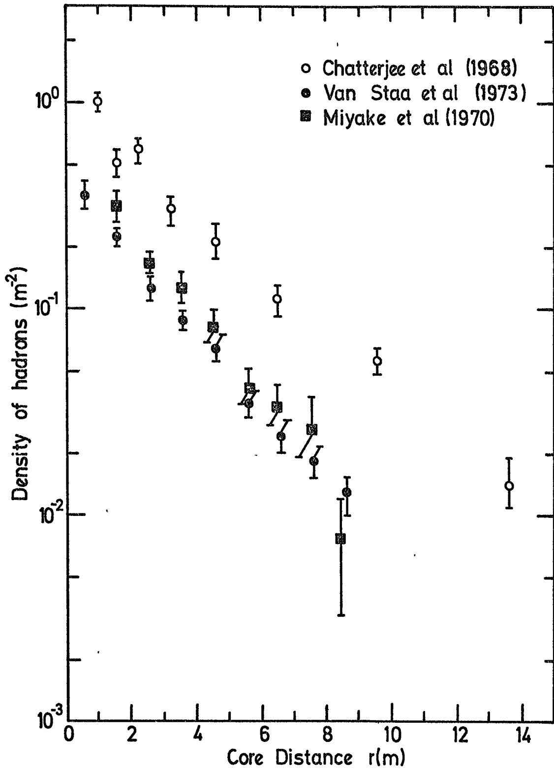
Figure 2.10. The lateral distribution of hadrons in air showers. (See Table 2.2.)
