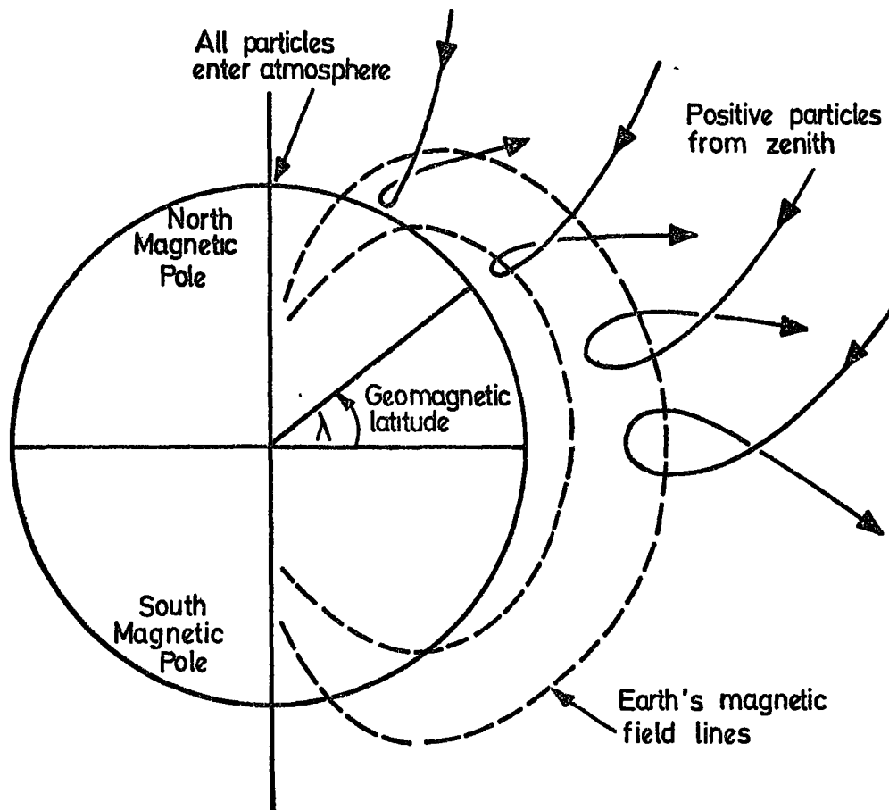
Figure: 1.1. Deflection of cosmic ray particles in the Earth's magnetic field.
