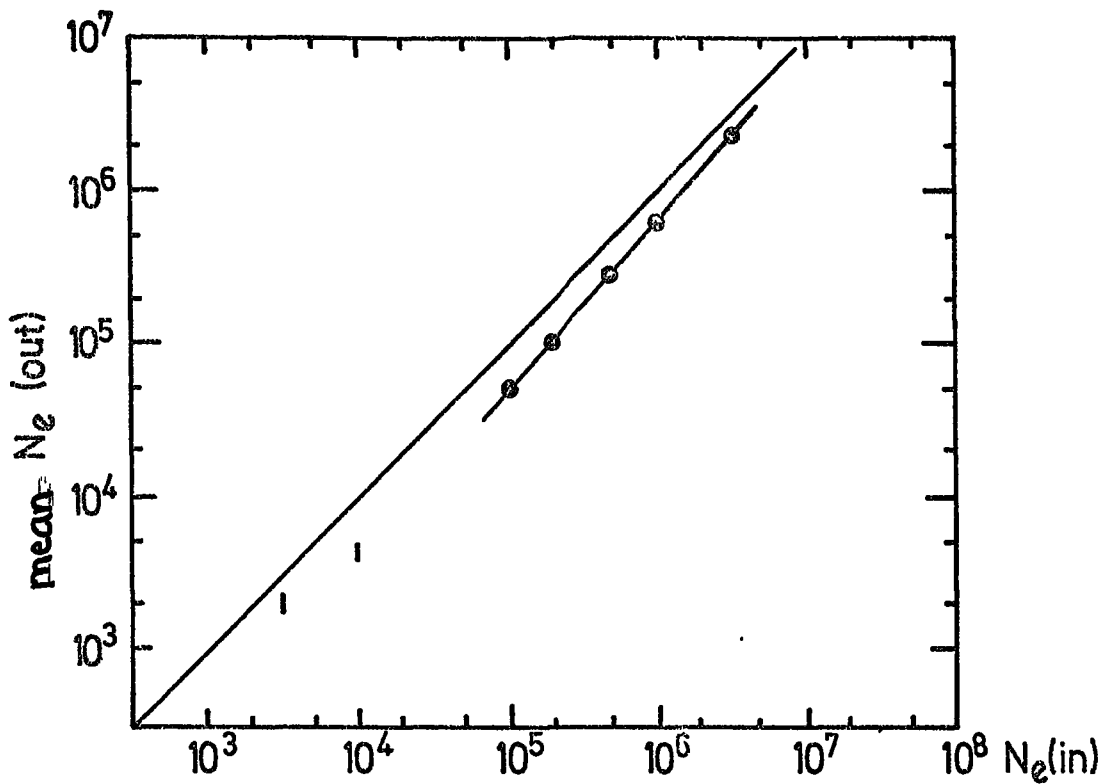
Figure 6.8. The response of the analysis programmes to simulated shower data. N_e(\text{in}) is the shower size fired at the array. N_e(\text{out}) is the analysed shower size.
