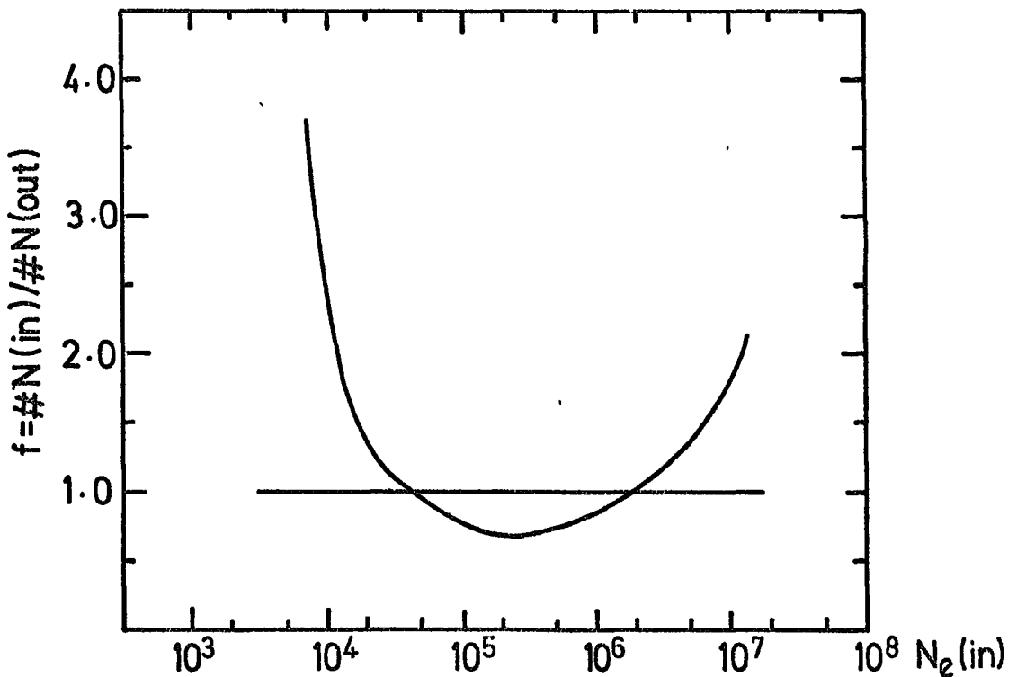
Figure 6.9. The response of the analysis programmes to simulated shower data. For a number of showers fired at the array of size N_e(\text{in}) a fraction f_i are returned as being within the array acceptance. (Array triggering probability = 1.0).
