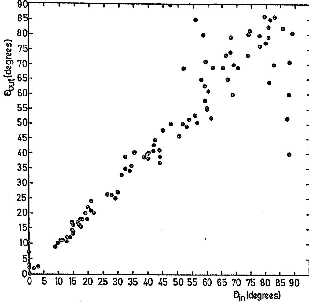
Figure 6.6(a). \theta_{in} versus \theta_{out} for simulated showers.
