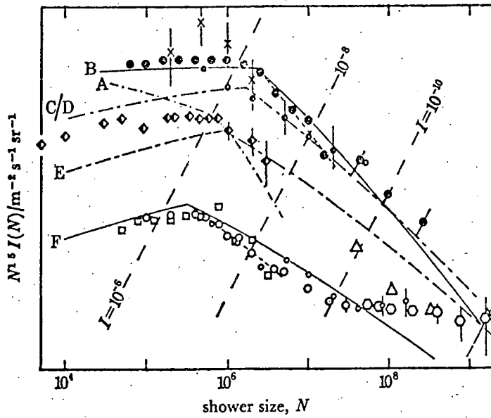
Fig A-3 Integral size spectrum of showers at various altitudes. For comparison, the expected size spectra for a power-law primary spectrum with differential exponent changing from -2.5 to -3.3 at 4 \cdot 10^{15} eV primary energy are shown. From Hillas (1974)
