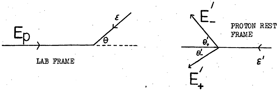
Fig 3-1. Geometry of pair-creation in a proton-photon interaction, illustrating notation used.
