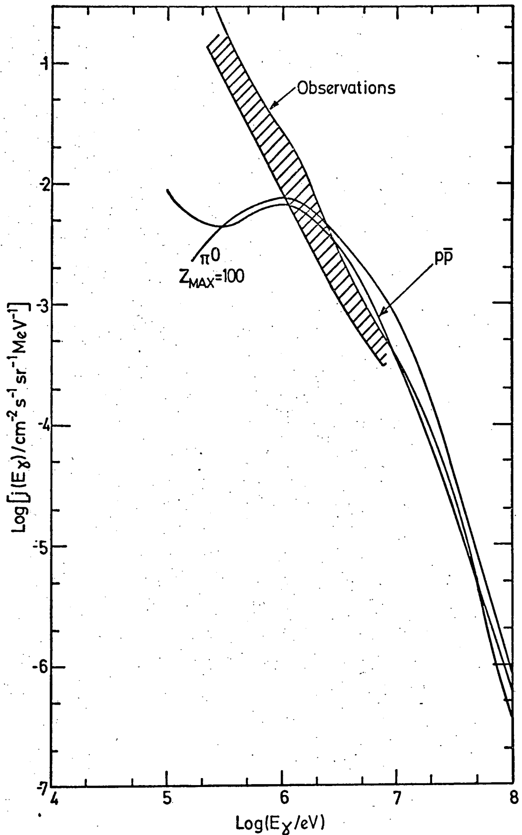
Fig 1-7 Comparison of two models for the gamma-ray background with a summary of the data in Fig 1-6. The models are 1) redshifted pion-decay spectrum from CR-gas interactions at early epochs ( z \sim 100 ), 2) matter-antimatter annihilation in baryon-symmetric cosmology. Both theoretical spectra are from Stecker (1975).
