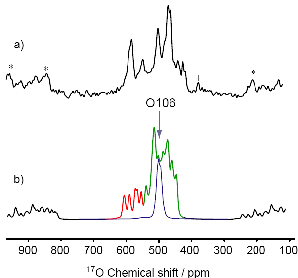
Figure 4-16 Comparison of (a) experimental MAS NMR spectrum of \gamma - ZrW_2O_8 and (b) simulated NMR spectrum based on ^{17}O NMR parameters (shifts and quadrupolar couplings) derived from DFT calculation on a neutron structure of \gamma - ZrW_2O_8 (25) . The calculated pattern has been shifted by +263 ppm as for the \alpha -phase calculations. The resonances in red and green show the calculated W-O-W and W-O-Zr oxygens respectively. O106 (see Figure 4-6) is shown in blue.
