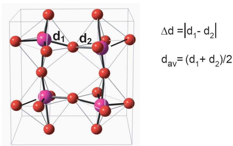
Figure 5-13 Schematic representation of the \text{WO}_6 arrangement on P2_1/n \text{WO}_3 structure showing the d_1 and d_2 distances and the expressions of the average bond distance ( d_{av} ) and asymmetry ( \Delta d ) around a given oxygen.
