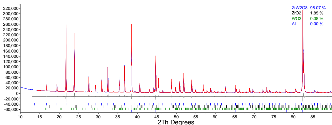
Figure 4-11 Rietveld refinement plots of the X-ray diffraction data from the room temperature enriched \alpha\text{-ZrW}_2\text{O}_8 (d9_01959). Rwp = 5.576 %
