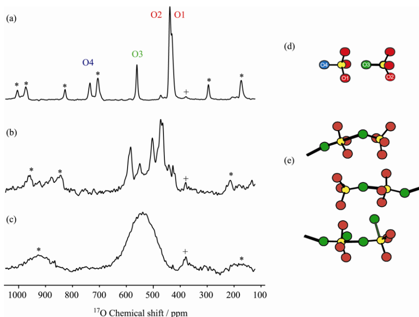
Figure 4-14 ^{17}O MAS NMR spectra for three phases of ZrW_2O_8 : (a) the cubic, \alpha -phase (288 scans with a recycle delay of 60 s), (b) the \gamma -phase (164 scans with a recycle delay of 34 minutes), and (c) the amorphous phase (288 scans with a recycle of 128 s). The magic-angle spinning rate was 25 kHz for (b) and (c), and 18 kHz for (a). Asterisks indicate spinning sidebands, while the + indicates the natural-abundance ^{17}O signal from the zirconia rotor (22) . On the right are schematic illustrations of the local tungsten environments in (d) \alpha - ZrW_2O_8 and (e) \gamma - ZrW_2O_8 .
