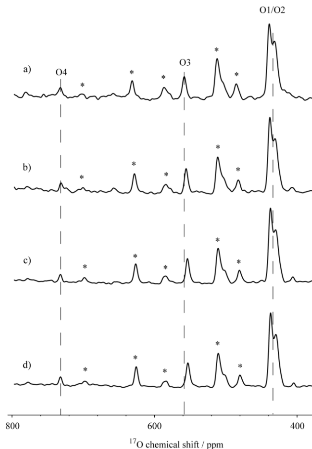
Figure 4-17 Variable temperature experiments on \alpha - ZrW_2O_8 recorded at 5 kHz in a 4 mm rotor on a 500 MHz Varian Chemagnetics a) RT, b) -50^\circ\text{C} , c) -100^\circ\text{C} , d) -120^\circ\text{C} .
