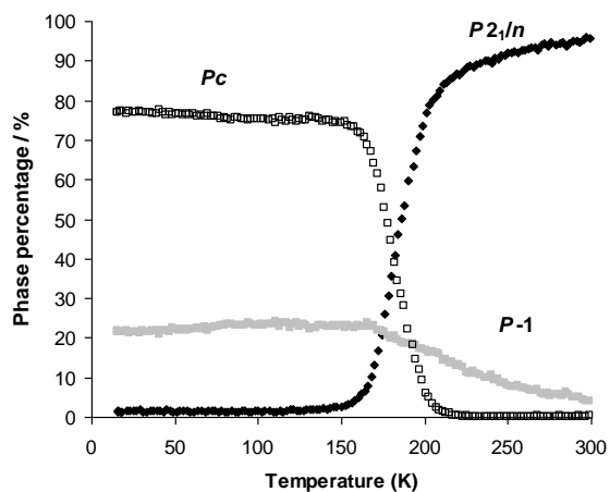
Figure 5-10 a),b) Selected portions ( 22.5^\circ < 2\theta < 25^\circ and 49^\circ < 2\theta < 52^\circ ) of the X-ray data acquired and c) Results of the refinement of the variable temperature (cooling from 300 K to 16 K) powder pattern of AS026B (left) and AS026C (right) enriched sample experiments (d9_02979 and d9_03124 respectively). The full, empty and grey data points correspond to the evolution of the P2_1/n (monoclinic), P1 (triclinic) and Pc (monoclinic) phases respectively.
