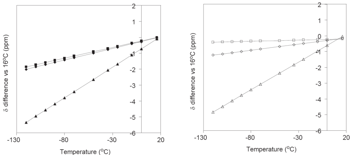
Figure 4-21 Comparison between the variations of experimental (full) and calculated (empty) ^{17}O chemical shift differences in ZrW_2O_8 as a function of temperature.
