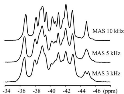
Figure 2-4 1D ^{31}\text{P} MAS NMR spectra of \text{ZrP}_2\text{O}_7 recorded at different spinning speeds
