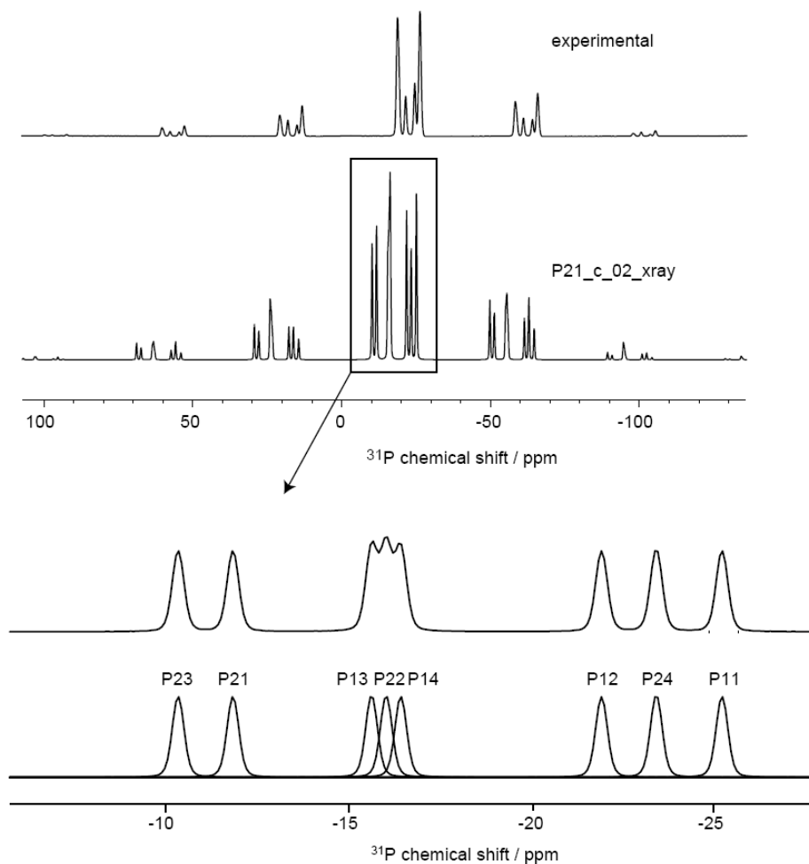
Figure 3-7 Experimental MAS NMR pattern recorded at 0^\circ\text{C} at 8 kHz on (\text{MoO}_2)_2\text{P}_2\text{O}_7 sample (SEL251) (top) and simulated spectra obtained from CASTEP calculations on \text{P}_2\text{O}_7 structure ( \text{P}_2\text{O}_7 code) provided by Lister (bottom).
