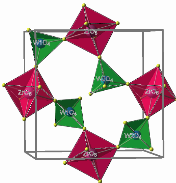
4-1 Schematic representation of the room temperature cubic ZrW_2O_8 structure.
