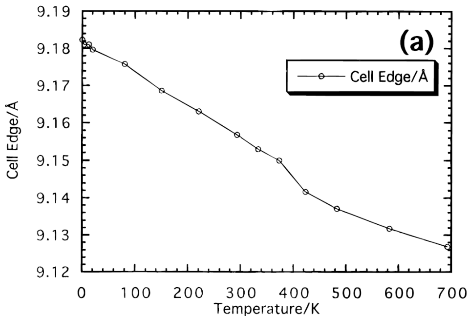
Figure 4-3 Evolution of the cell parameter of the cubic ZrW_2O_8 as a function of temperature.
