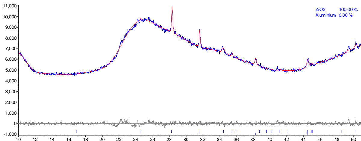
Figure 4-13 Rietveld refinement plots of the X-ray diffraction data from the room temperature of AS0012 (amorphous phase of ZrW_2O_8 (d9_01992)). Rwp = 1.63 %
