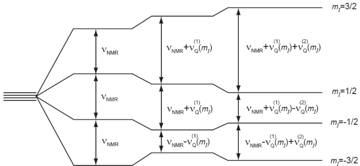
Figure 1-5 Influence of the first and second order quadrupolar interaction on the energy levels of a I=3/2 nucleus.
