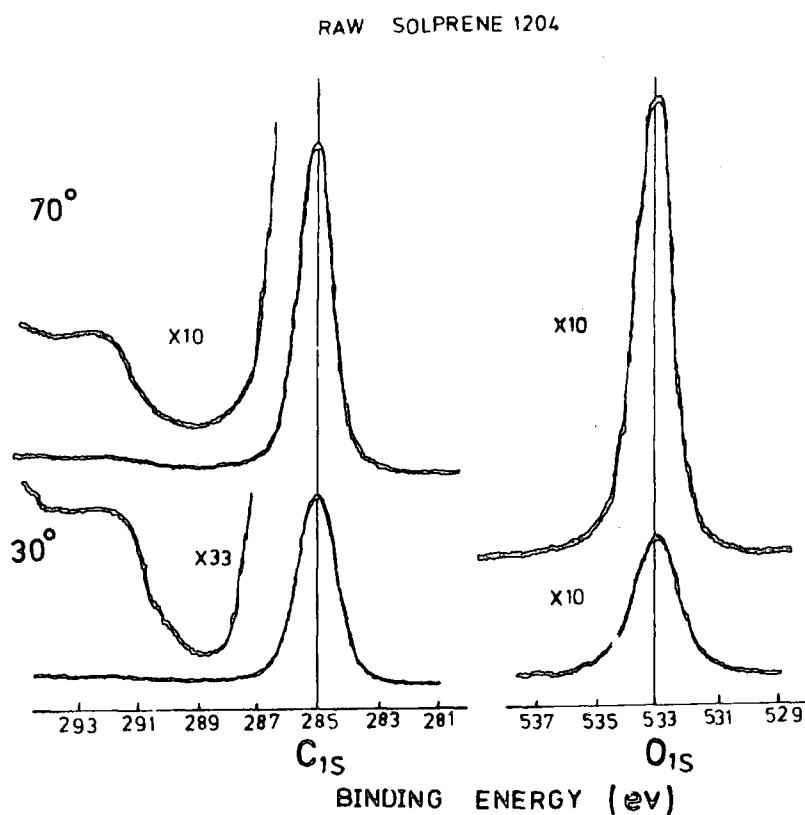
Figure 4.6. C_{1s} and O_{1s} levels for the as received, raw Solprene 1204, milled for 10 minutes and pressed for 5 minutes at 100^{\circ}\text{C} .
