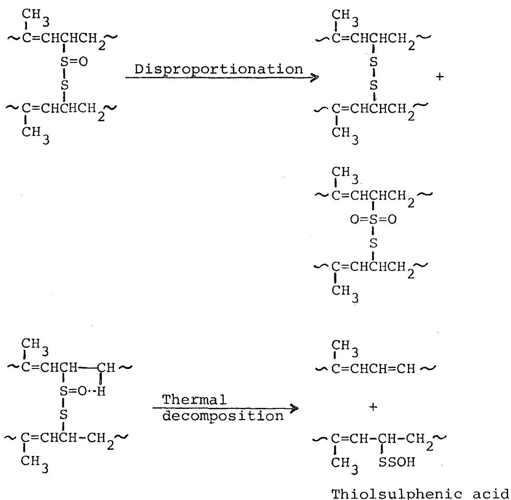
Scheme 7
