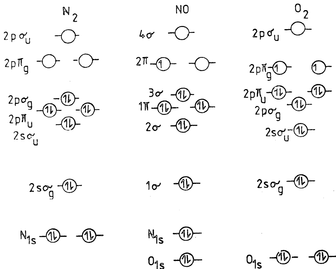
Figure 2.9. Electronic configurations of N_2 , NO and O_2 .
