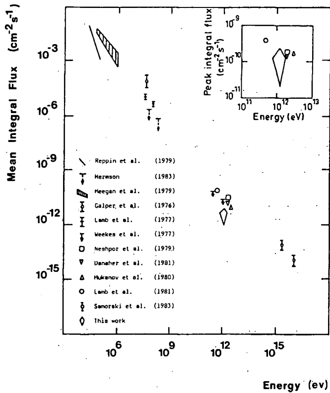
Figure 8.1 Energy Spectrum of Radiation from Cygnus X-3 in VHE Gamma Rays at X-Ray Phase 0.625.
