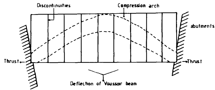
Theoretical load transfer in a Voussoir beam
