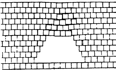
Trollope's Block Jointed Model (Trollope, 1966)
