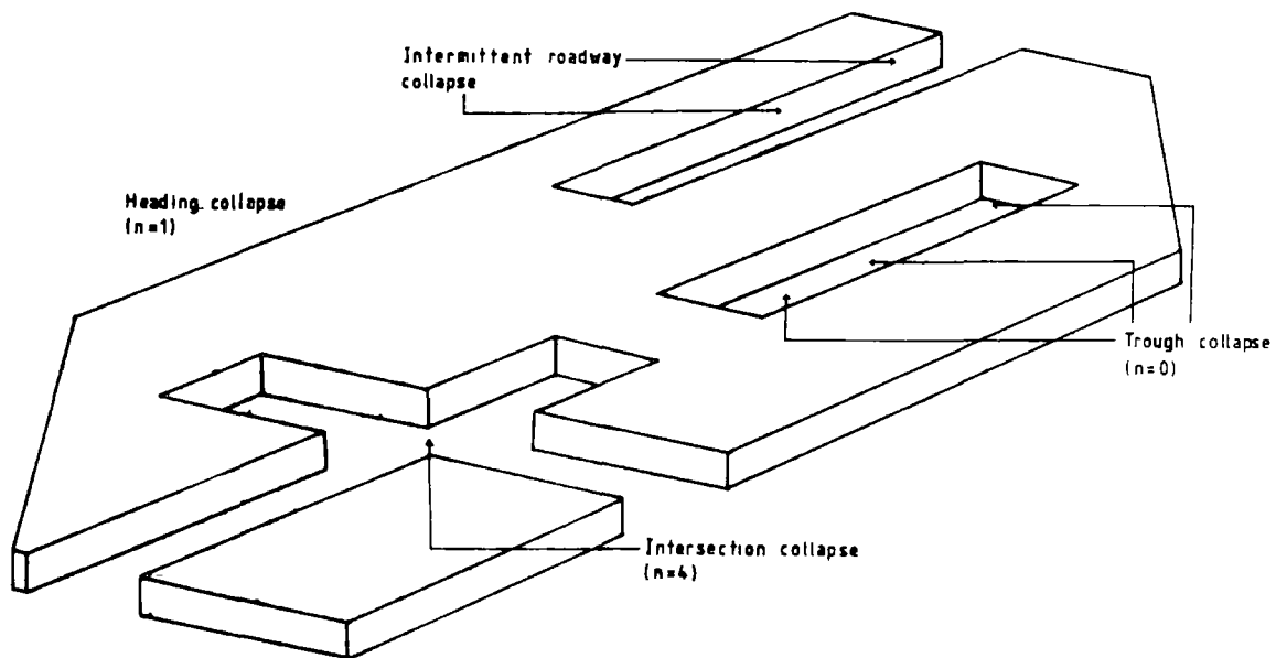
Figure 8.3 Possible locations for roof collapse.
