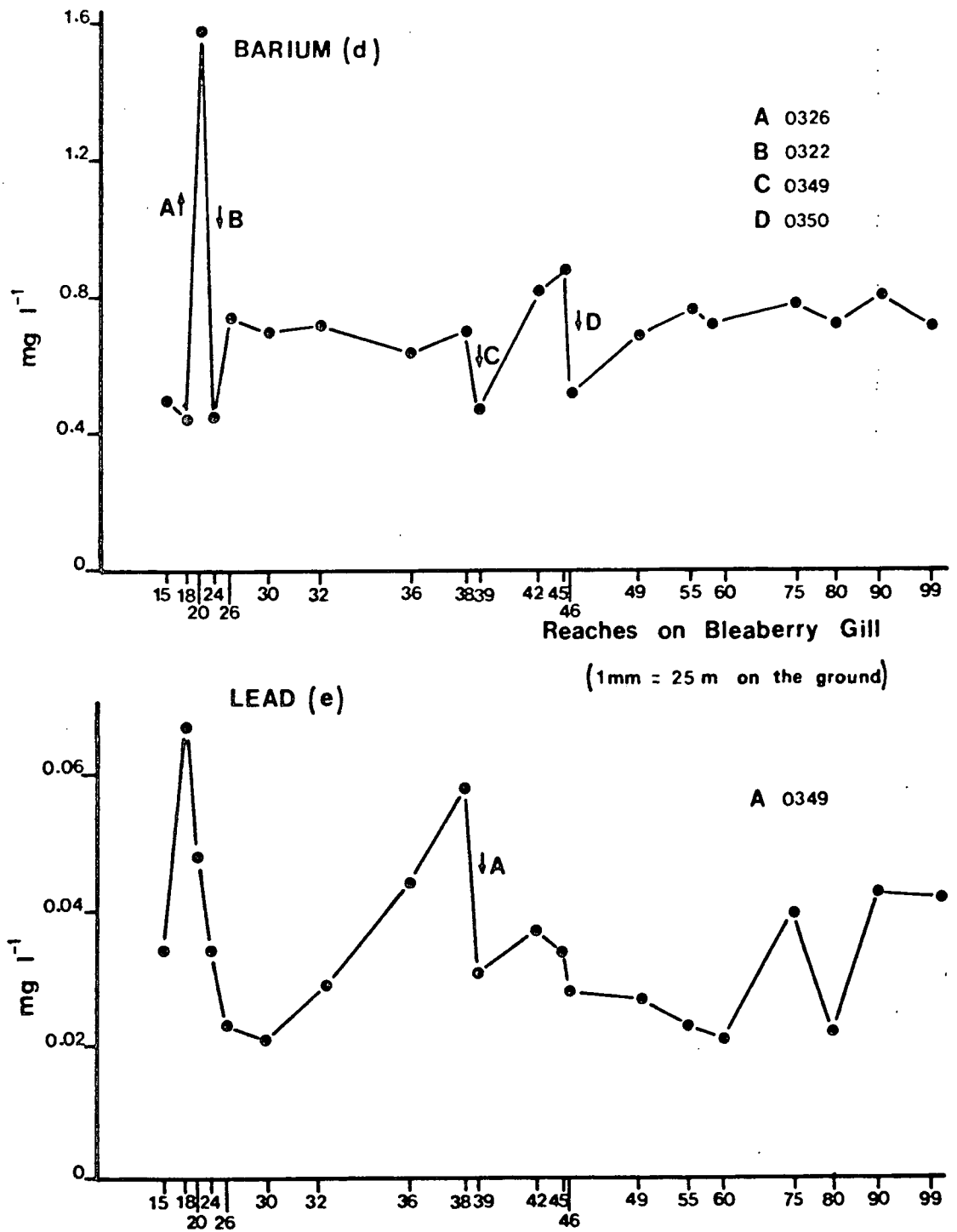
Fig. 4.1d-e Barium and lead in 'total' water (mg l -1 ) from 20 reaches on Bleaberry Gill (O212), 27.04.82. Fig. 3.2 gives reach locations. Arrows indicate input from tributaries which affected the aqueous metal concentration substantially
