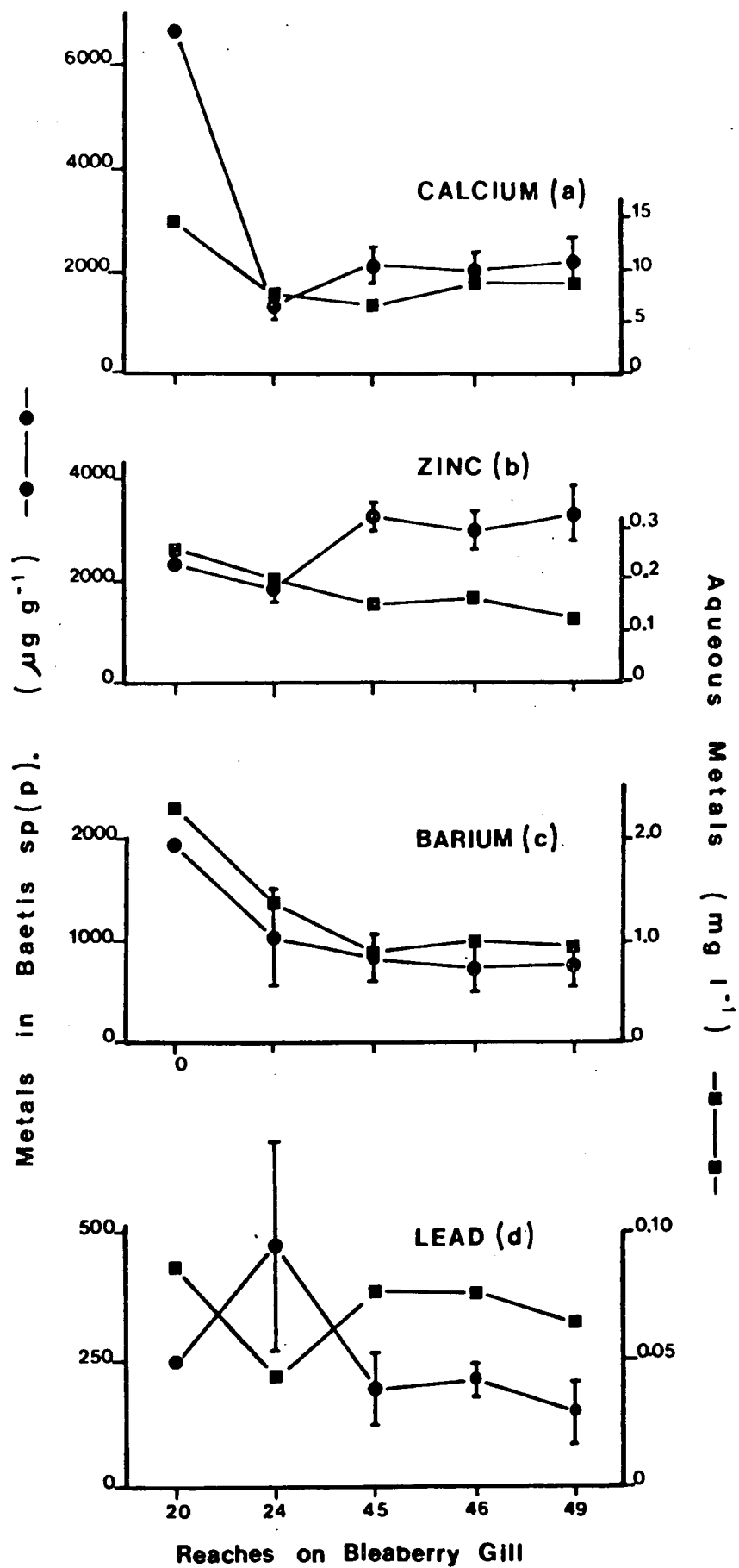
Figure 5.2a-d Metals in Baetis sp(p) . ( \mu\text{g g}^{-1} dry wt) compared with 'total' aqueous metal ( \text{mg l}^{-1} ) at five reaches on Bleaberry Gill, 24.06.82 Vertical bars represent 95% confidence limits of the mean
