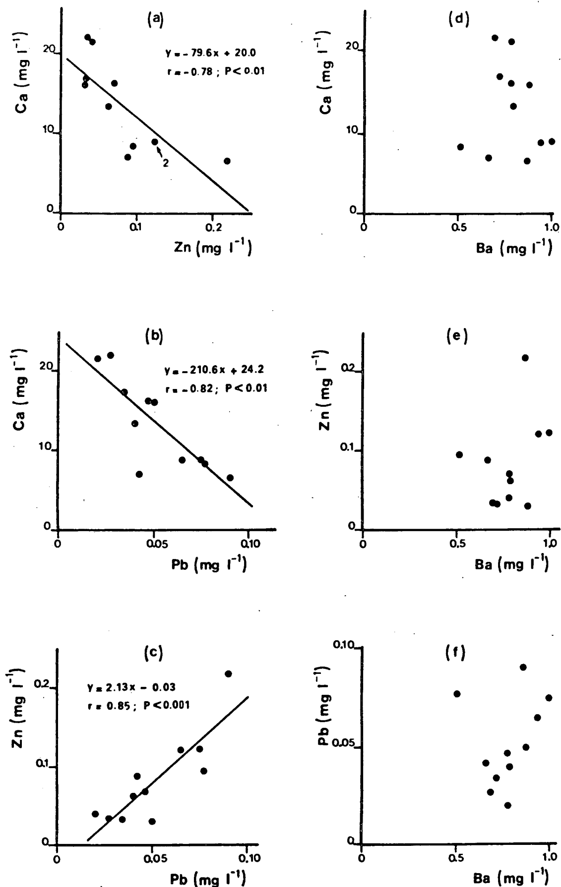
Fig. 4.2a-f Scattergrams showing the relationships between the concentrations of metals in 11 'total' water samples from one reach on Bleaberry Gill (O212 - 49)
