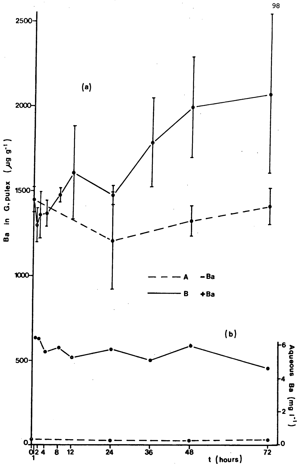
Figure 6.1 Influence of high aqueous barium ( 6\text{mg l}^{-1} ) on the barium concentration in G. pulex
