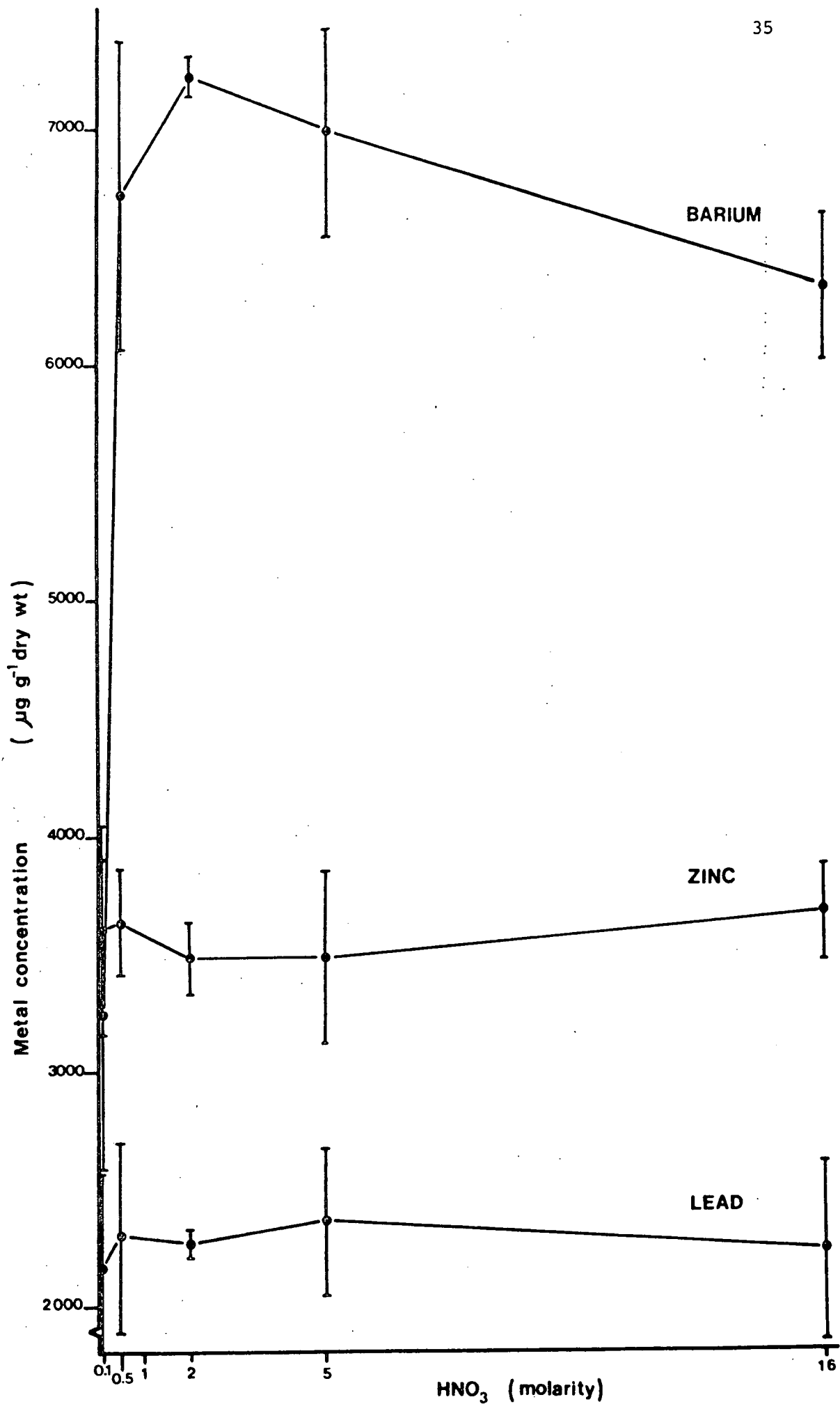
Figure 2.1b Zinc, barium and lead in Baetis sp(p) . digested in a range of nitric acid concentrations. Vertical bars represent 95% confidence limits of the mean
