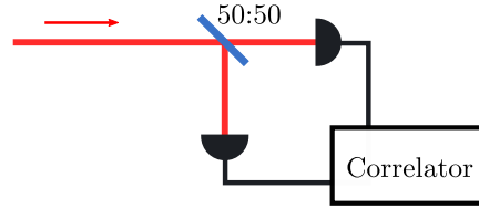
Figure 8.1: Hanbury Brown Twiss Interferometer. The input light is separated onto a pair of single photon counters using a 50:50 beam-splitter, and coincidence counts are detected as a function of delay \tau to build up the correlation function.
