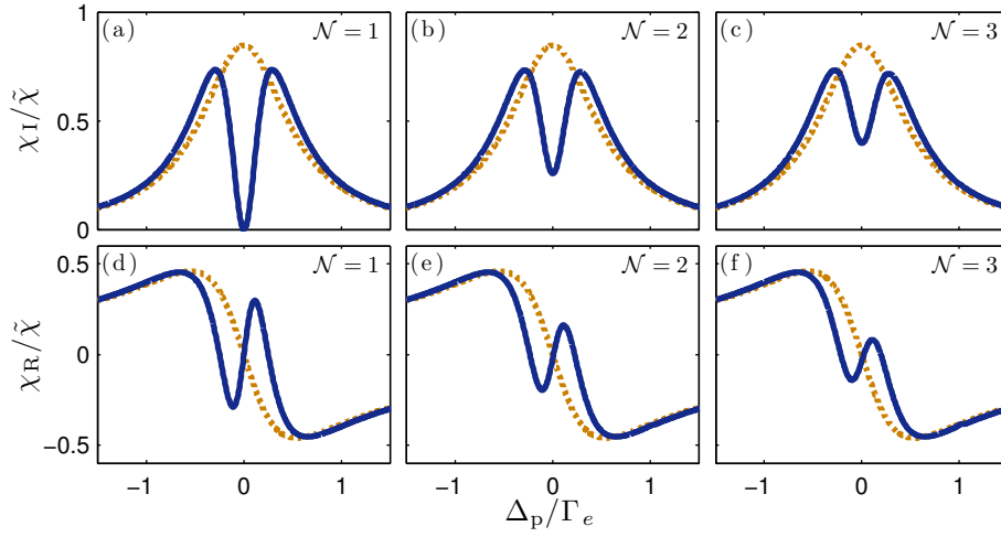
Figure 5.8: Resonant susceptibility for \Omega_p = \Gamma_e/4 , \Omega_c = \Gamma_e/2 and V = 2\Gamma_e , with the probe-only susceptibility plotted as a dashed line. \chi is scaled relative to the weak, probe-only resonant susceptibility \tilde{\chi} = 2\rho d_{eg}^2/\epsilon_0\hbar\Gamma_e .
