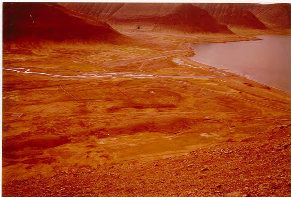
Fig. 3.54. View from Sandafell to the mouth of Kirkjubólssdalur.
