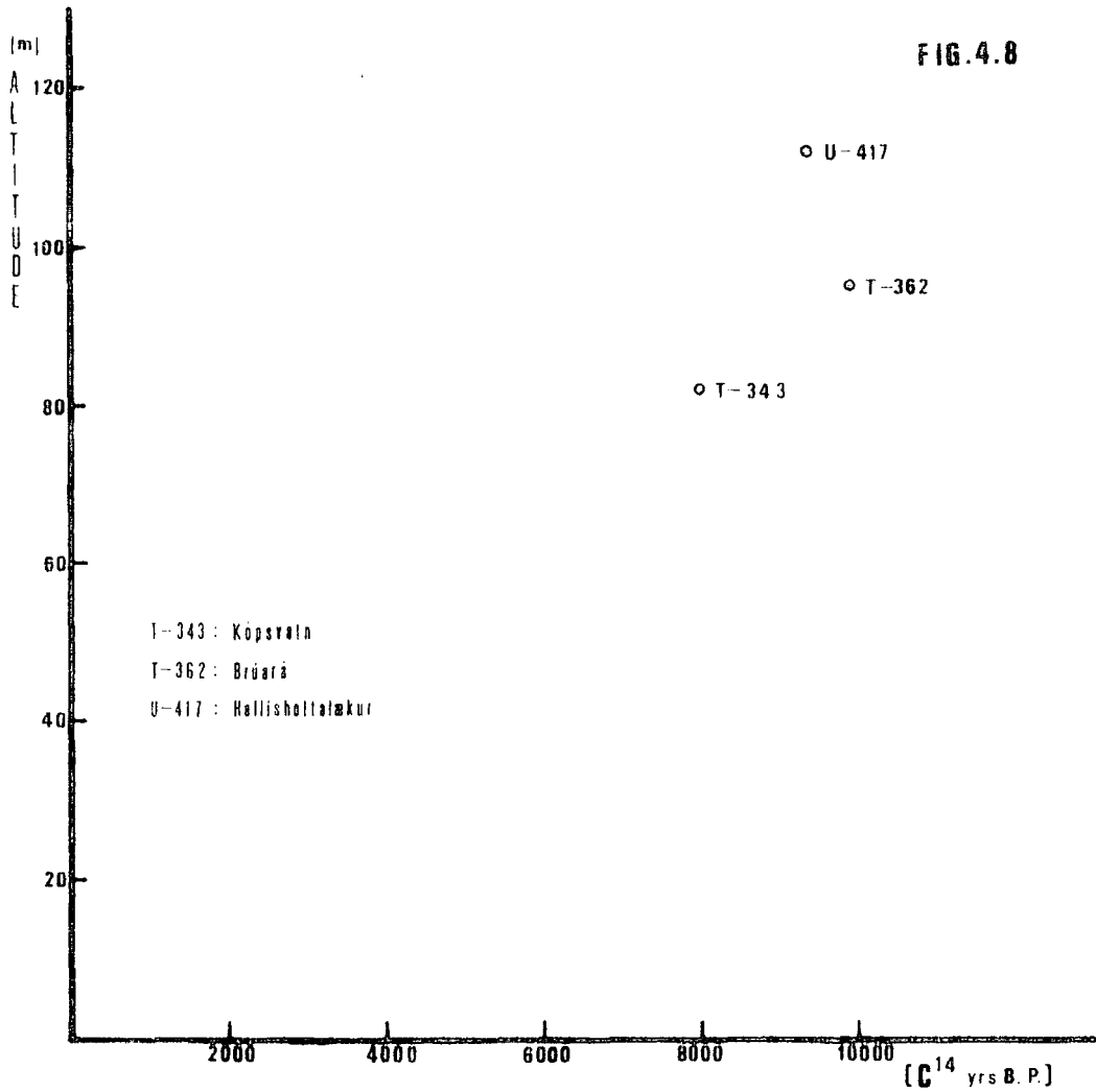
Fig. 4.8. An altitude/age plot of the three samples from the Hreppar district.
