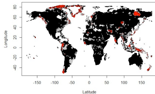
Figure 3.3: Map of extinct climate space in ordination and geographical space. In ordination space black and grey correspond to 2050 and 2000 climate space respectively and red corresponds to level of confidence that a point is extinct, brightest meaning most remote from all future points and dark green being closest. In the geographic map black points map land grid cells and the grey to red gradient maps likelihood of extinction in the same way as in ordination space.
