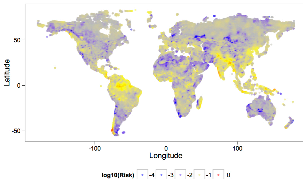
Figure 4.5: Additive combined risk across the world (climate change, GDP, population).
