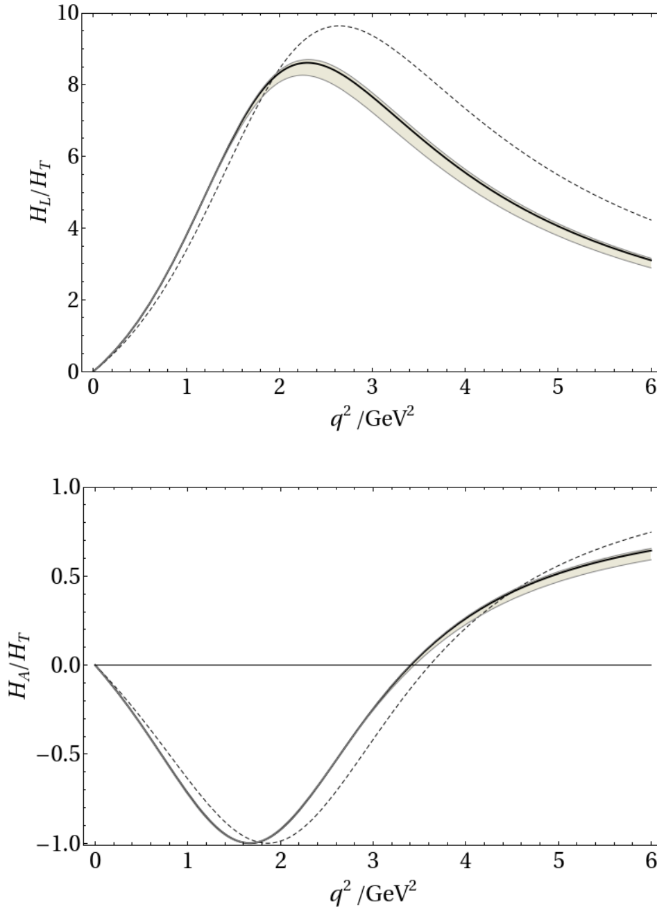
Figure 5.14: Ratios of observables H_L/H_T and H_A/H_T as a function of q^2 . Dashed lines indicate the SCET limit (5.23,5.24). Solid lines include the default estimates for the form-factor corrections from hard gluons, C_{f_i} and hard-collinear gluons, \Delta\xi_\Lambda , as well as kinematic corrections of order m_\Lambda/M_{\Lambda_b} . In order to illustrate the (tiny) uncertainty from the variation of \Delta\xi_\Lambda/\xi_\Lambda , the error has been blown up to an interval of [25%, 400%] of its default value (shaded error band).
