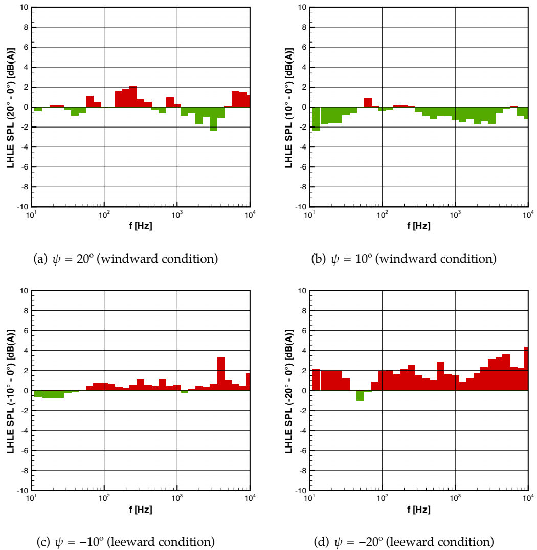
Figure 3.18: Steady AWT (Pininfarina) variation of LHLE cabin noise spectra at yaw (Geometry 1)
