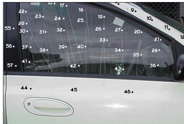
Figure 1.32: Side door pressure tappings, from Gilhome and Saunders (2002)
