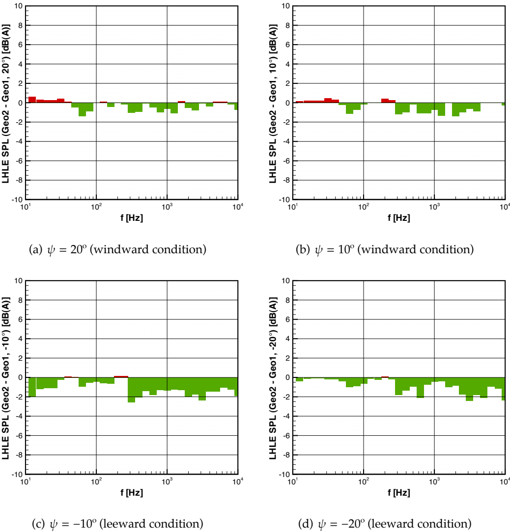
Figure 3.22: Steady AWT (Pininfarina) variation of LHLE cabin noise spectra at yaw between Geometry 1 and 2
