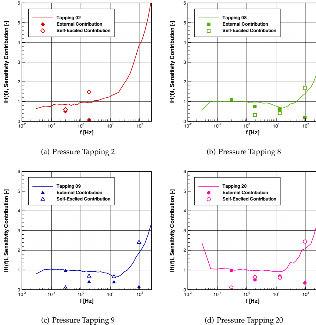
Figure 4.15: Contributions of external and self-excited unsteadiness to overall sideglass pressure transfer functions (Mirror wake region, Geometry 2 SG)
