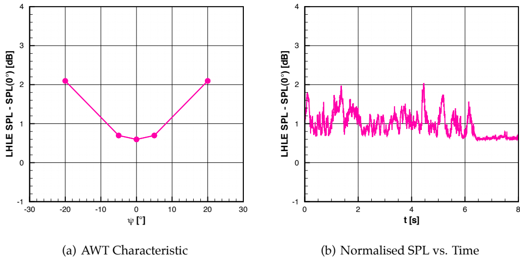
Figure 4.36: YawSens1Plus characteristic and simulated time history
