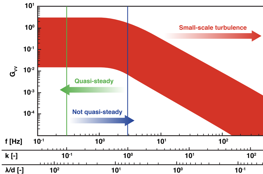
Figure 1.30: Expected bounds for vehicle quasi-steady response
