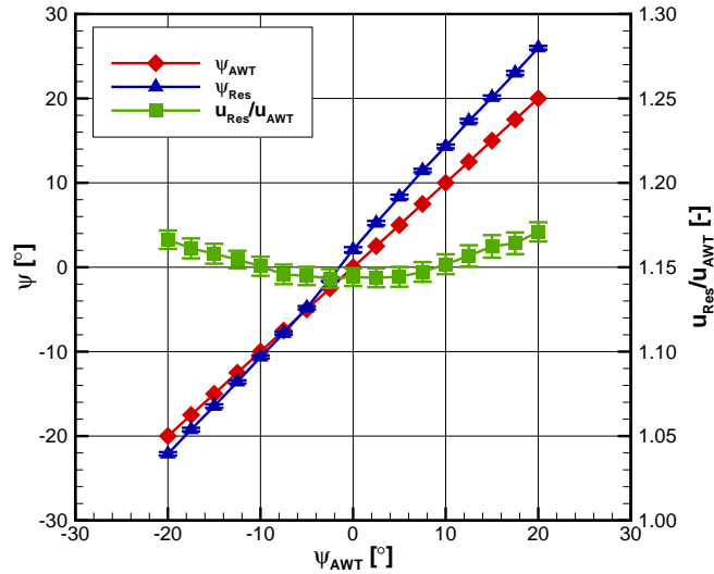
Figure 2.32: Ford AWT: Error of roof-mounted probe measurements (Geometry 1)
