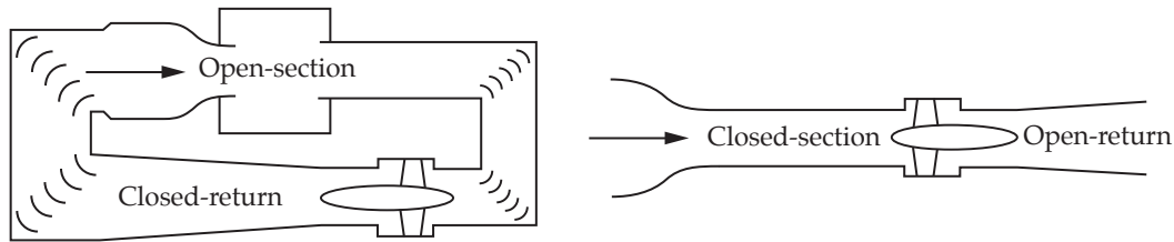
(a) Open-section, closed-return
