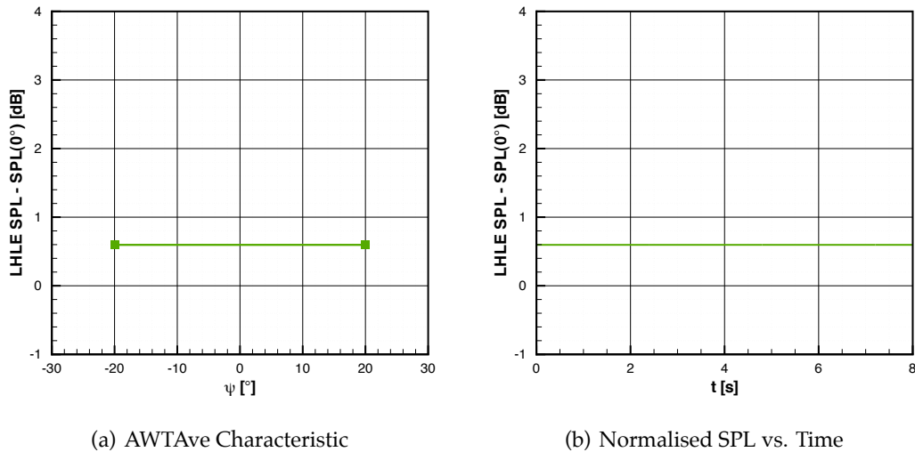
Figure 4.40: AWTave characteristic and simulated time history
