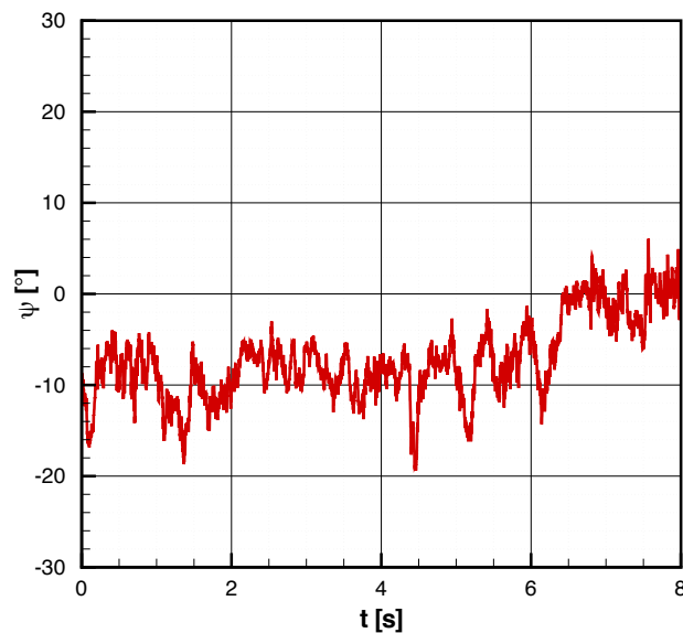
Figure 4.32: Yaw time history 20090619bHist3, 8–16s used in subjective assessment
