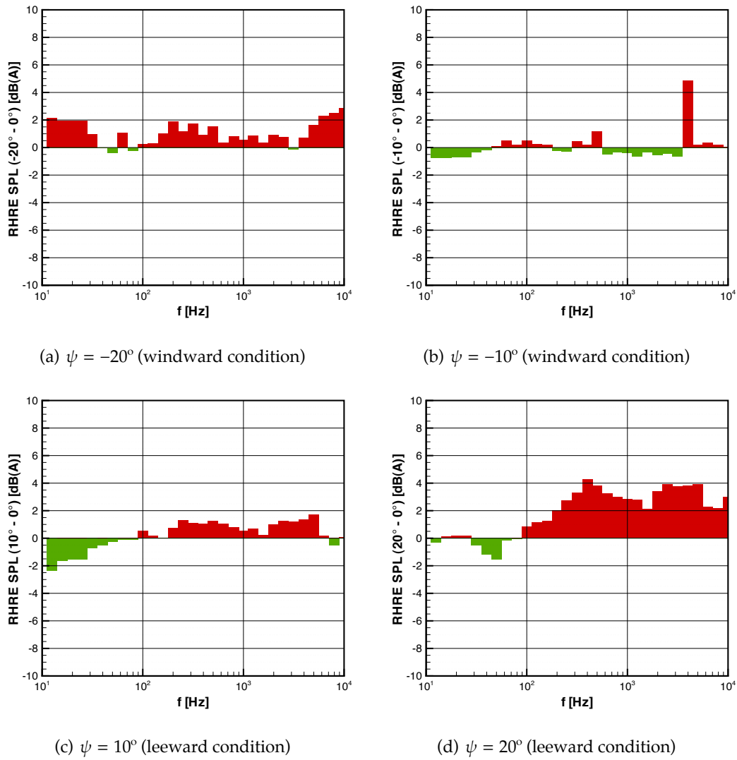
Figure 3.19: Steady AWT (Pininfarina) variation of RHRE cabin noise spectra at yaw (Geometry 1)
