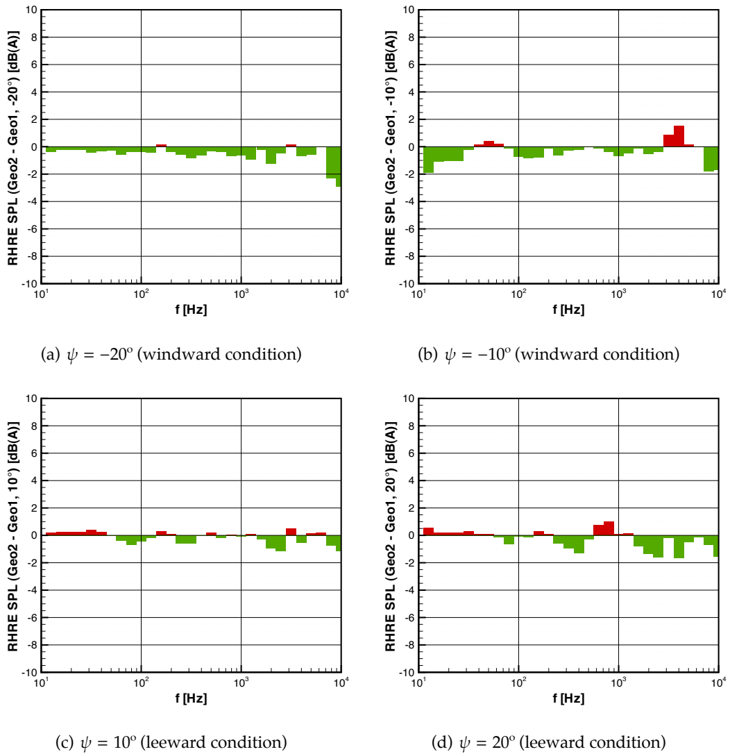
Figure 3.23: Steady AWT (Pininfarina) variation of RHRE cabin noise spectra at yaw between Geometry 1 and 2
