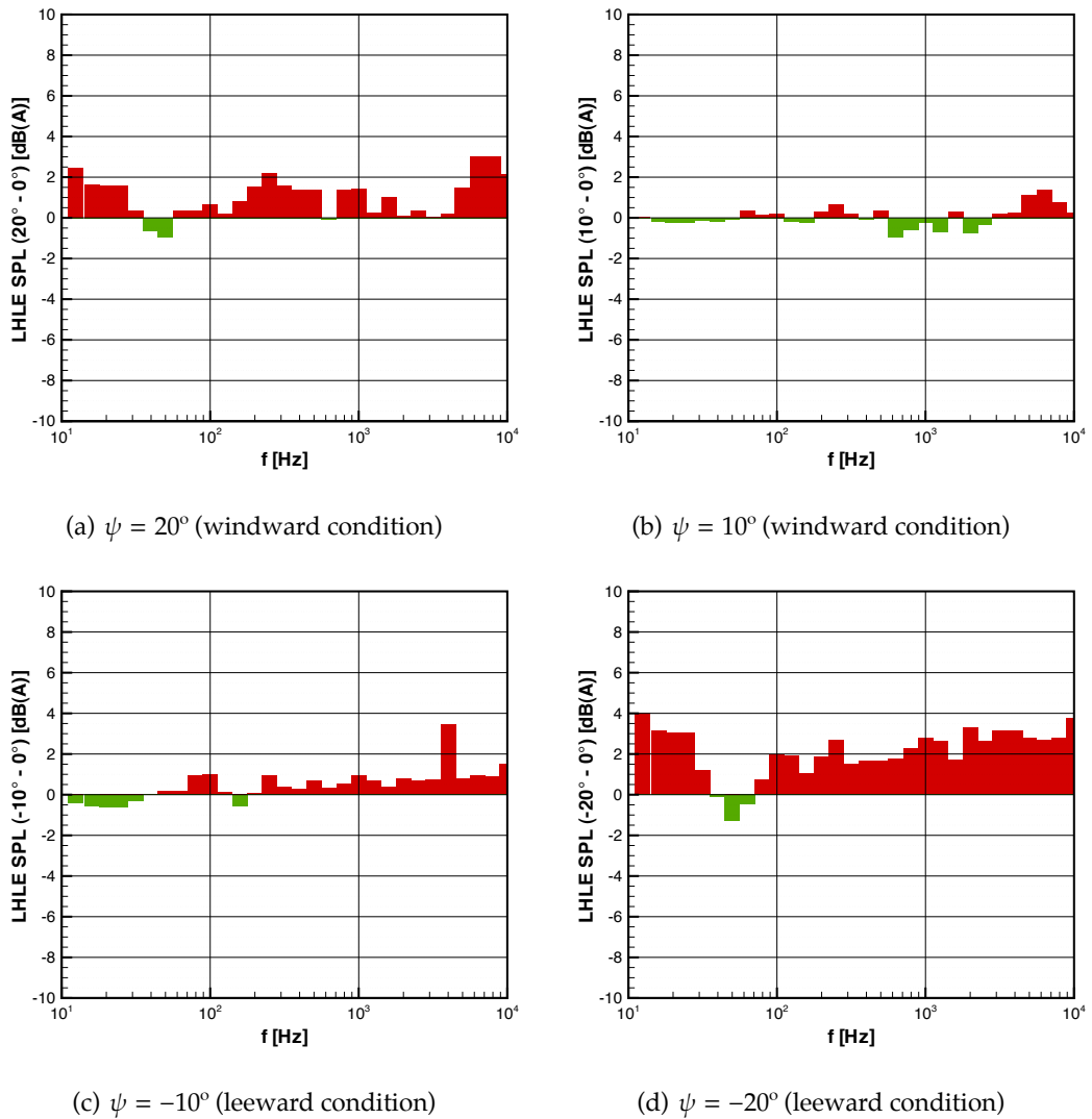
Figure 3.20: Steady AWT (Pininfarina) variation of LHLE cabin noise spectra at yaw (Geometry 2)
