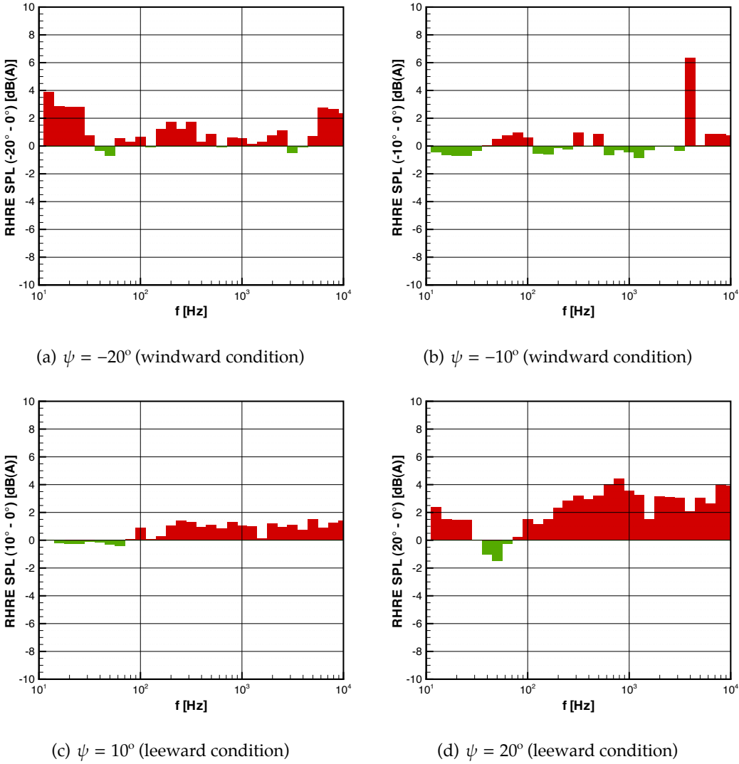
Figure 3.21: Steady AWT (Pininfarina) variation of RHRE cabin noise spectra at yaw (Geometry 2)
