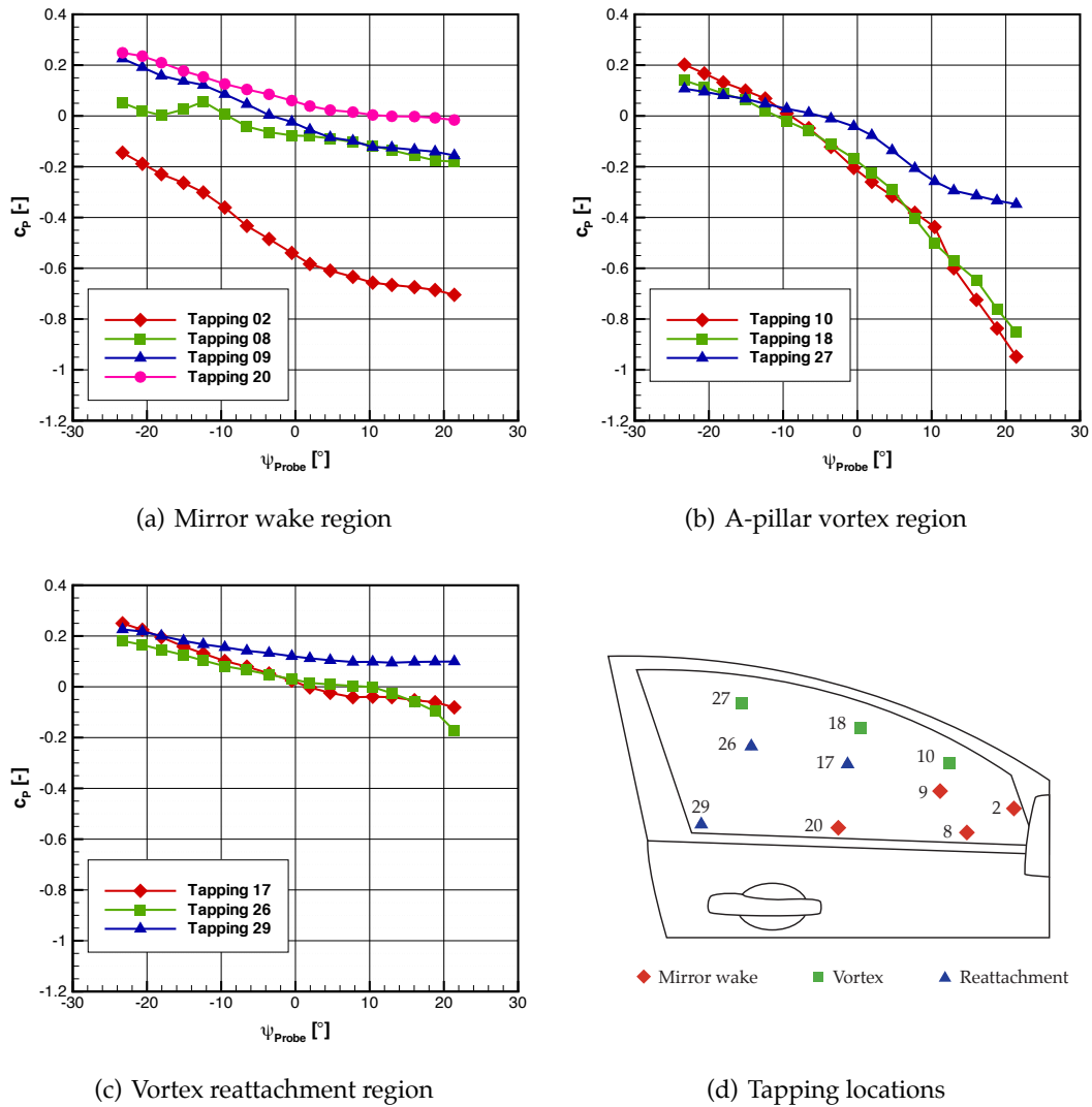
Figure 3.36: Steady AWT sideglass pressure characteristics (Geometry 1 SG)
