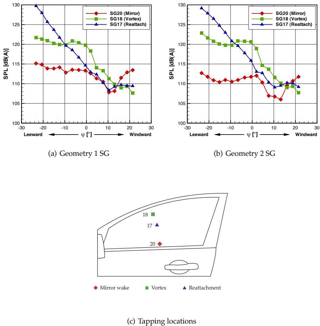
Figure 3.42: AWT (Pininfarina) sideglass surface noise characteristics
