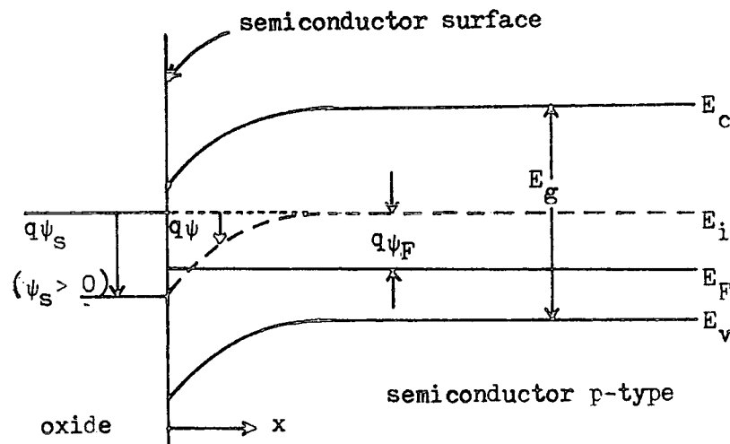
Fig 2.4 : Energy band diagram at the surface of a semiconductor. The potential \psi is measured with respect to the intrinsic Fermi level E_i (after Sze (31)).
