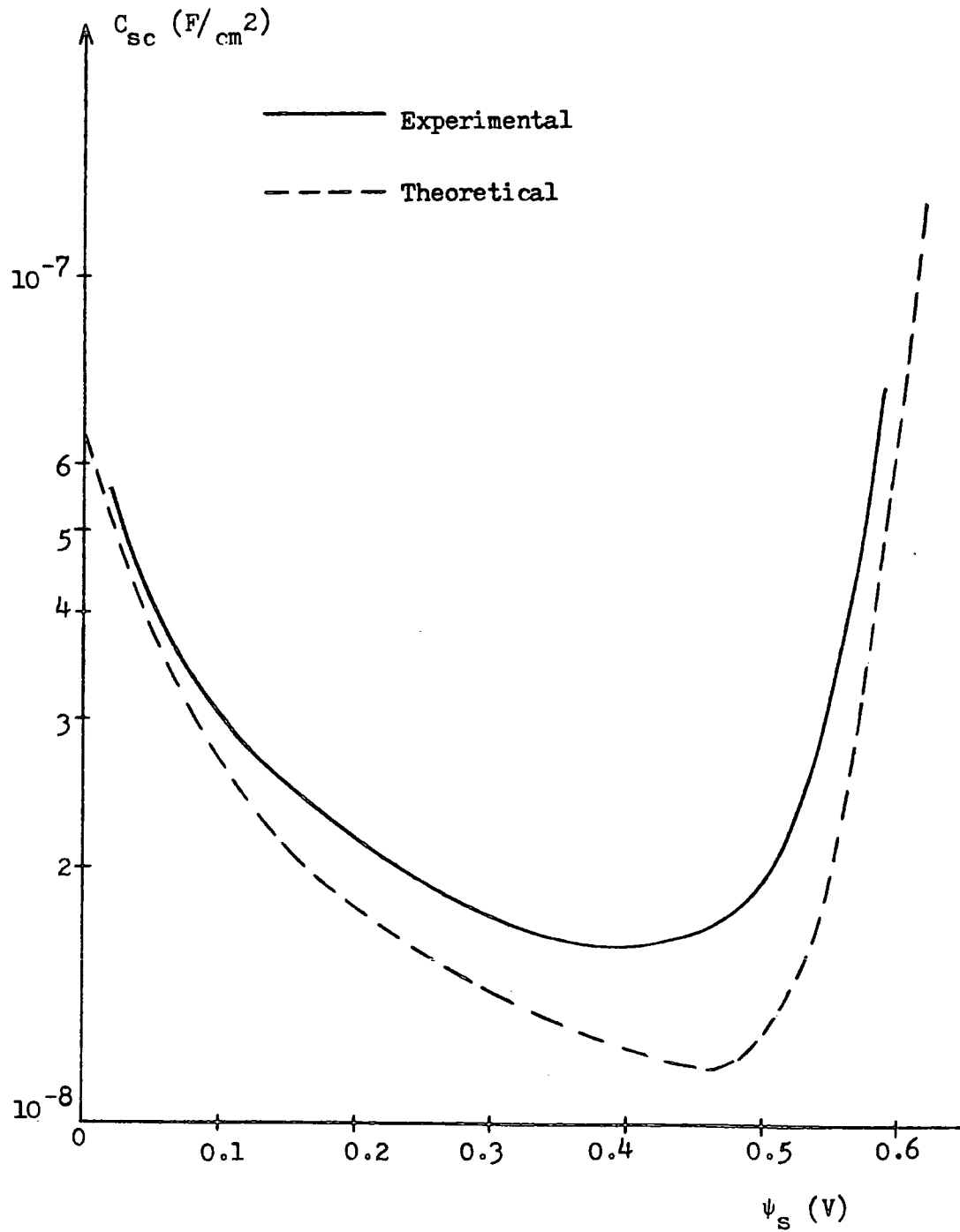
Fig 2.19 : Surface capacitance as a function of surface potential.
