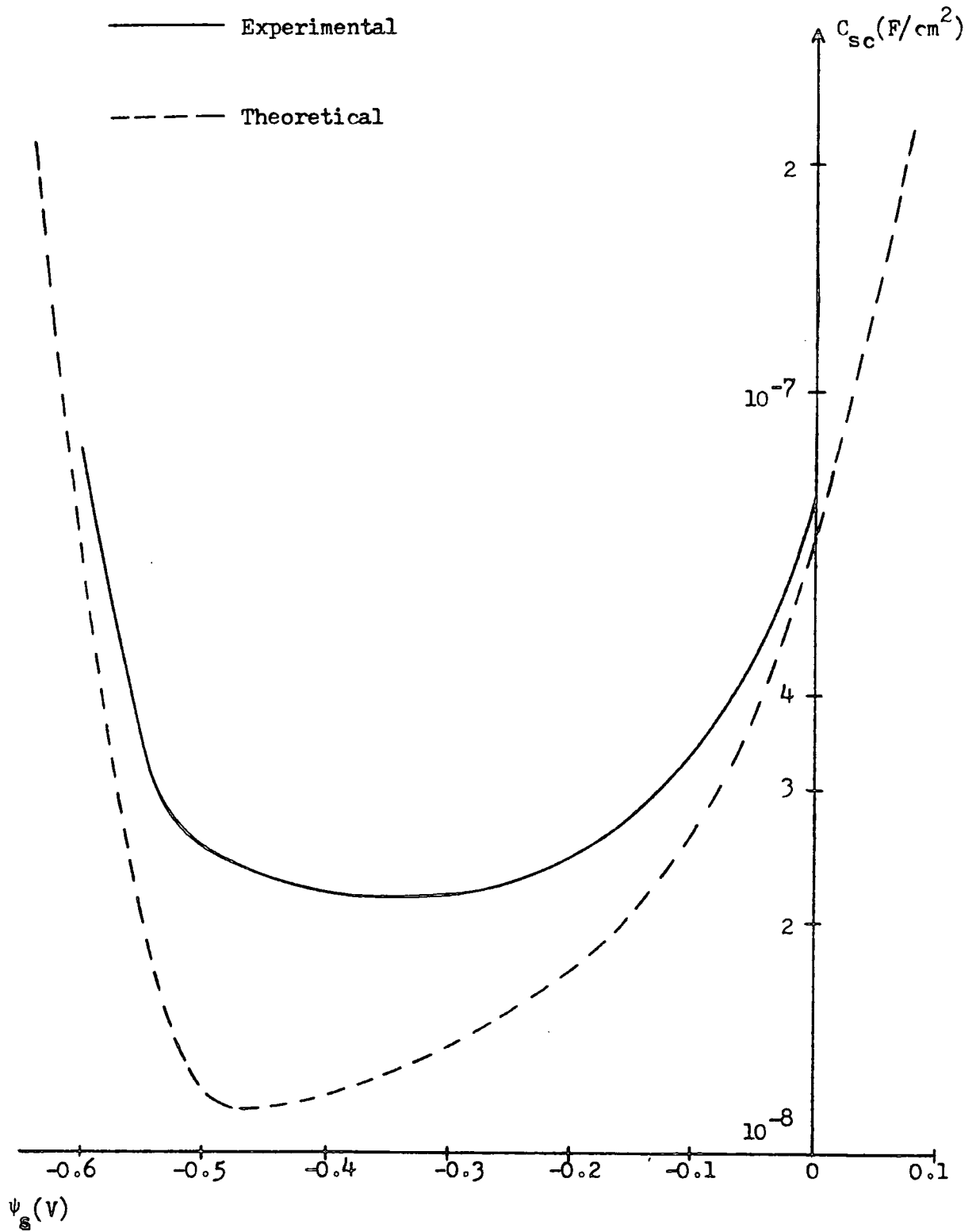
Fig 2.14 : Surface capacitance as a function of surface potential.
