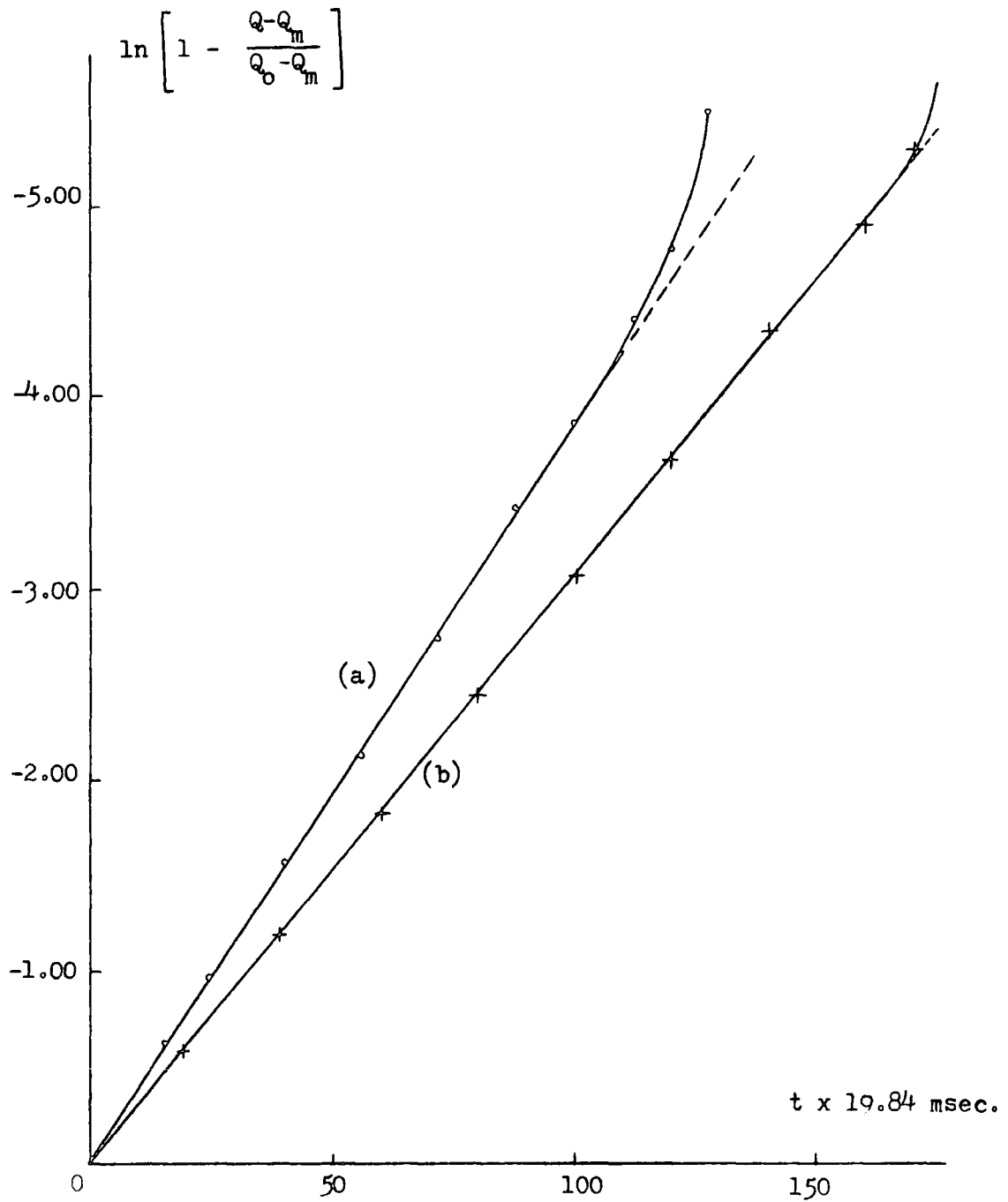
Fig 4.6 : Evaluation of charge-time plots
