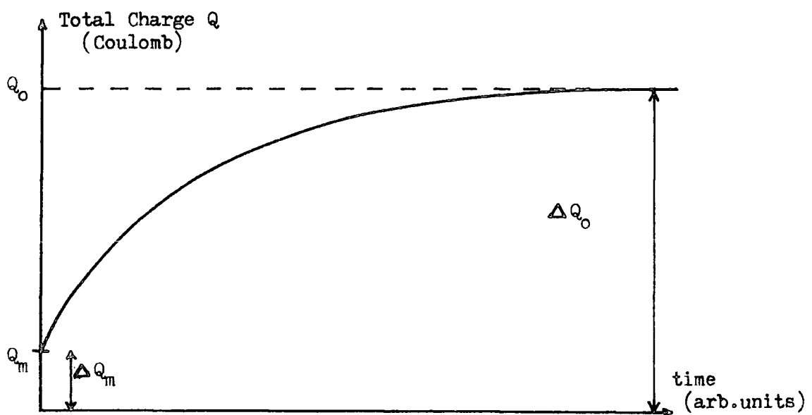
Fig. 4.3 : Schematic diagram of the transient characteristic of the total charge in an MOS capacitor after a small depleting voltage step.
