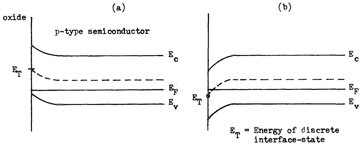
Fig 2.6 : Illustration of interface-states behaviour as surface potential is varied.
