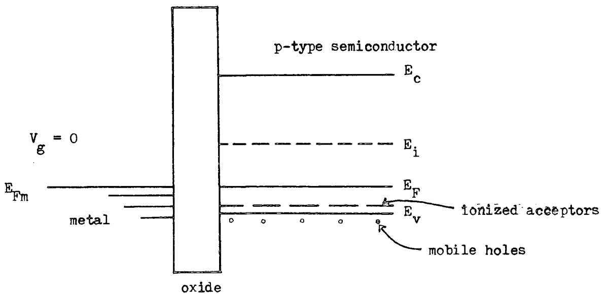
Fig. 2.2 : Ideal energy band diagram at V_g = 0 .
