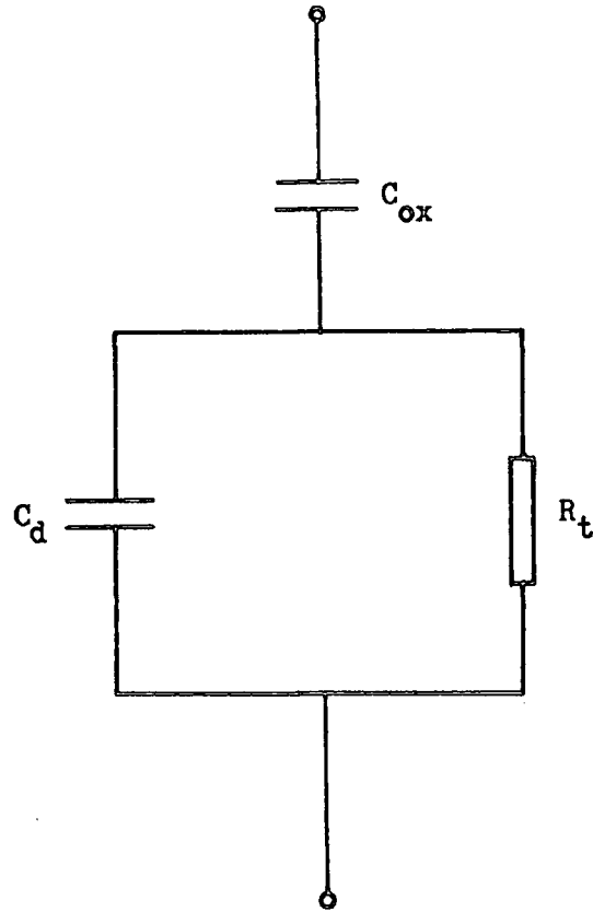
Fig 4.2 : Equivalent circuit of the MOS structure in strong inversion.
