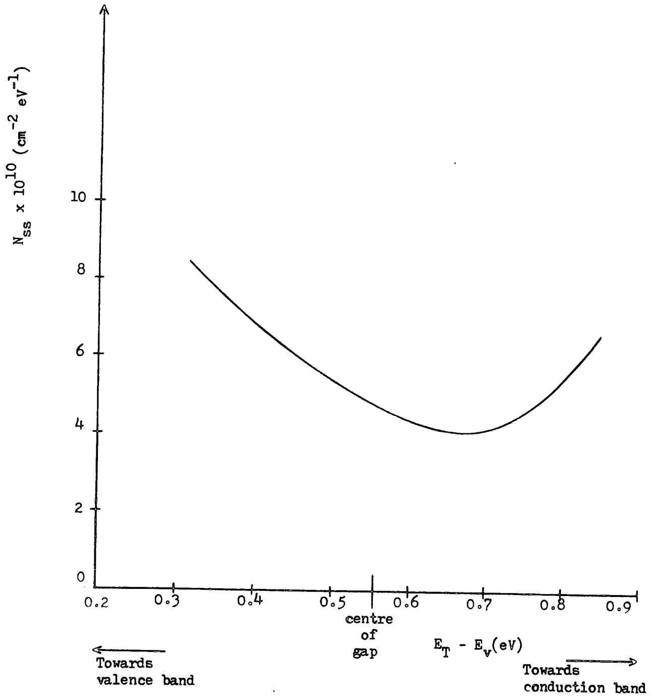
Fig 2.15 : Interface states density distribution obtained for n-type MOS capacitor.
