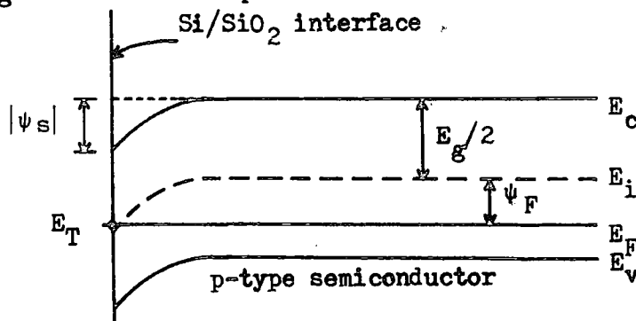
Fig 2.9 : Position of a single discrete interface-state level within the band gap as a function of surface potential.
