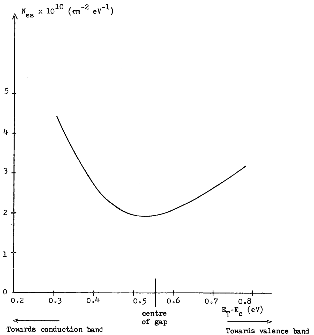
Fig 2.20 : Interface states density distribution obtained for p-type MOS capacitor.
