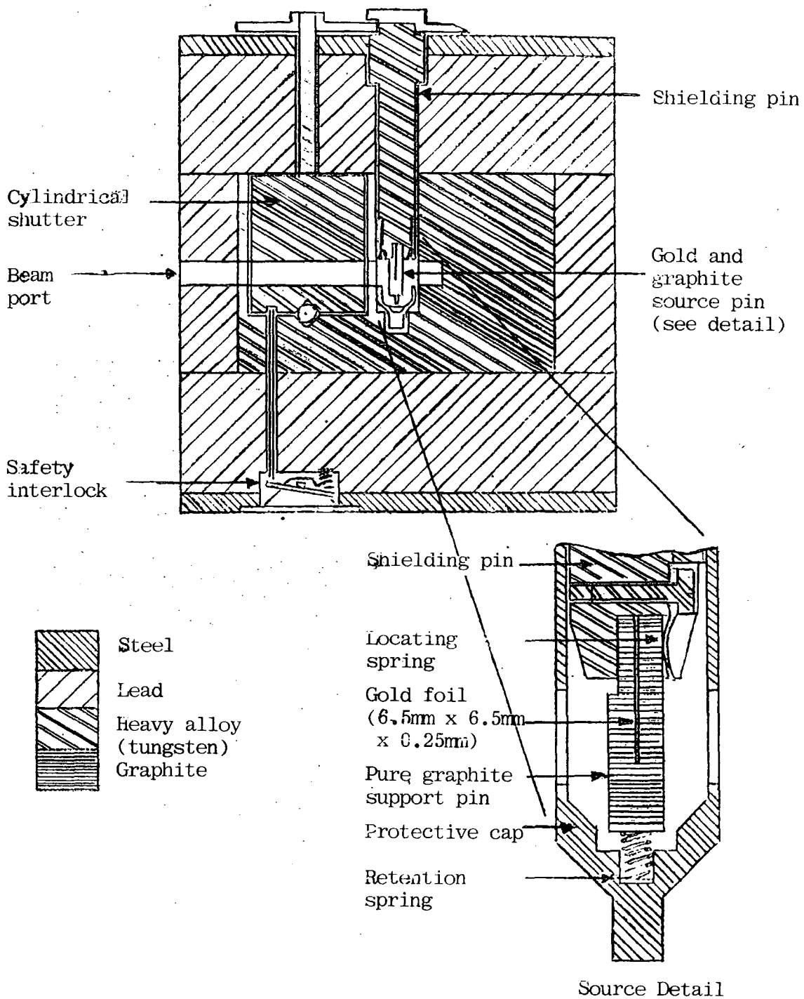
Fig. 6.2 The design of the container used to carry the gamma ray source.
