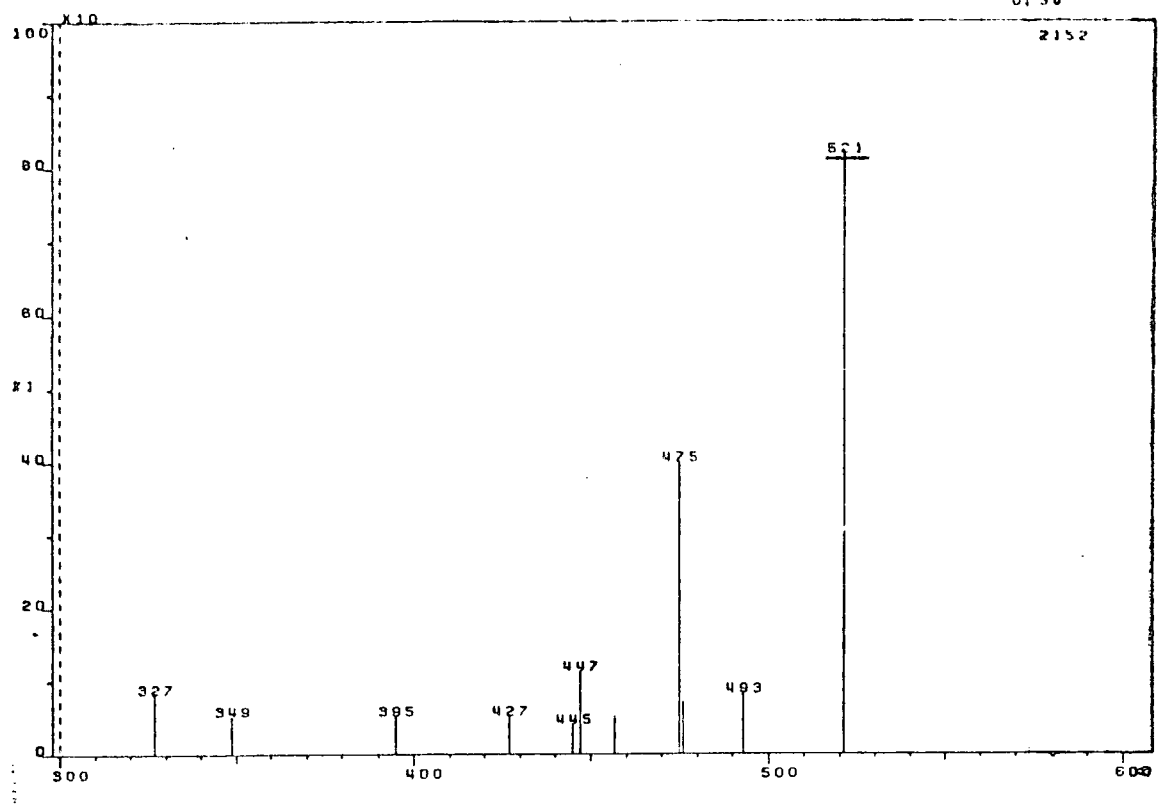
Compound No. 15 (MW 520) - Chemical Ionisation m.s.
