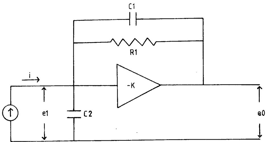
Figure 4.4.1 Electrical circuit for low current measurement.
