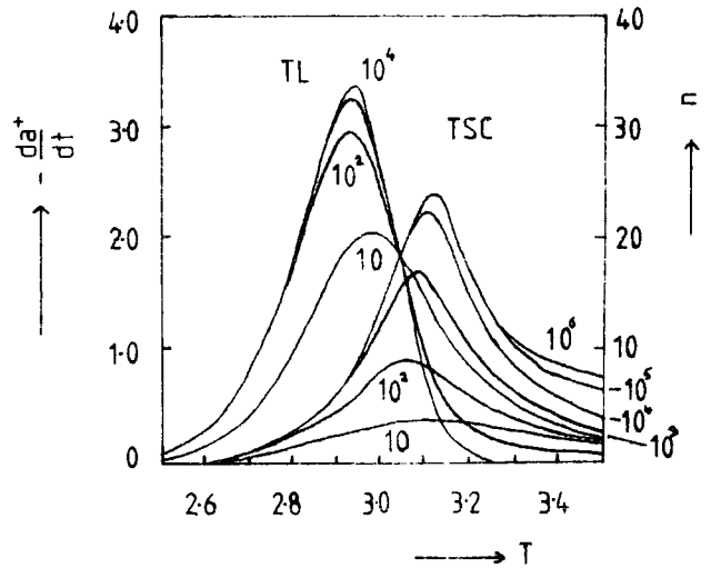
Figure 2.2.2 The influence of \alpha on TSL and TSC curves. E = 75 , s = 10^{12} , \delta = 0.01 , \xi = 10^{-6} .
