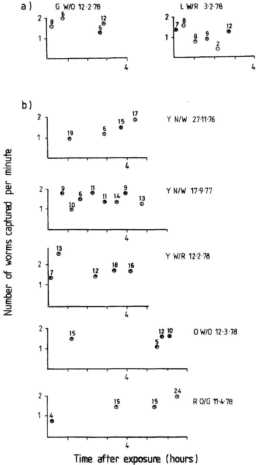
Figure 4.30 The rate of capture of worms in relation to time after exposure: a) two marked Curlews which showed a decrease, b) five which showed no decrease.
