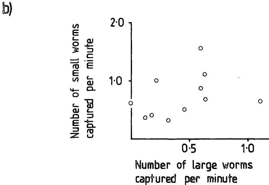
Figure 4.26 a) Rates of capture of large and small worms in relation to substrate temperature shown by one marked Grey Plover (L W/L) in one winter. These graphs are derived from the data presented in Figure 4.24. b) The relationship between the rates of capture of small and large worms taken by this marked Grey Plover.
