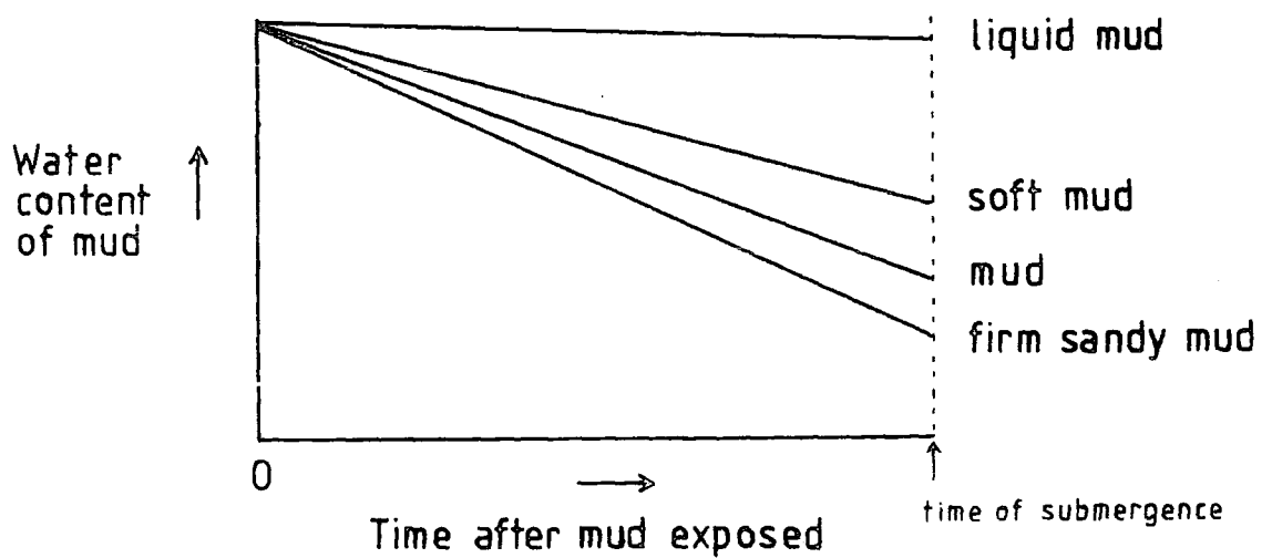
Figure 3.32 The rates of drying of four sediment types at the same tidal level.
