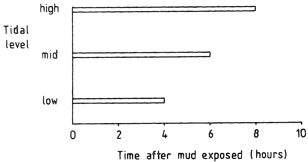
Figure 3.31 The approximate periods of exposure of mudflats at three tidal levels.
