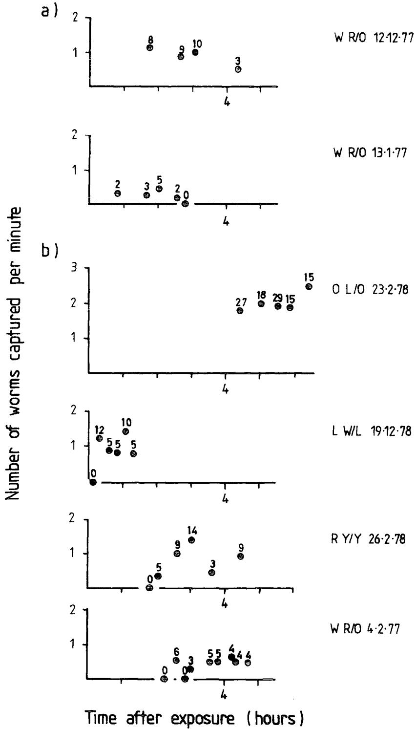
Figure 4.19 Changes in the rate of worm capture with time after exposure shown by thirteen marked Grey Plovers that fed in single sites throughout their periods of exposure; a) birds that showed a decrease, b) birds which showed no decrease.
