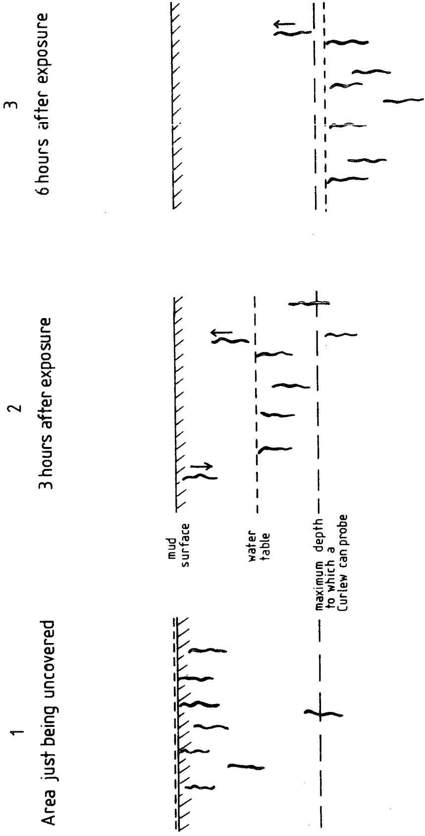
Figure 3.33 The depth distribution of Nereis worms at different stages of the tide. (Derived from information in Vader, 1964.)
