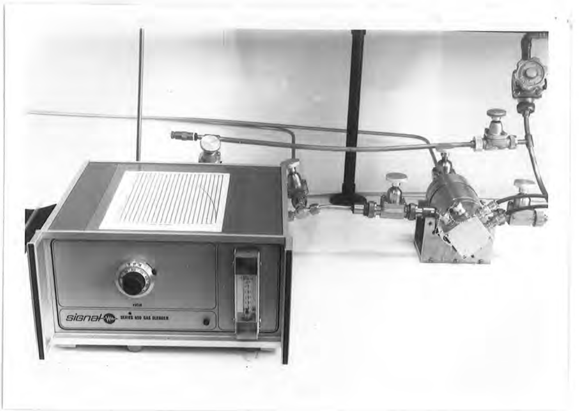
Figure 10. A photograph of the equipment used to measure the conductivity of the phthalocyanine films in the presence of various ambients.
