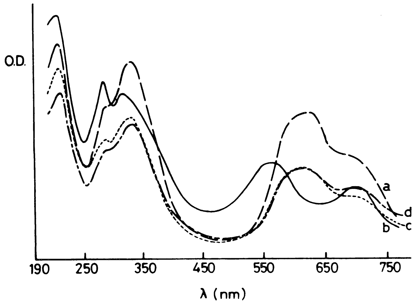
Figure 11. The effects of NOX on the electronic spectrum of a-phthalocyanine: a) before NOX, b) after NOX, c) the film heated to 150°C, d) the film further heated to 200°C (after Honeybourne and Ewen).
