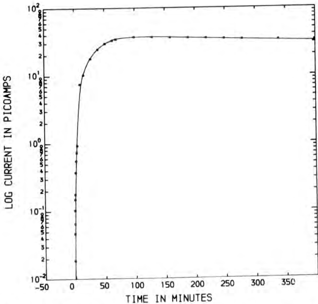
Figure 8. A typical result showing the rise in conduction due to placing a sample incorporating one layer of ASY-CuPc in a 20ppm ambient of NO 2 .
