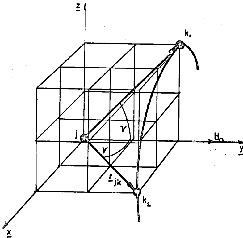
Figure 5.2 Illustrates how ions in symmetrically similar sites k_1, k_2 are identical with respect to ion j , when H_0 \parallel \langle 100 \rangle
