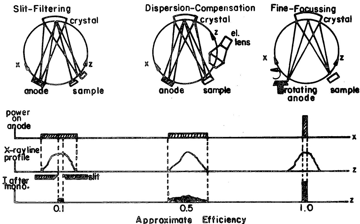
Figure Ten Diagram of alternative monochromatization systems employed for Al k\alpha monochromatization
