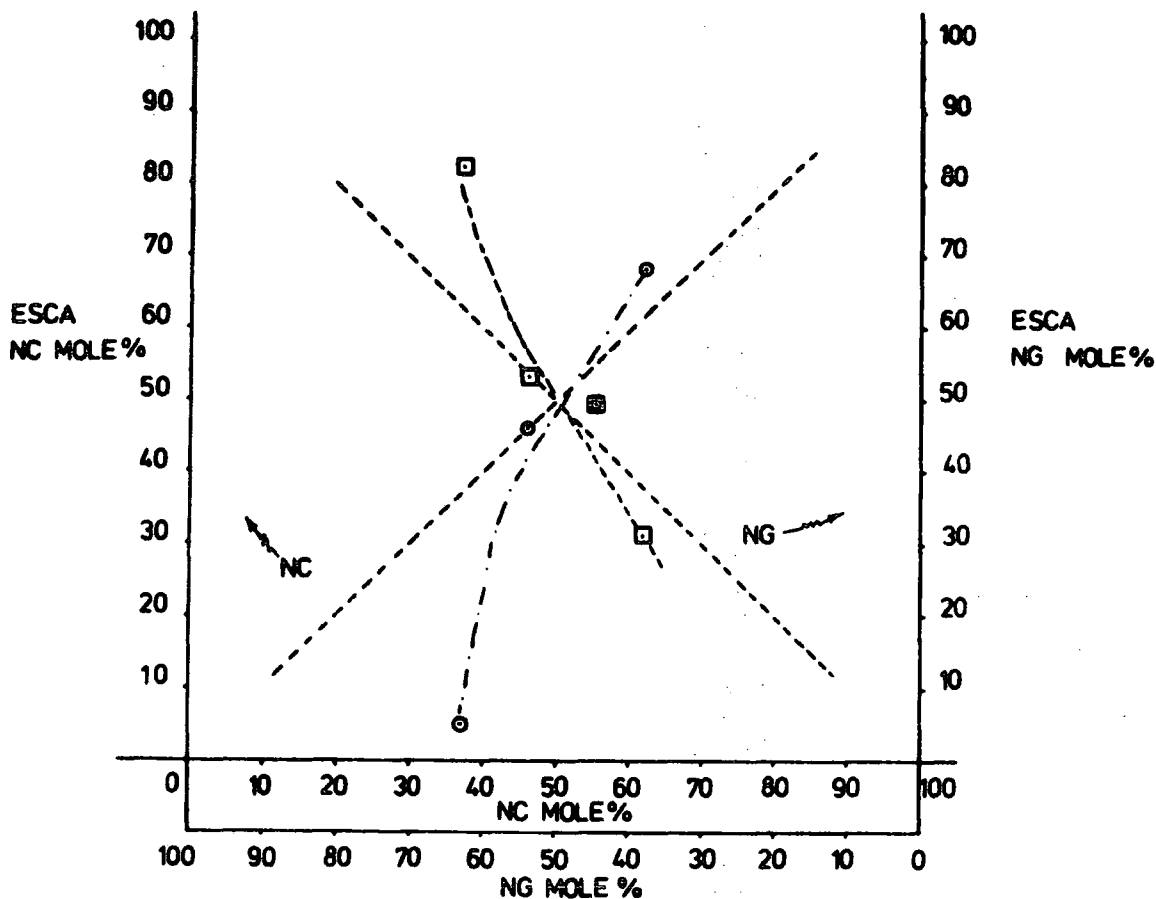
Fig. 44 Graph of Bulk mole % of NC/NG in double based propellants versus mole % NC/NG determined by E.S.C.A. (The dashed curves link the NC (O) and NG (□) data points whilst the dotted lines represent the correlations expected if surface and bulk are identical
