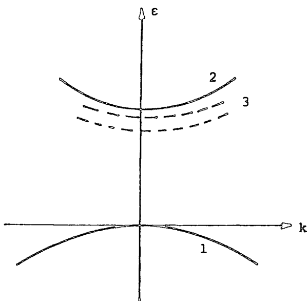
Fig 2.6 Exciton levels for a direct transition (1) valence band, (2) conduction band, and (3) exciton levels.
