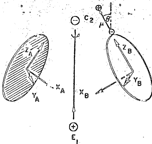
Fig 2.22 Conventions for axes, dipoles, and fields. Note that the dipole vector is positive along the direction from minus to plus. (45)
