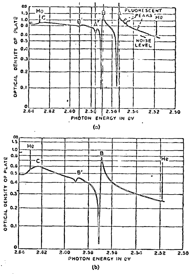
Fig 5.5 : Reflection of CdS at 4.2^{\circ} K for light polarized with (a) E_{\perp} and (b) E_{\parallel} to c. These are traces taken from microphotometer recordings of Kodak 103-O plates. The noise level is as indicated in Fig 2(a). The helium calibration lines indicate the resolution used. (14).
