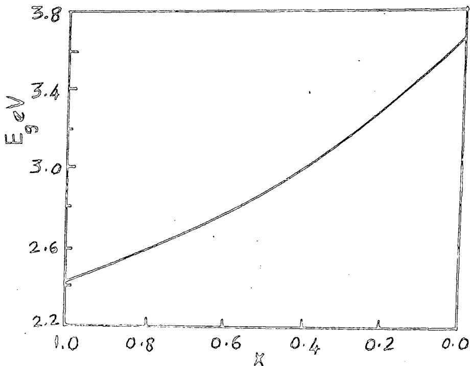
Fig 5.8: Variation of band gap, E_g , with composition in \text{Cd Zn}_x \text{S} crystal (12) .
