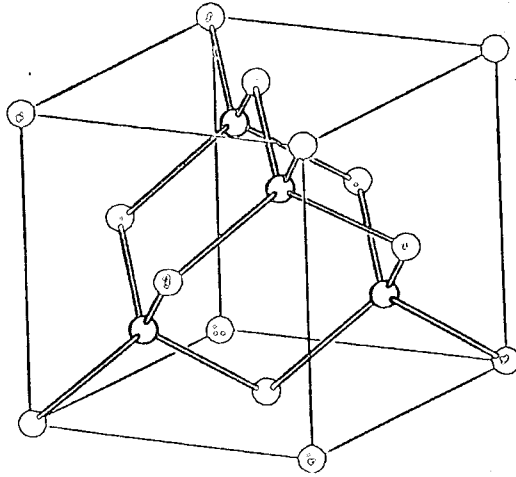
Fig 4.1: The two equivalent interpenetrating face centre cubic lattices of the zinc blende structure.
