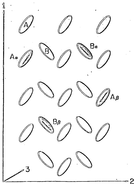
Fig 2.23 Orientation of molecules in a model molecular crystal. (45)
