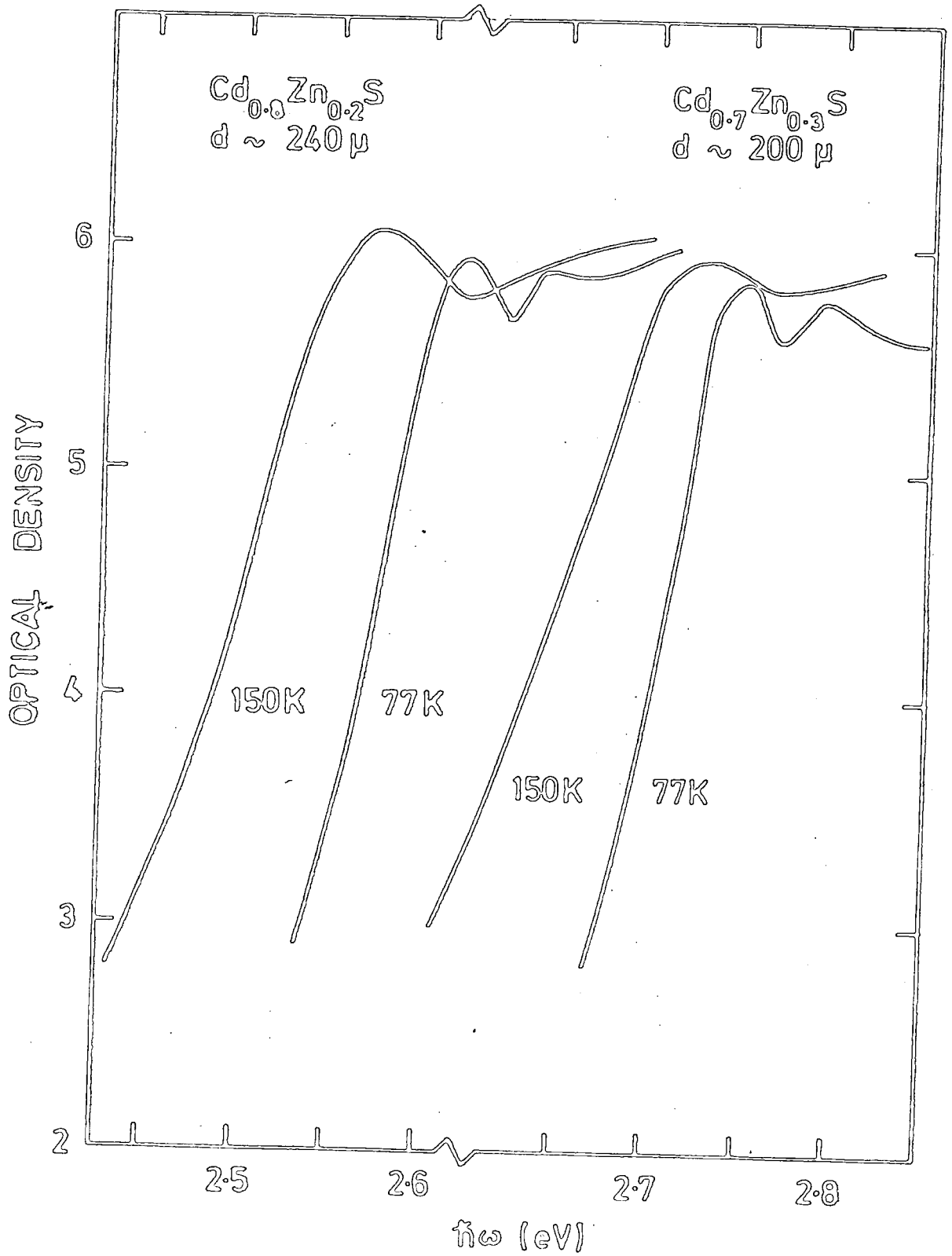
Fig 5.16 : Absorption edges of Cd 0.8 Zn 0.2 S and Cd 0.7 Zn 0.3 S samples.
