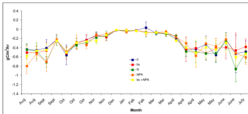
Figure 4.12 The seasonal variation in PP and insignificant affect of fertiliser, where 0: control; bs: basic slag; N: nitrogen; NPK: NPK; bs + NPK: basic slag and NPK; where symbols represent the mean and error bars represent the standard deviation
