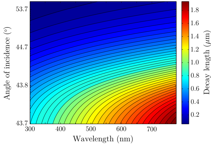
Figure 8.4: The decay length of the evanescent wave as a function of incident angle and wavelength, for n = 1.45 .
