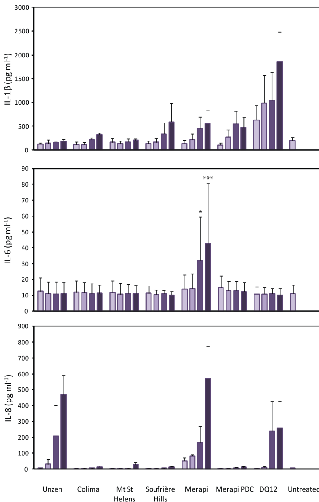
Figure 6.19: Production of proinflammatory markers IL-1β, IL-6 and IL-8 by differentiated THP-1 cells at 24 hours following treatment with volcanic ash. Data columns are treatment doses of 5, 10, 25 and 50 μg cm -3 *p<0.05, **p<0.01, ***p<0.001.
