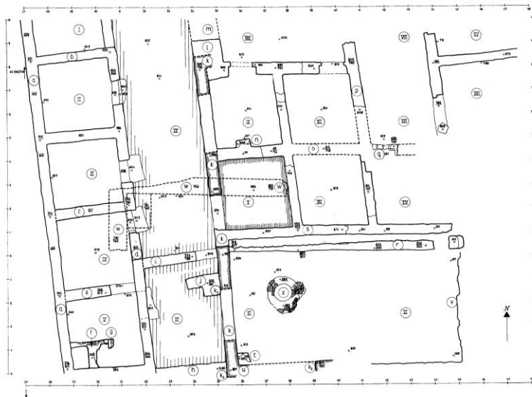
Fig. 67. Plan of the Islamic Town. The small rooms (I-V) facing a street (VII) suggest a suq. (VI) is a building later blocking the street. Area (XI) with well (x) may be an enclosed yard (public bath?), (f),(g),(w) are walls from an earlier Islamic building phase, (k) indicates four piers, and (r) is a secondary wall later than the pier-structure.
