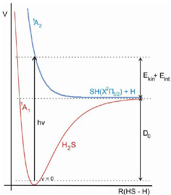
Figure 6.2: schematic diagram of the potential energy surfaces of H 2 S involved in the photodissociation process following excitation in the first absorption band.
