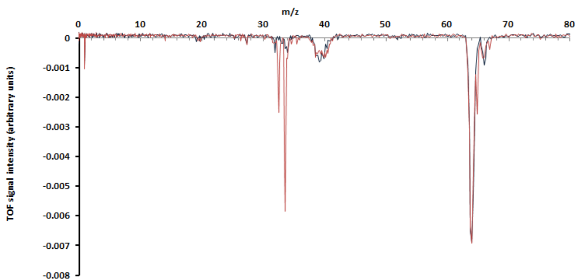
Figure 6.22: TOF spectra resulting from the action of the unfocussed photodissociation laser. The blue spectrum is the result of the action of the photodissociation laser only; the red is the result of the action of both the photodissociation and probe lasers.
