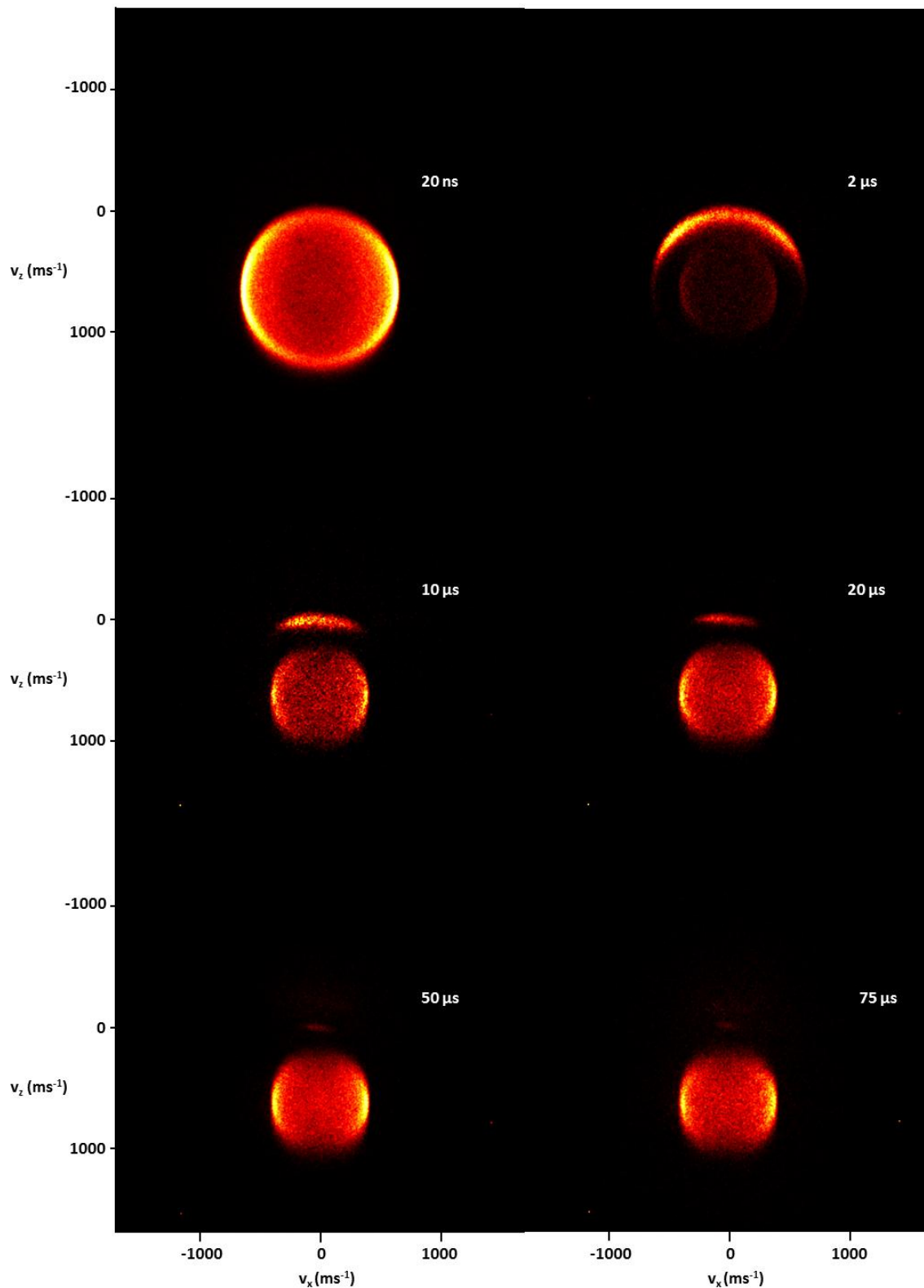
Figure 6.18: ion images of photostopped SH( X \ ^2\Pi_{3/2} ) at a series of photodissociation-probe intervals. The 100 \mu\text{s} image is not shown because the signal is very weak and cannot easily be seen. This figure is best viewed in the electronic copy of this thesis.
