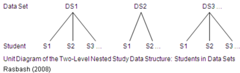
Figure 8: Two-level MLM study data structure
