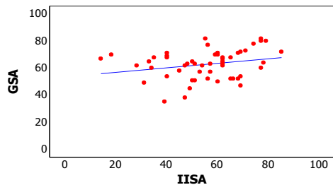
B6 GSA = 53.5 + 0.168 IND
