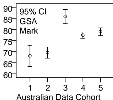
Figure 18: Data source A cohorts GSA marks means and confidence intervals
