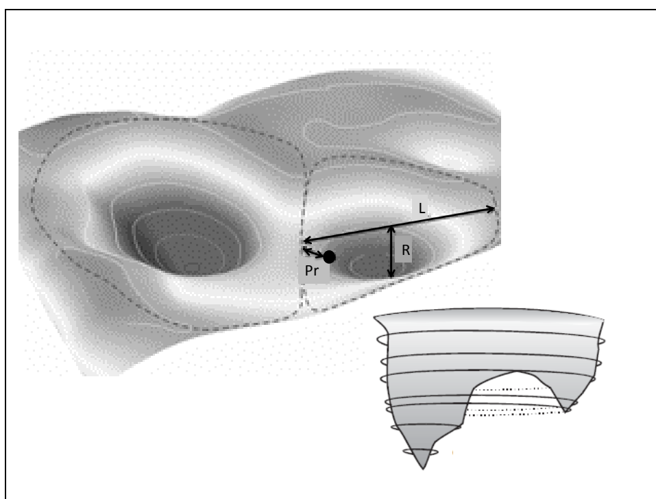
Figure 2.2: “Stability landscape,” top image adapted from Walker et al. 2004 with bottom image adapted from Gallopín 2006.
