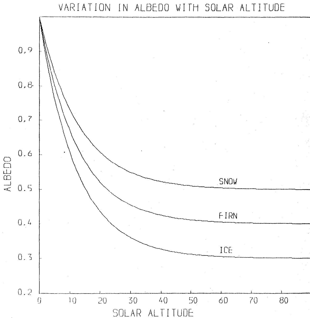
FIGURE 8.11 Variation of Glacial Material Albedo With Solar Altitude
