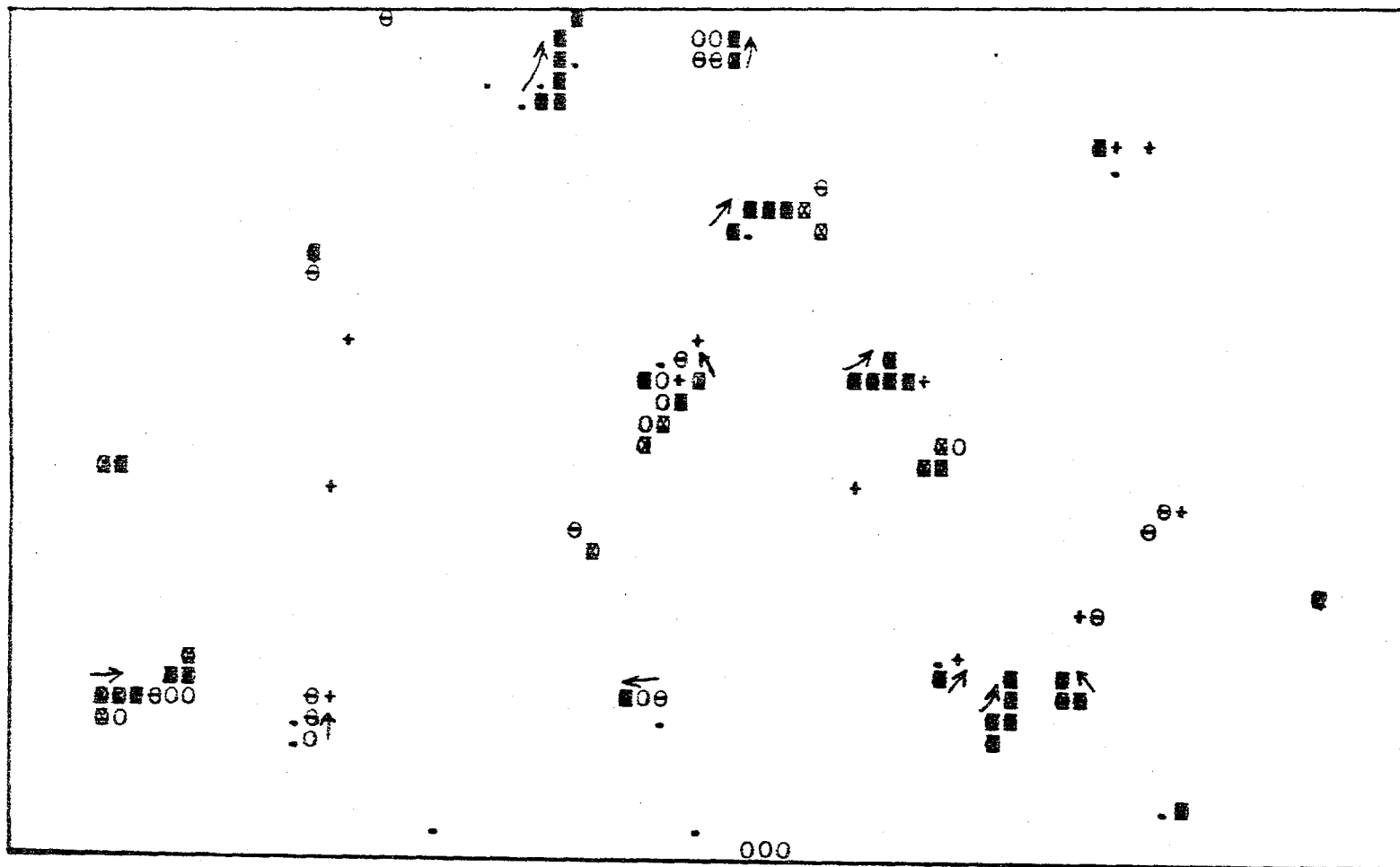
FIGURE 9.24 Central Nupur Glacier Balance Simulation (4° temperature drop)
