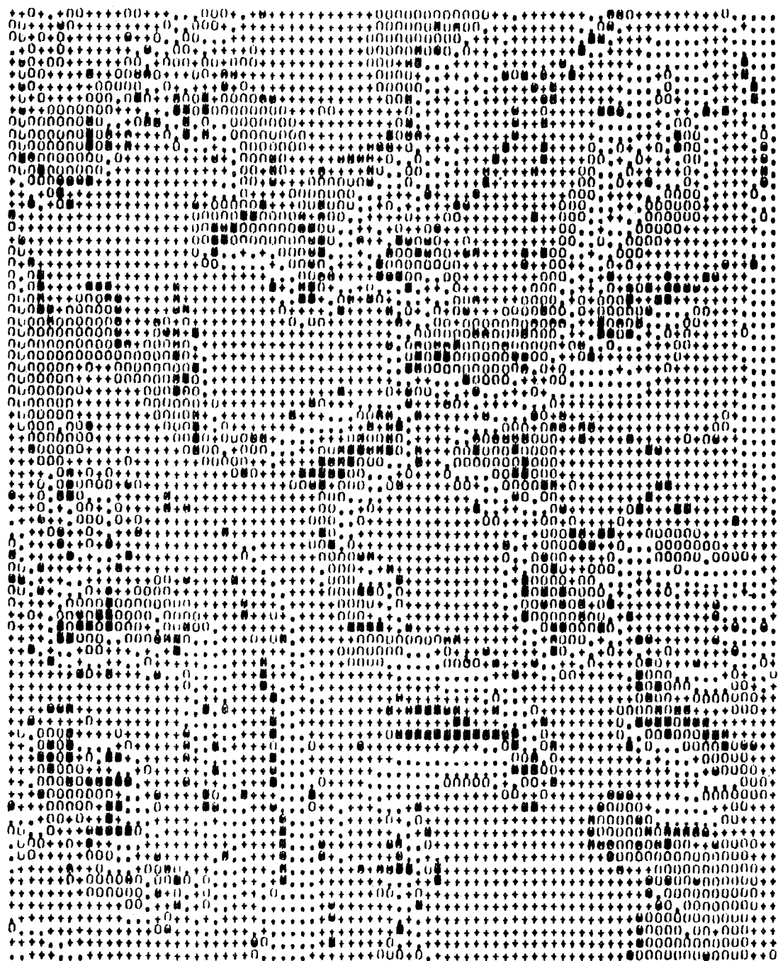
FIGURE 9.6 Nupur Mass Balance Simulation (1931-60): March (A=6)
