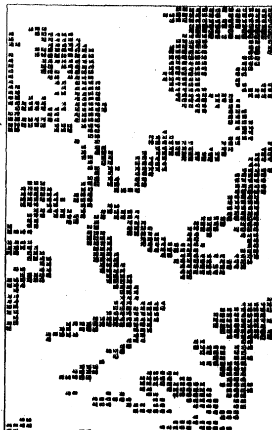
FIGURE 7.7 Distribution of the Grid-Points Over the Central Nupur-Matrix which Satisfy Conditions 2, 3, 6 and 7 for the Determination of Snow Density (see Table 7.3).
