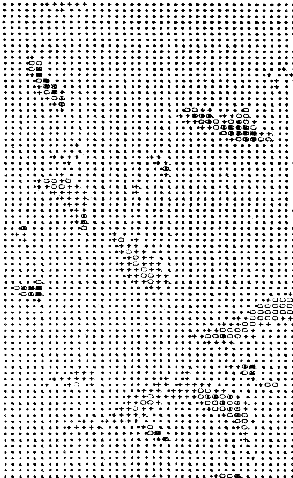
FIGURE 8.7 Percentage Reduction of Shortwave Radiation Receipt (for July) as a Result of Topographic Shading Over the Central Nupur Matrix.
