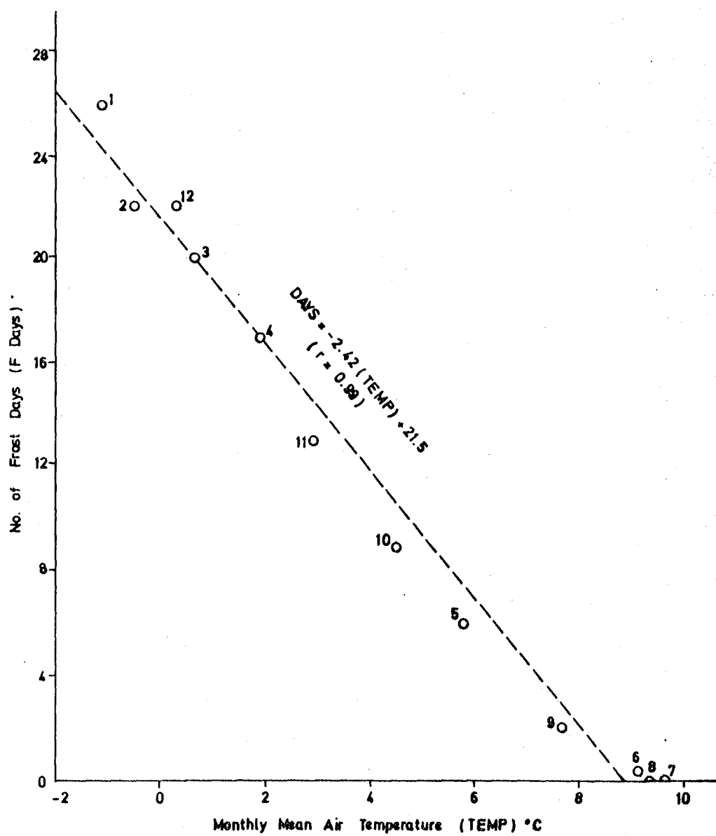
FIGURE 8.4 Number of Frost Days as a Function of the Monthly Mean Air Temperature at Sudureyri (mean of 1951-1960). Source: Icelandic Meteorological Office.
