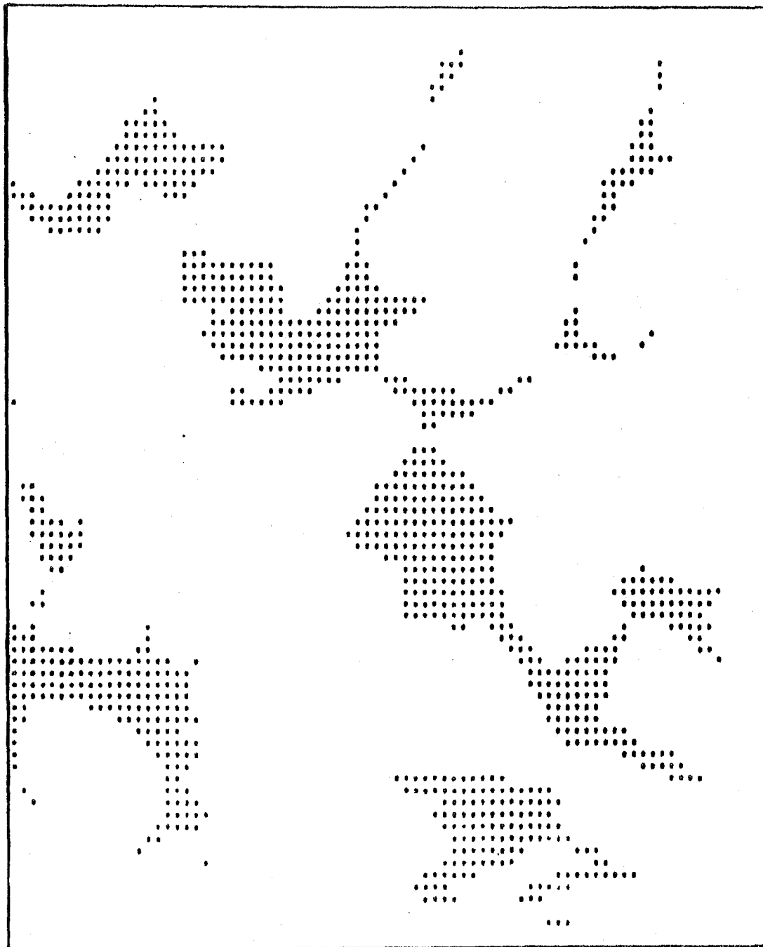
FIGURE 9.1 Nupur Mass Balance Simulation (1931-60): October (A=1)
