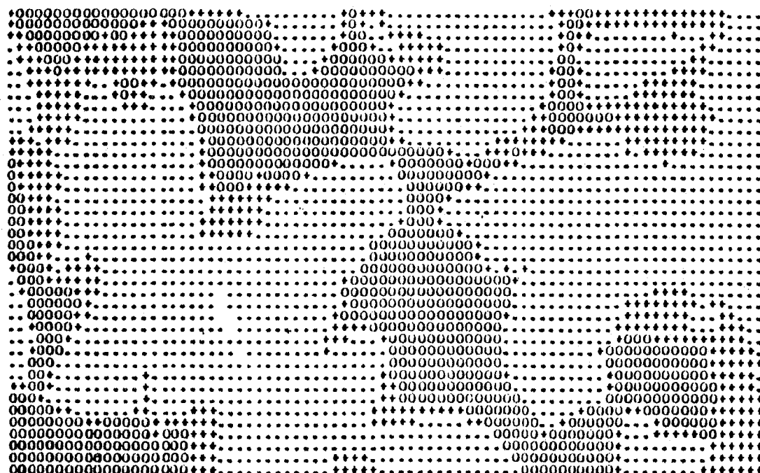
FIGURE 6.15 January and July Wind Speeds Over the Central Nupur Matrix as Determined by the Subroutine MWIND.
