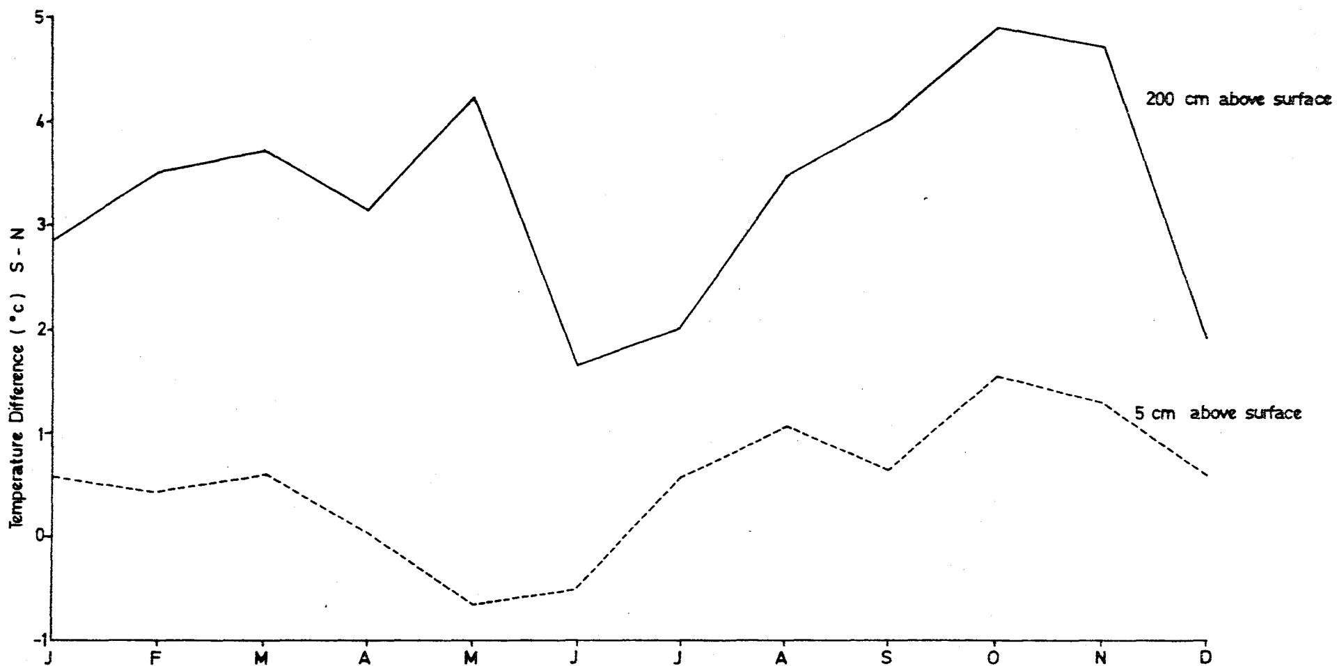
FIGURE 6.3 Seasonal Variation of the Temperature Difference (°C) between South and North Slopes on the Cushtunk Mountain, New Jersey. Data provided by Cantlon (1953 p.248).
