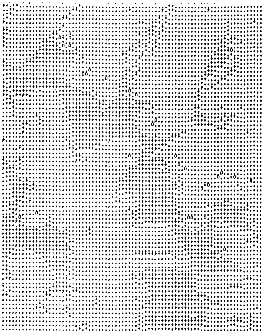
FIGURE 9.3 Nupur Mass Balance Simulation (1931-60): December (A=3)
