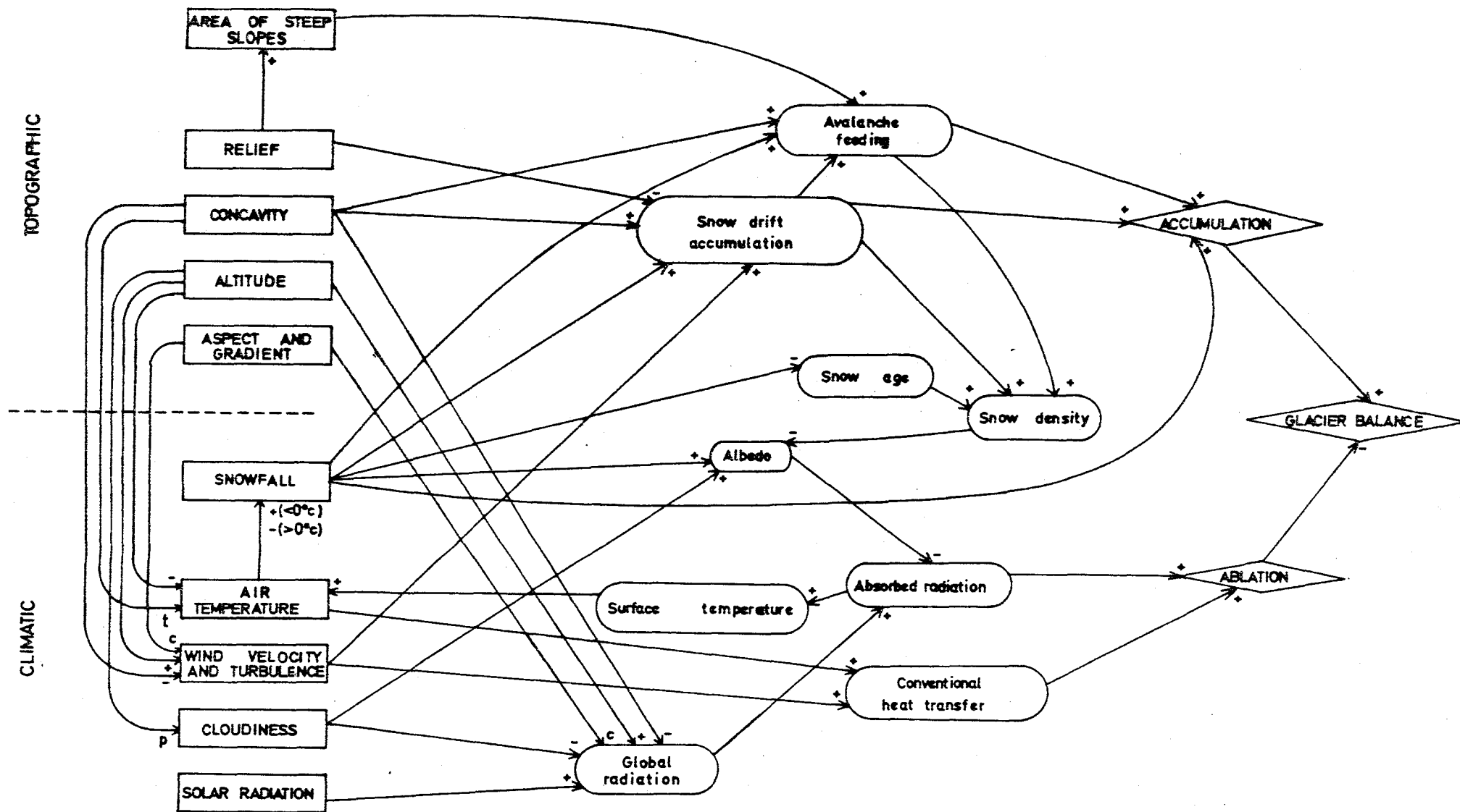
FIGURE 3.11 Interaction of Factors Affecting Glacier Mass Balance (modified after Evans, 1974 p.67)
