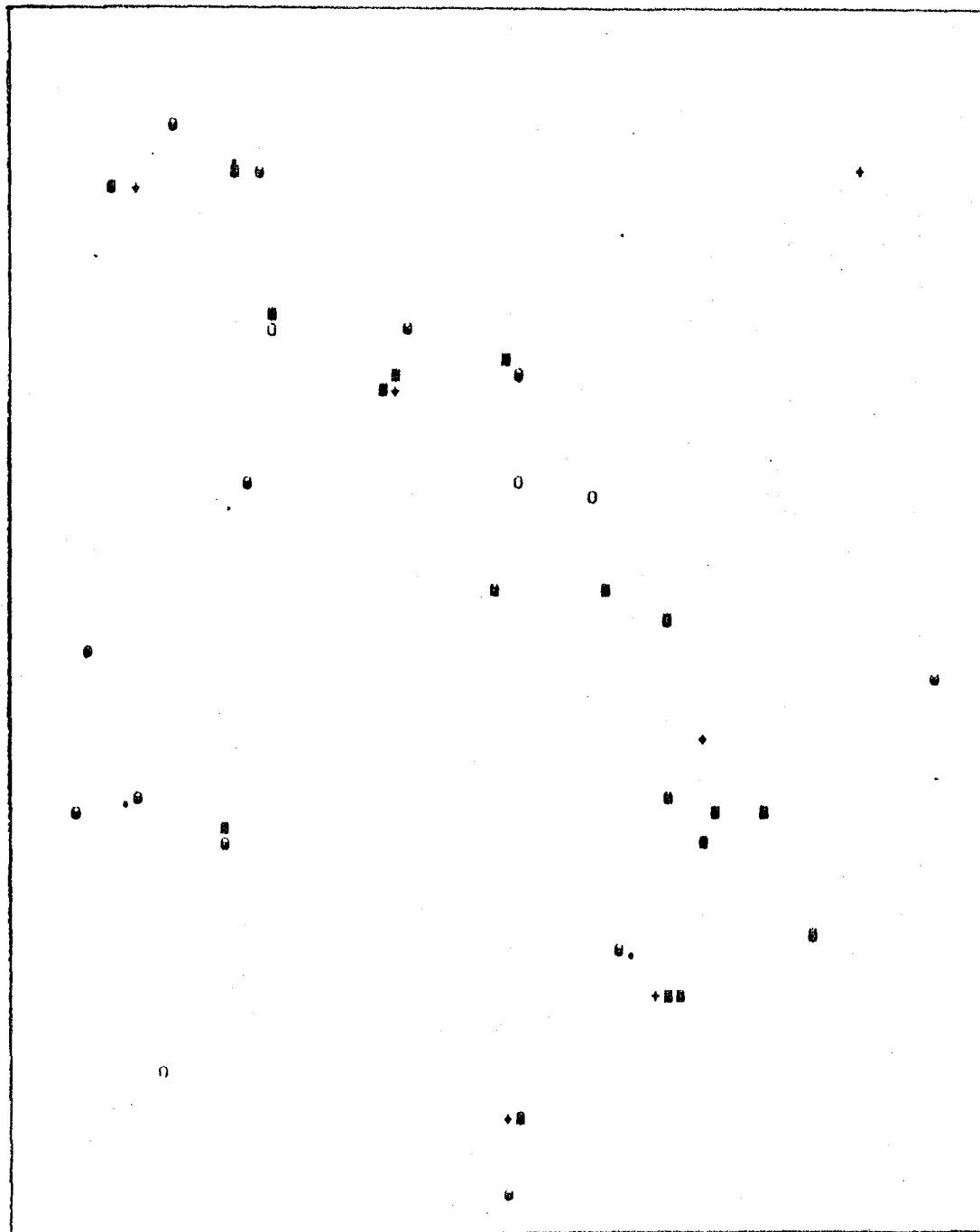
FIGURE 9.10 Nupur Mass Balance Simulation (1931-60): July (A=10)
