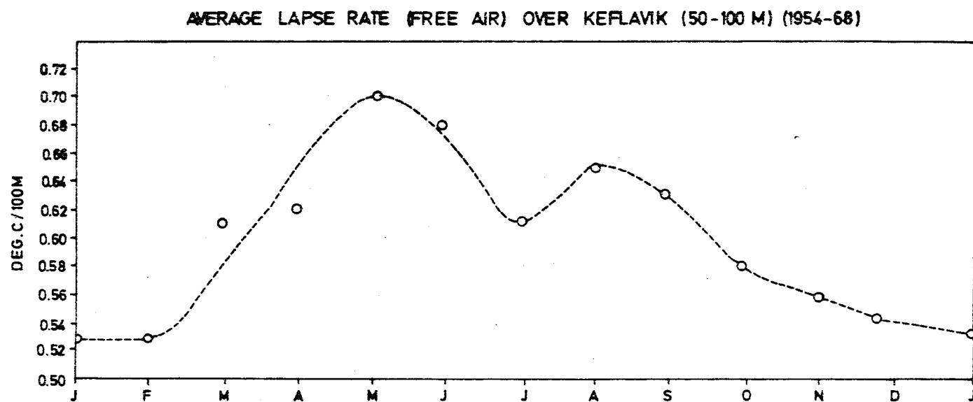
FIGURE 6.2 Variation of Monthly Lapse Rate (Free Air) Over Keflavik, Iceland. Source: Eythórsson and Sigtryggsson (1971 p.16).
