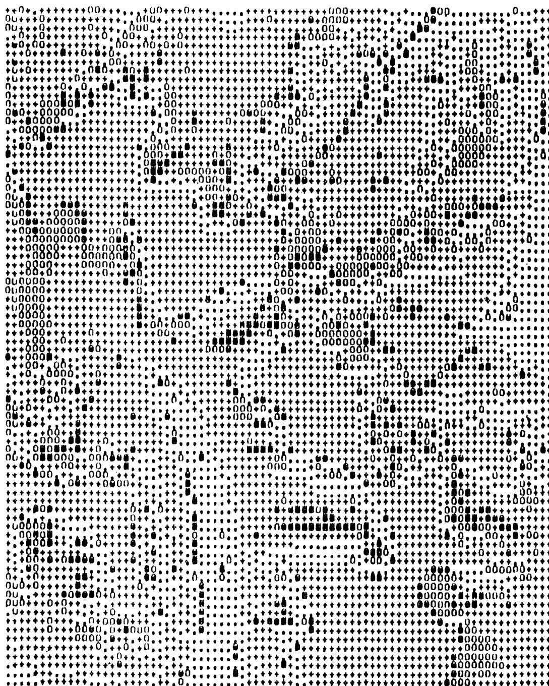
FIGURE 9.5 Nupur Mass Balance Simulation (1931-60): February (A=5)
