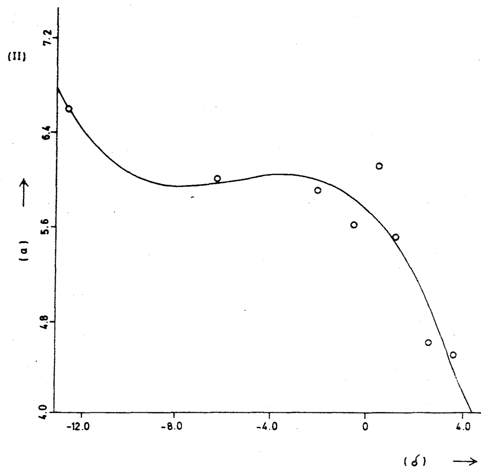
FIGURE 6.10 Relationship Between Coefficients a and b to \delta . Data from Bogdanova (1976). See text for explanation.
