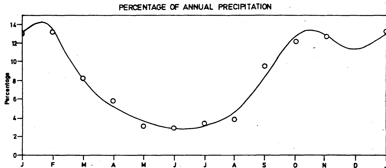
FIGURE 6.9 Mean Monthly Contribution to the Annual Precipitation at Thorustadir. Source: Icelandic Meteorological Office.
