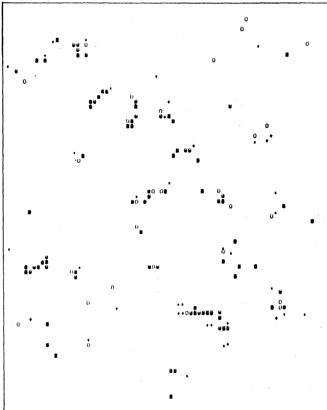
FIGURE 9.9 Nupur Mass Balance Simulation (1931-60): June (A=9)
