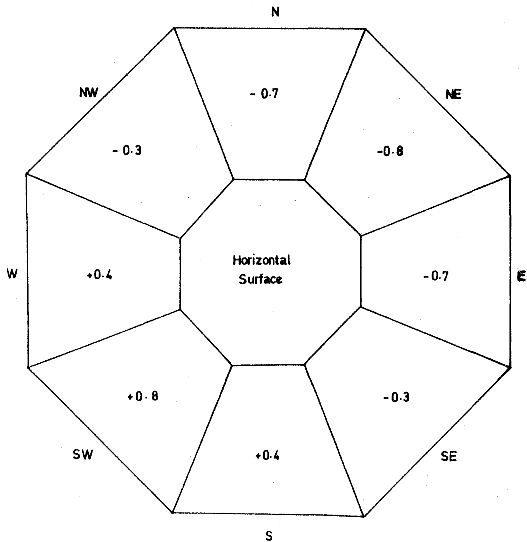
FIGURE 6.4 Modification of Mean Monthly Air Temperature ( ^{\circ}\text{C} ) Due to Slope Aspect as Suggested by Wymore (1974) for Use in the Piceance Watershed, Colorado.
