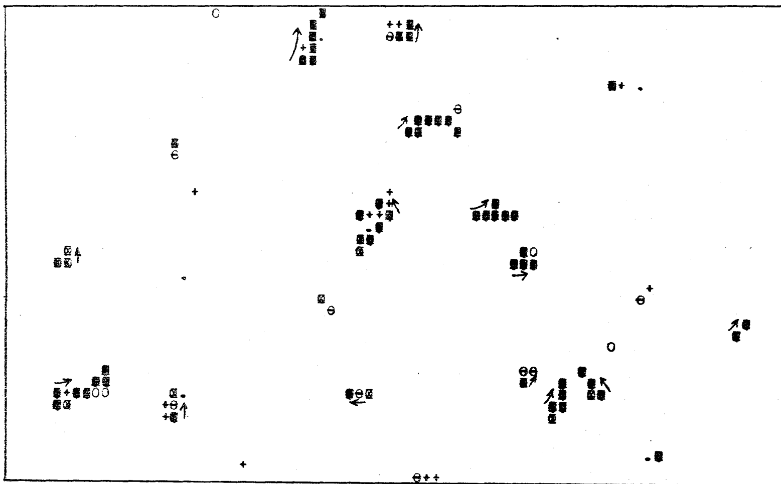
FIGURE 9.25 Central Nupur Glacier Balance Simulation ( 2^{\circ} temperature drop + 50% precipitation increase)
