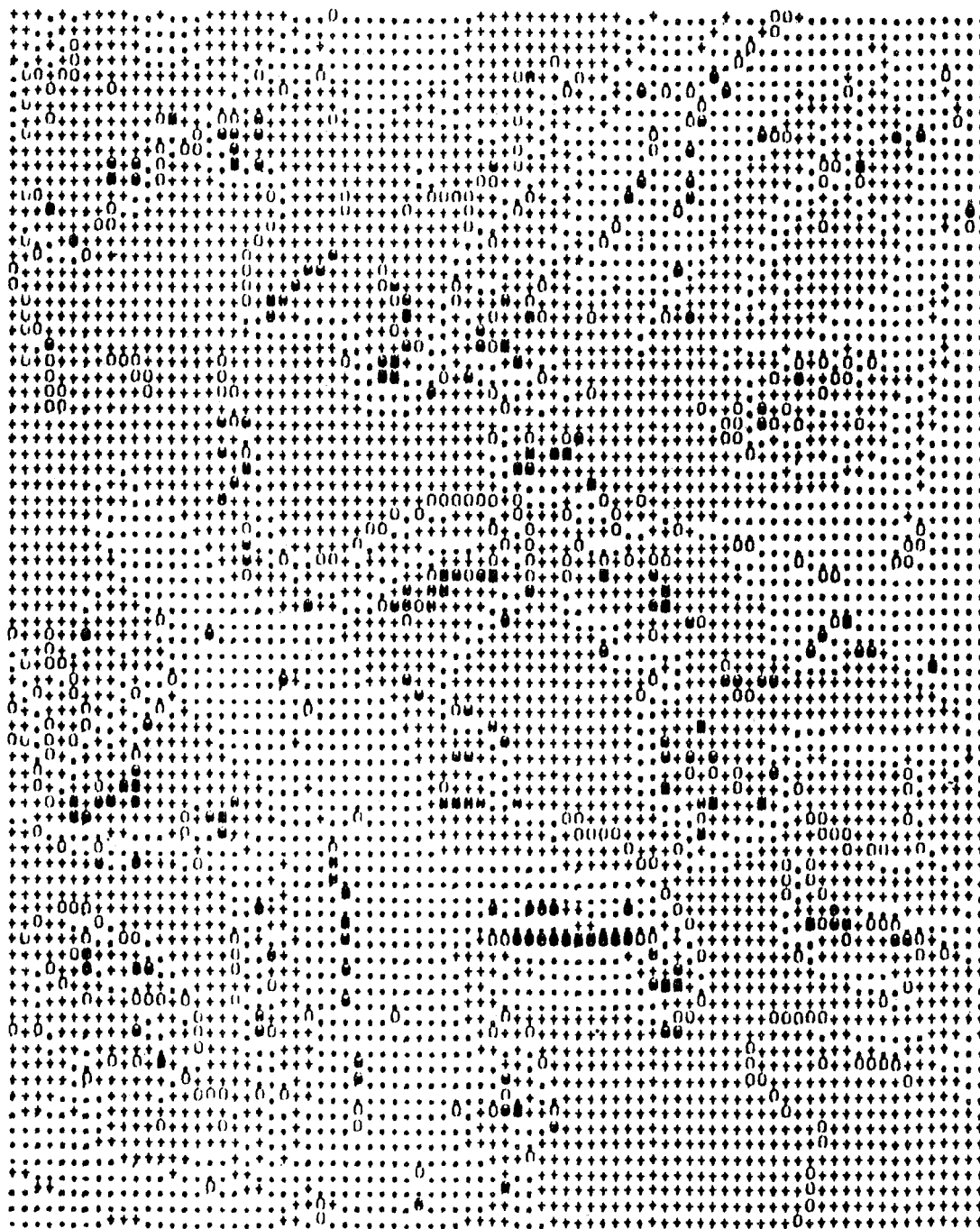
FIGURE 9.4 Nupur Mass Balance Simulation (1931-60): January (A=4)
