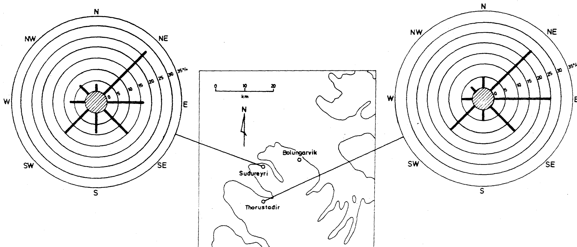
FIGURE 6.13 Frequency of Winter (Nov-Apr) Wind Direction (1931-60) in N.W. Vestfirðir. Source: Vetrattan: Icelandic Meteorological Office.
