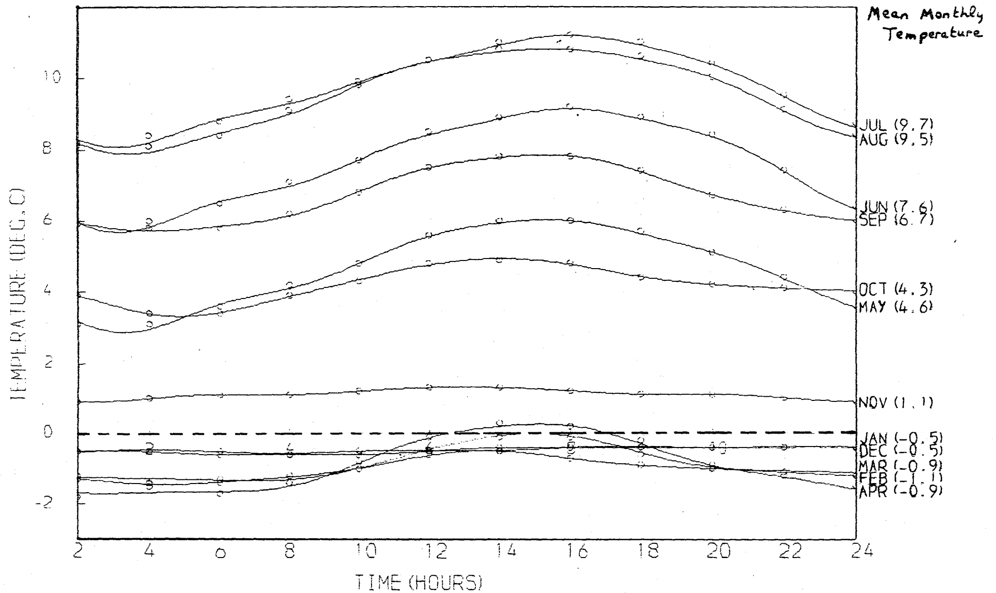
FIGURE 8.2 Diurnal Variation of Temperature at Bolungarvik (1946-1953) Source: Vetrattan. Icelandic Meteorological Office.
