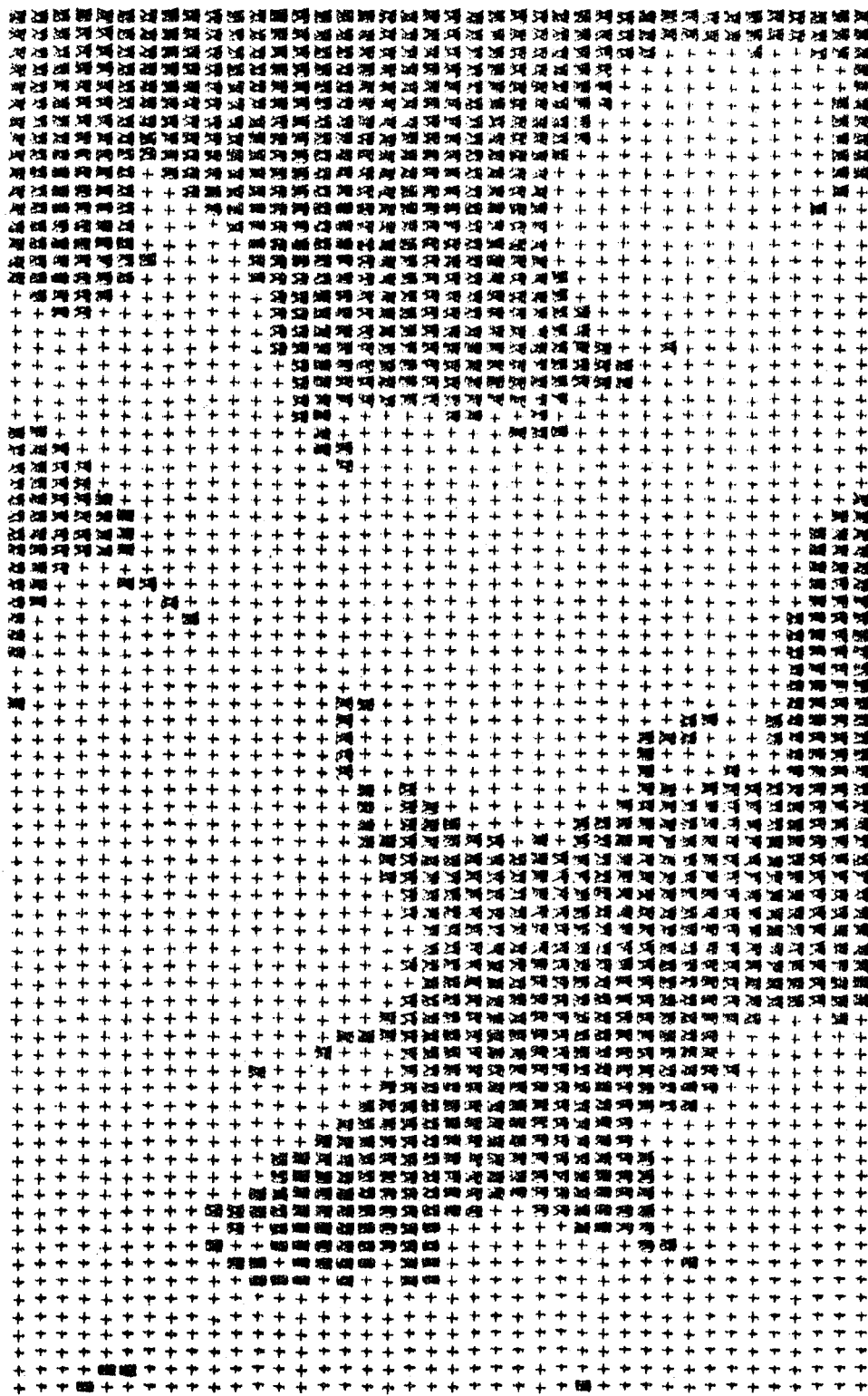
FIGURE 8.5 Distribution of Potential Melt Areas Over the Central Nupur Matrix (for April)
