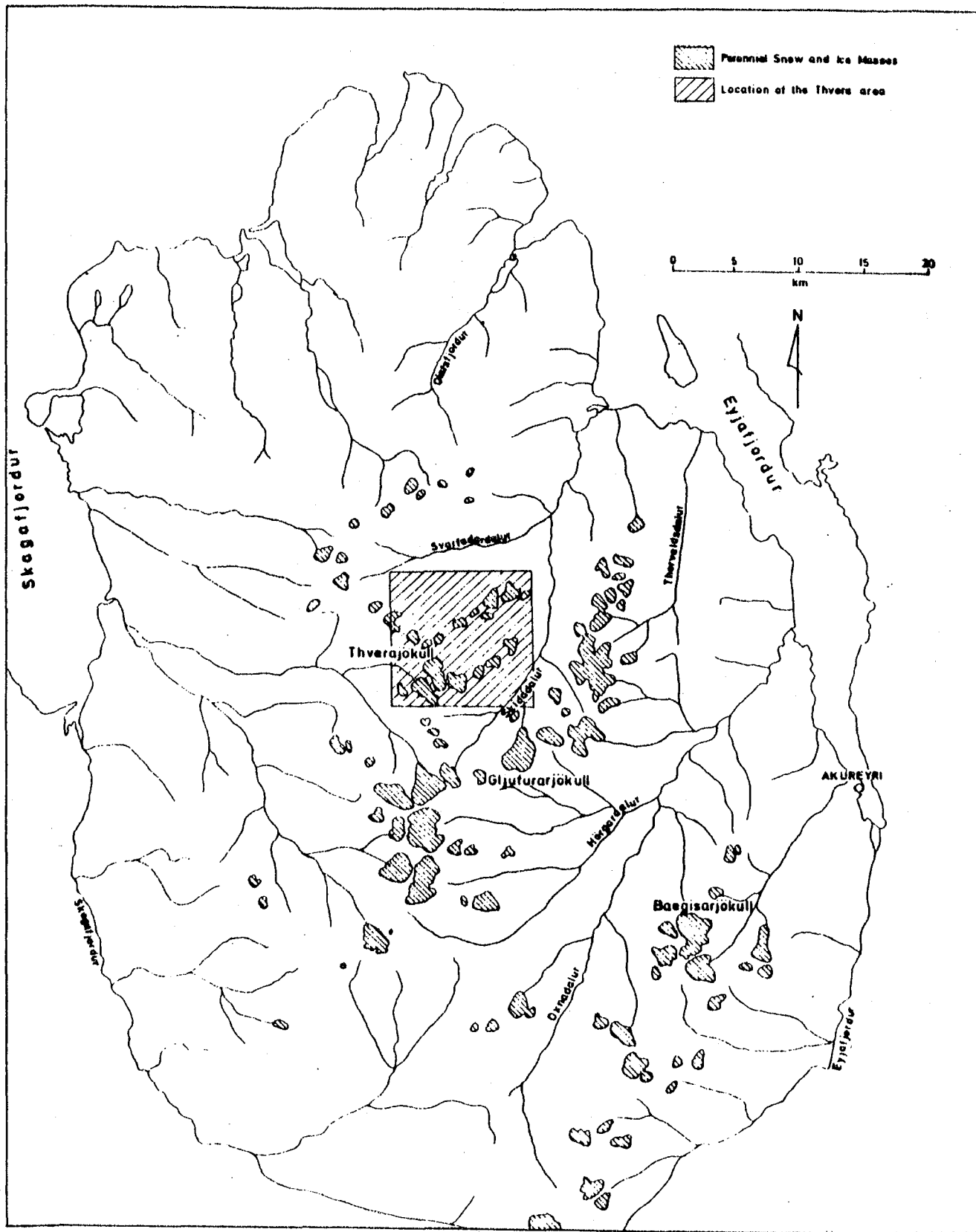
FIGURE 3.9 Local Glaciers of Tröllaskagi,
