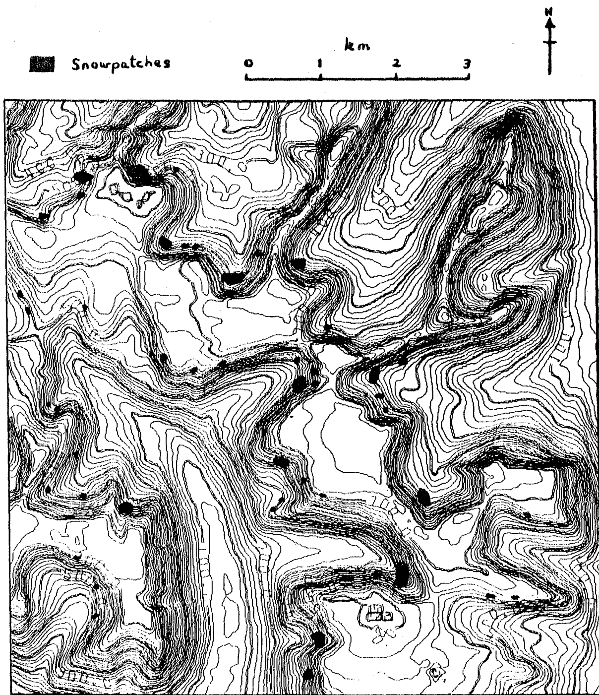
FIGURE 3.6 Snowpatch Distribution in the Nupur Area (August 1978).
