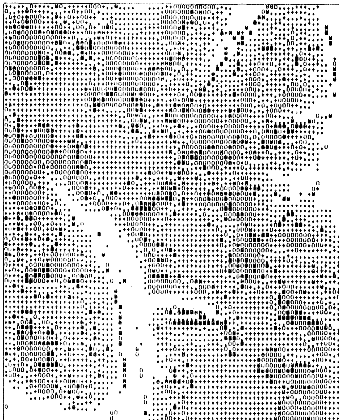
FIGURE 9.7 Nupur Mass Balance Simulation (1931-60): April (A=7)
