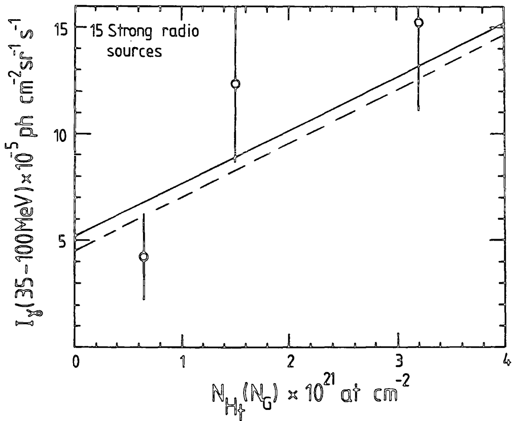
FIGURE 7.2 SAS II intensities I_\gamma(35-100 \text{ MeV})(\pm 1\sigma) versus N_{H_T}(N_G) for the radio source positions. The solid lines are the fits to the mean backgrounds. The excess intensities are given by the broken lines.
