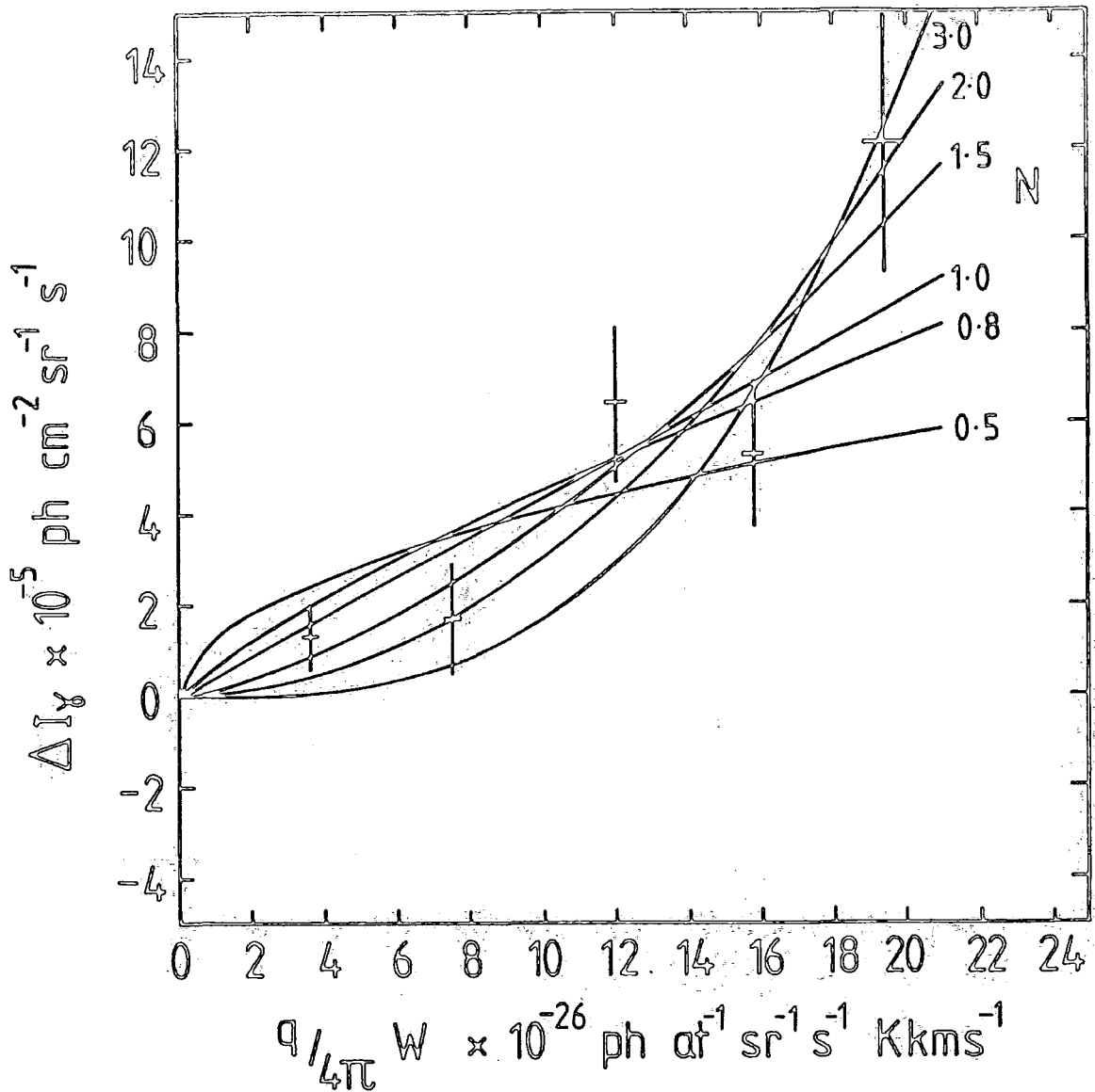
Figure 6.11 Variation of the excess intensity \Delta I_{\gamma} ( > 100 MeV) as a function of q/4\pi[W_{\text{co}}]^N , for the Orion clouds. A reduced fixed isotropic background intensity is assumed. The binned observations are plotted with standard errors. Smooth curves give the expected gamma-ray intensity for each case of N .
