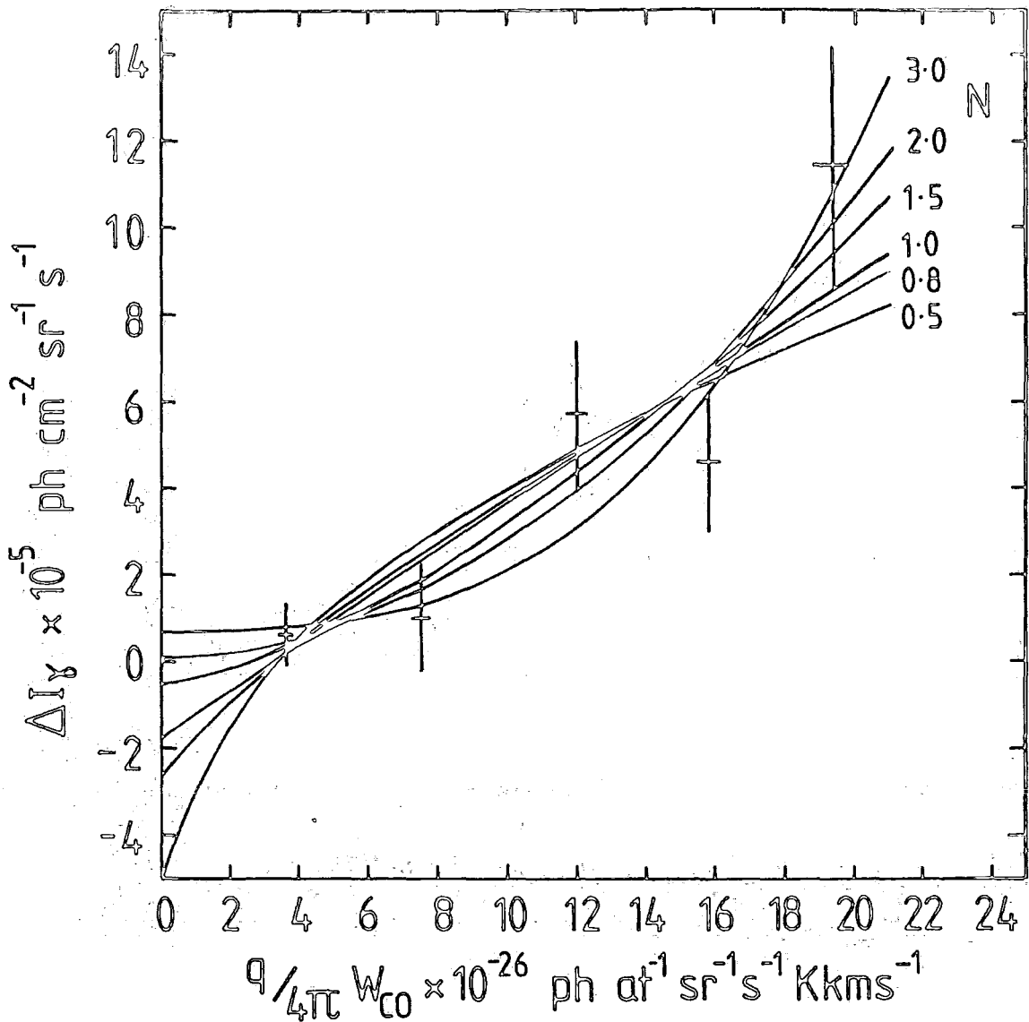
Figure 6.9. Variation of the excess intensity \Delta I_\gamma ( >100 MeV) as a function of \Phi/4\pi [W_{\text{CO}}]^N , for the Orion clouds. The isotropic background intensity I_b is treated as a variable. The binned observations are plotted with standard errors. Smooth curves give the expected gamma-ray intensity for each case of N .
