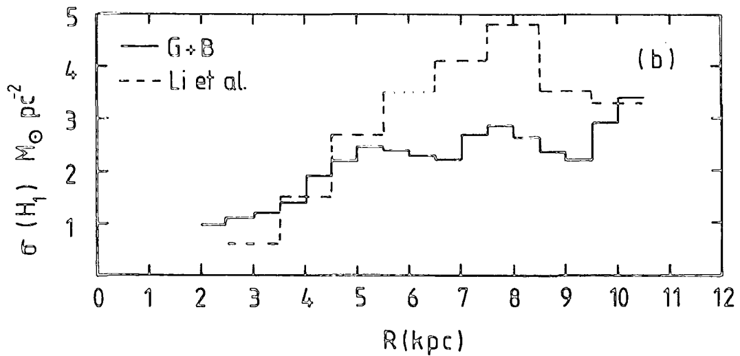
Figure 8.2 (a) The surface densities of H_2 derived from the ^{12}CO surveys by Sanders, Solomon and Scoville (1984a): SSS and Dame (1984). Both are corrected to \alpha = 3.7 \times 10^{20} at \text{cm}^{-2} (\text{K kms}^{-1})^{-1} as described in the text. (b) The surface densities of HI from the data of Gordon and Burton (1976): G + B and Li et al. (1983).
