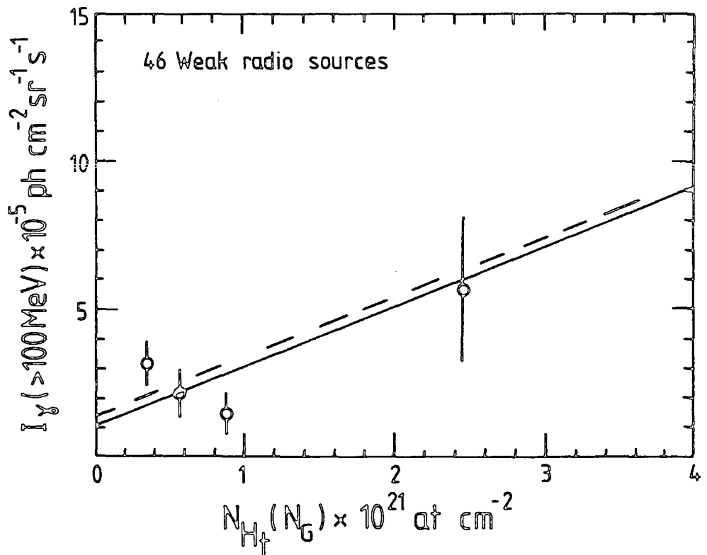
FIGURE 7.3 SAS II Intensities I_\gamma(>100 \text{ MeV})(\pm 1\sigma) versus N_{H_t}(N_G) for the radio source positions. The solid lines are the fits to the mean backgrounds. The excess intensities are given by the broken lines.
