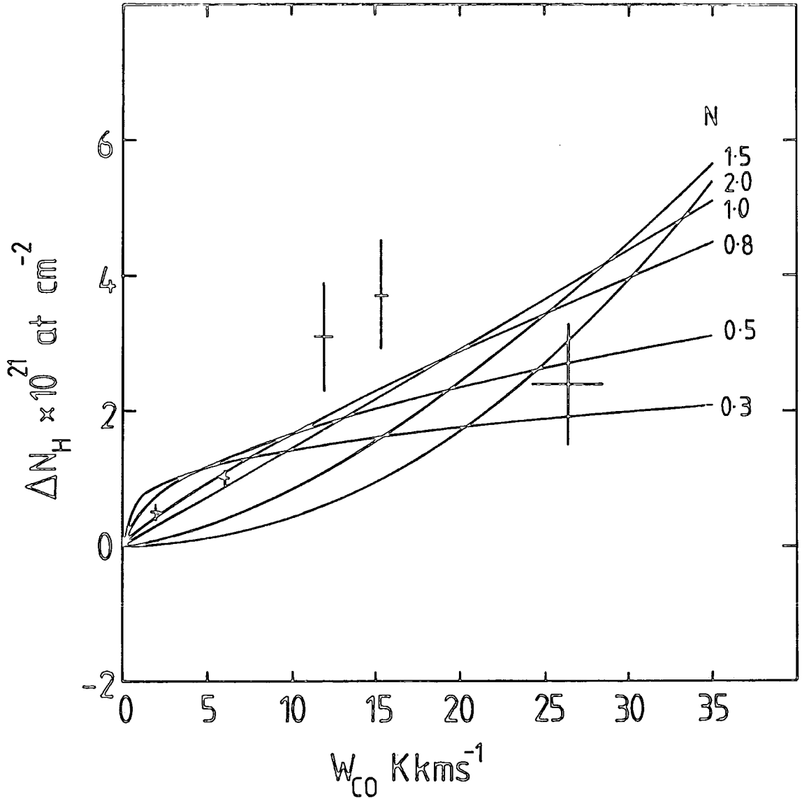
Figure 6.13. Variation of the excess gas column density \Delta N_{\text{H}} = N_{\text{H}_t} (N_{\text{G}}) - N_{\text{HI}} as a function of W_{\text{CO}} for the Orion clouds. The binned observations are plotted with standard errors. Smooth curves give the expected excess column density for each case of N .
