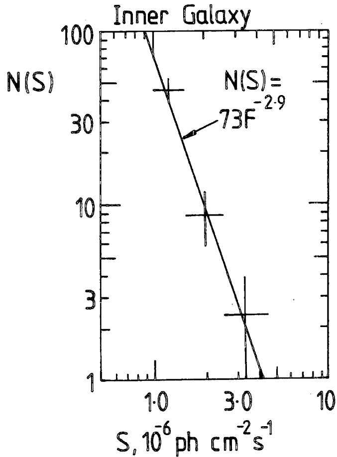
Figure 5.8 Log N - Log S distributions derived from the total 2CG source list ( |b| < 10^\circ ) after applying the appropriate correction factors from Figures 5.5, 5.6, 5.7. Error bars are \pm 1\sigma and the least-squares power law regressions are given in each case.
