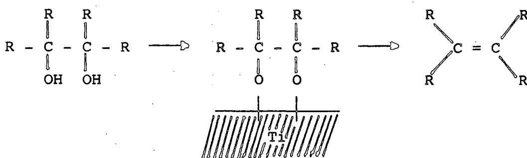
Scheme 3.2
