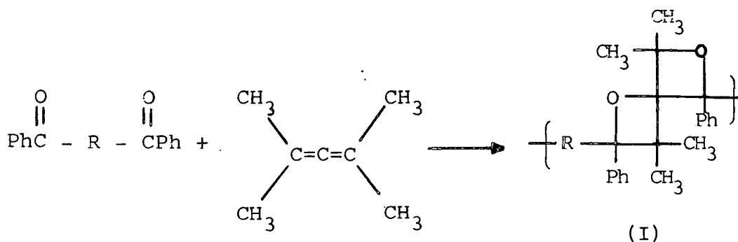
Tetramethylallene
