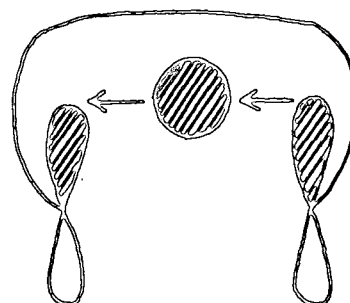
suprafacial migration
