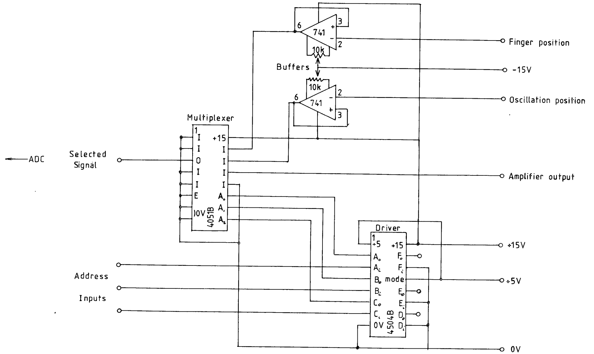
Multiplexer circuitry
