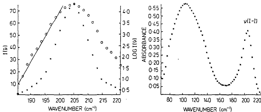
Fig. 5. Spectrum of \nu(\text{I}-\text{I}) band for a solution of I 2 in a cyclohexane/dioxan mixture, T = 300 \text{ K} ; conc. \approx 0.2 \text{ M} .
