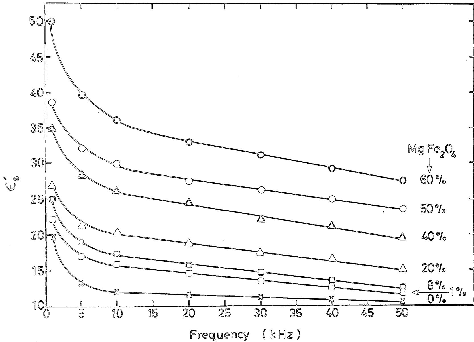
Figure 6.10. Frequency dependence of permittivity in mixed \text{MgFe}_2\text{O}_4 / \text{MgO} powders.
